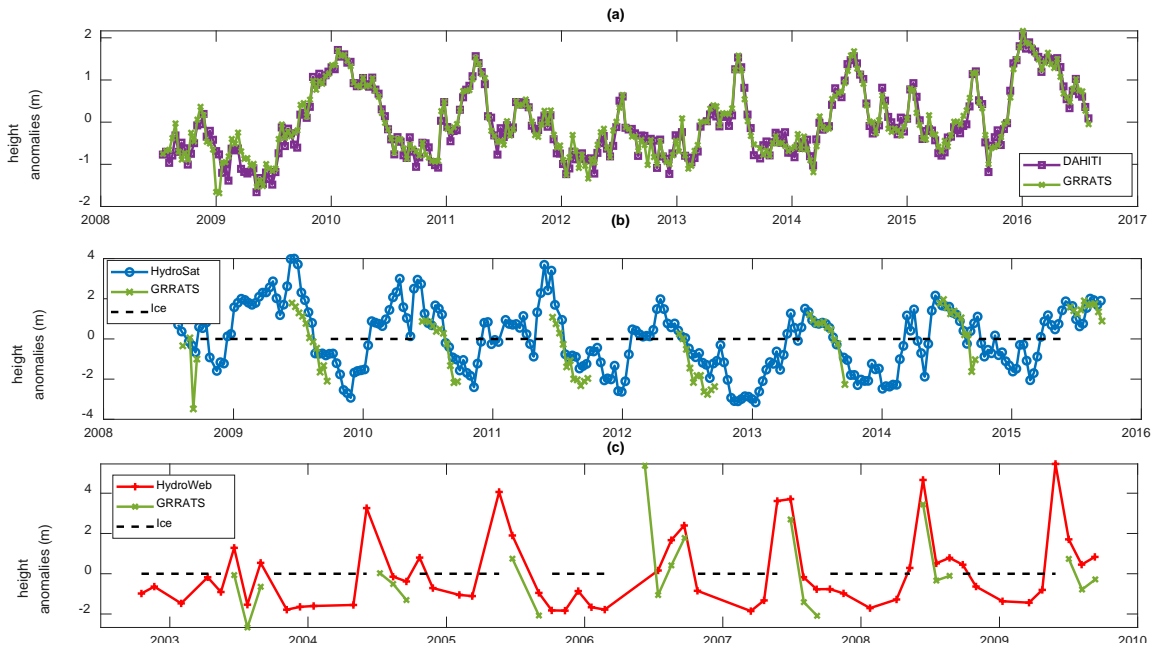
5 Figure 5 multi product evaluation at ungagged river locations GRRATS plotted in green, DAHITI in purple with square markers, HydroSat in blue with circle markers, HydroWeb in red with cross markers, and times of ice cover plotted with a dotted black line. Panel (a) is a comparison with DAHITI on the Parana River. Panel (b) is a comparison with HydroSat on the Ob River, and Panel (c) is a comparison with HydroWeb on the Lena River.
