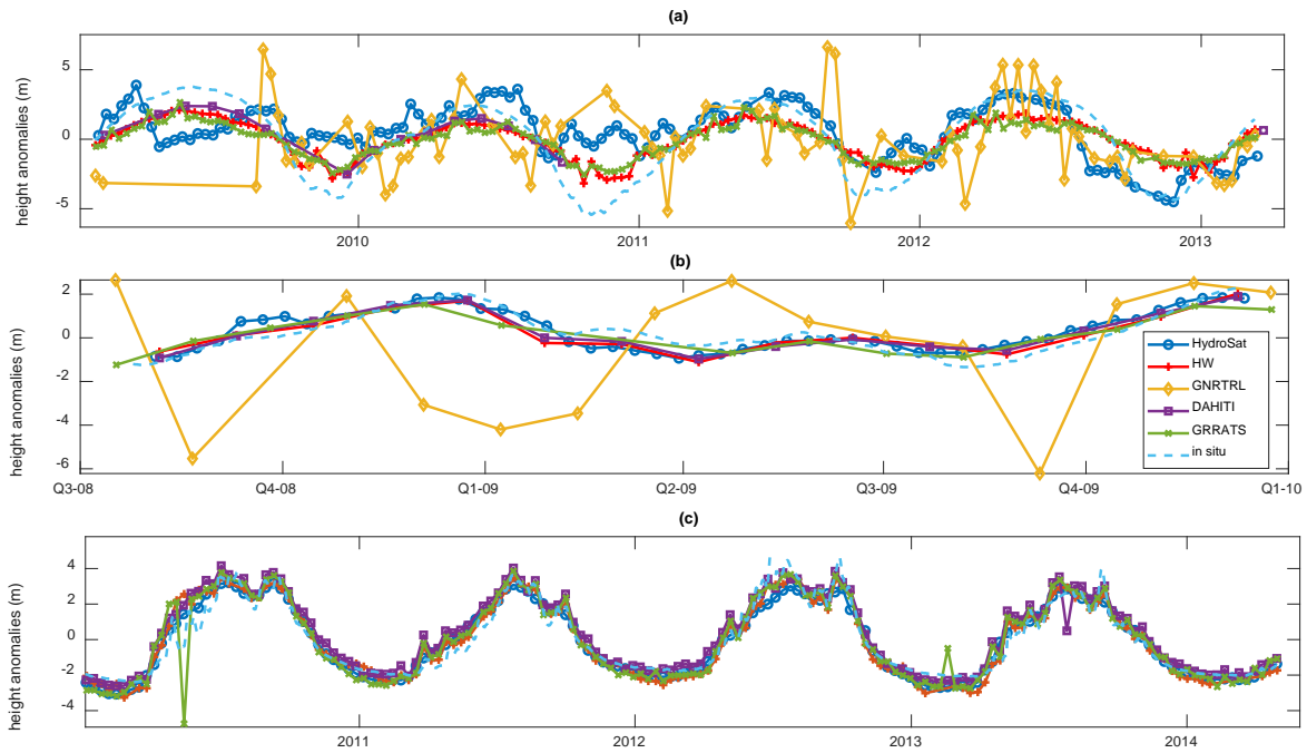
5 Figure 4: Multi product evaluation at same location. Panel (a): multiproduct comparison on the Amazon River Panel (b): multi product comparison on the Congo River. Panel (c): multi product comparison on Brahmaputra River. DAHITI plotted in purple with square markers, HydroSat in dark blue with circle markers, River&LakeNRT in yellow with diamond markers, Hydroweb in red with cross markers, and GRRATS in green with x markers and in-situ in dashed light blue. Note that the legend in panel (b) applies to all of figure 4. GRRATS error bars not shown to improve readability.
