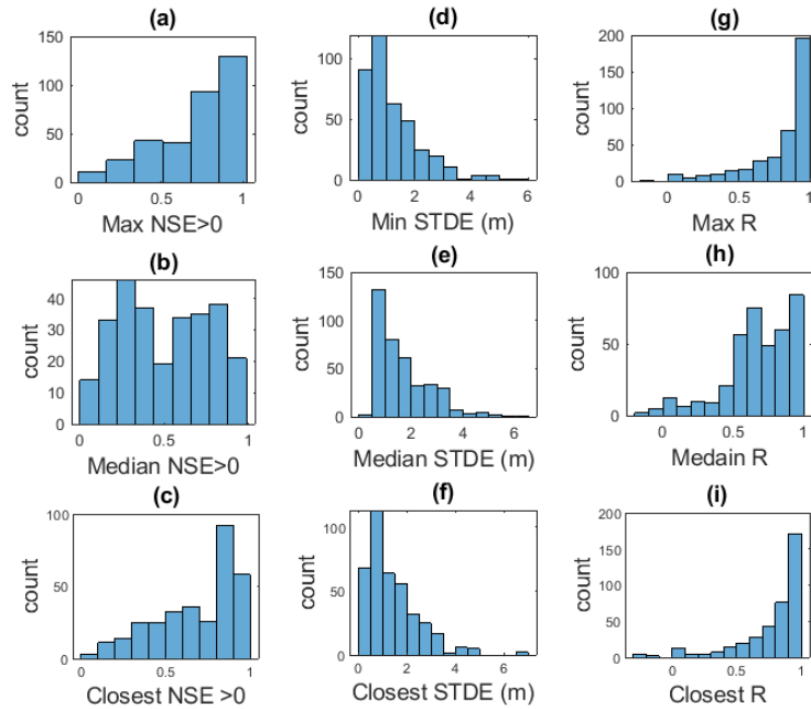
5 Figure 3 Virtual Station fit statistics computed with all available evaluation gages located in the same river and closest comparison. Please note that NSE values are plotted here only when greater than 0 to enable readers to more easily see the majority of the data. 12.2%, 28.8% and 17.2% of the total data are not shown in panel a, b, and c respectively. Panel (a) histogram of the max NSE >0 at each VS in the dataset, Panel (b) histogram of the median NSE > 0 at each VS in the dataset, Panel (c) histogram of closest NSE > 0 , Panel (d) A histogram of the minimum STDE in the dataset, Panel (e) A histogram of the median STDE all the VSs in the dataset, Panel (f) histogram of closest STDE, Panel (g) histogram of the max R at each VS in the dataset, Panel (h) histogram of the median R at each VS in the dataset, Panel (i) histogram of closest R.
