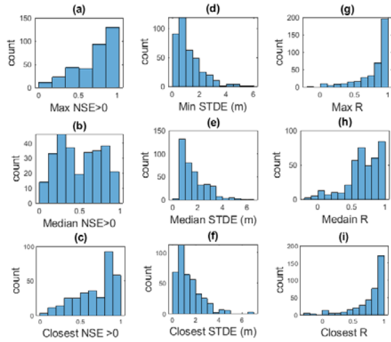
Figure 3 Virtual Station fit statistics computed with all available evaluation gages located in the same river and closest comparison. Please note that NSE values are plotted here only when greater than 0 to enable readers to more easily see the majority of the data. 12.2%, 28.8% and 17.2% of the total data are not shown in panel a, b, and c respectively. Panel (a) histogram of the max NSE >0 at each VS in the dataset, Panel (b) histogram of the median NSE > 0 at each VS in the dataset, Panel (c) histogram of closest NSE > 0, Panel (d) A histogram of the minimum STDE in the dataset, Panel (e) A histogram of the median STDE all the VSs in the dataset, Panel (f) histogram of closest STDE, Panel (g) histogram of the max R at each VS in the dataset, Panel (h) histogram of the median R at each VS in the dataset, Panel (i) histogram of closest R.
