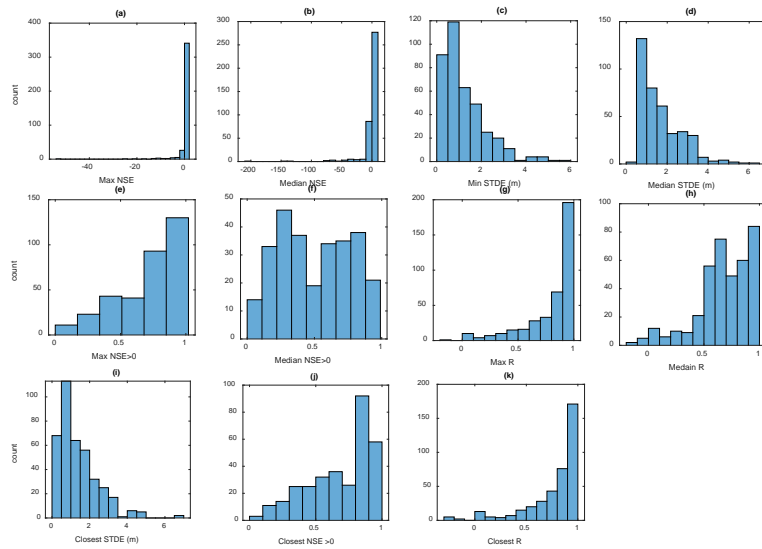
Figure 3 Virtual Stations Nash-Sutcliffe efficiencies computed with all available evaluation gages located in the same river. Panel (a) histogram of the max NSE at each VS in the dataset, Panel (b) histogram of the median NSE at each VS in the dataset, Panel (c) histogram of the minimum STDE at each VS in the dataset, Panel (d) A histogram of the median STDE in the dataset, Panel (e) A histogram of the Max NSE at all the VS s in the dataset with NSE>0, Panel (f) histogram of the median NSE at all the VS s in the dataset with NSE>0, Panel (g) histogram of the max R at each VS in the dataset, Panel (h) histogram of the median R at each VS in the dataset, Panel (i) histogram of closest STDE, Panel (j) histogram of closest NSE>0, Panel (k) histogram of closest R.
