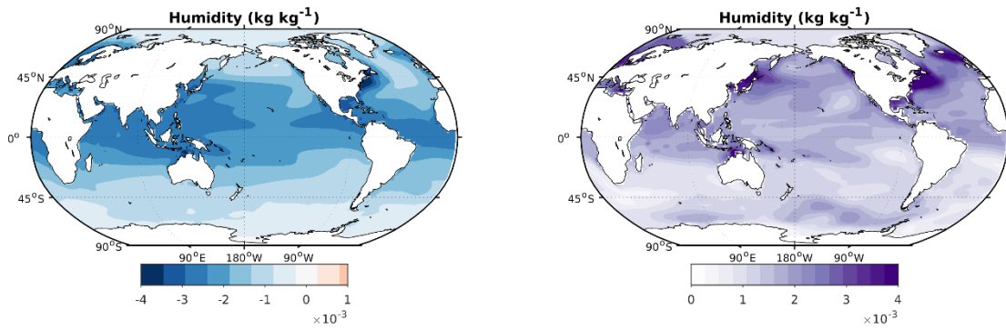
Figure 1: Annual mean specific humidity lgm-piControl anomaly (left) and model spread (right) in \text{kg kg}^{-1} .
