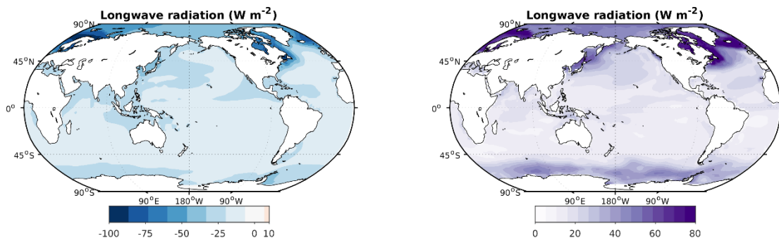
Figure 2: Annual mean downwelling longwave radiation lgm-piControl anomaly (left) and model spread (right) in \text{W m}^{-2} .
