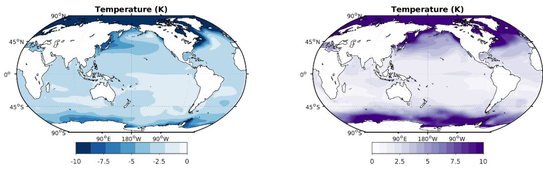
Figure 7: Annual mean temperature Igm-piControl anomaly (left) and model spread (right) in K.
