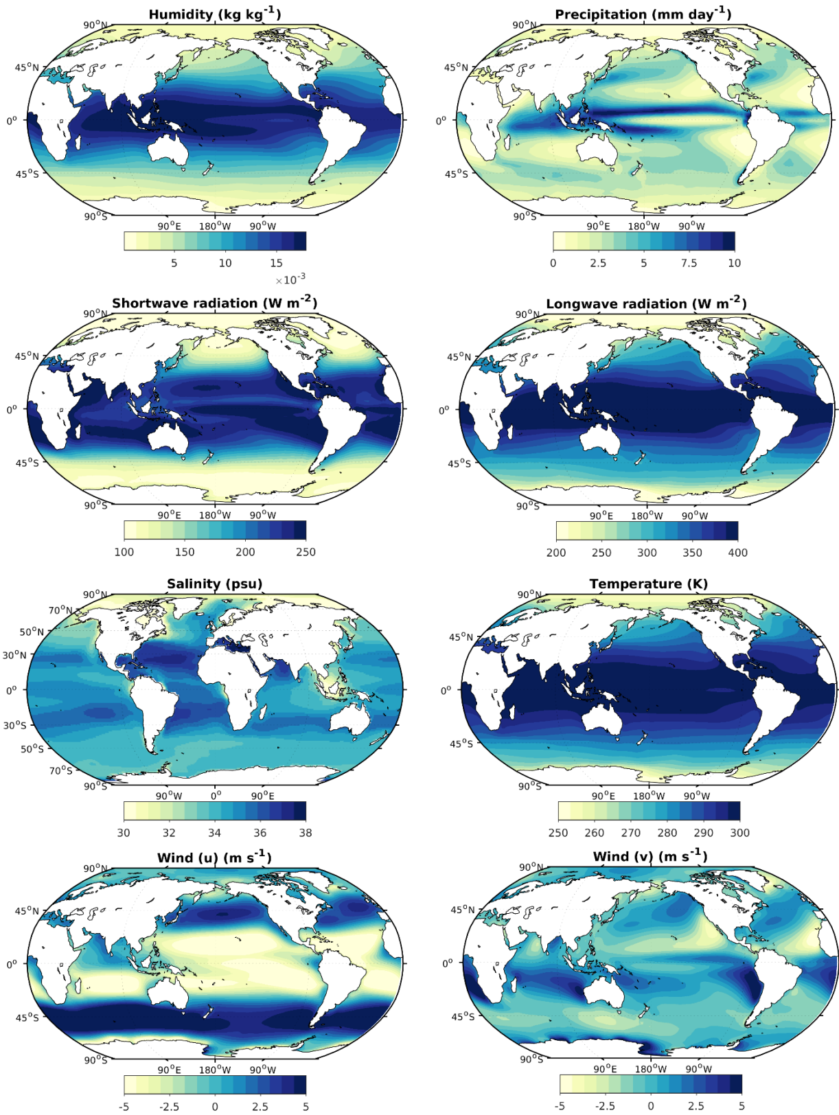
Figure A2: Annual mean for each of the variables (see Table 1) for the piControl CMIP5/PMIP3 experiment.
