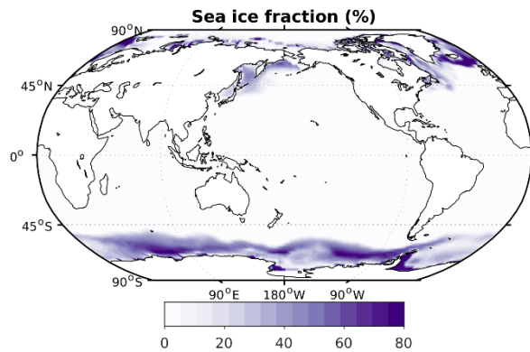
Figure A3: Annual mean model spread of sea ice fraction.
