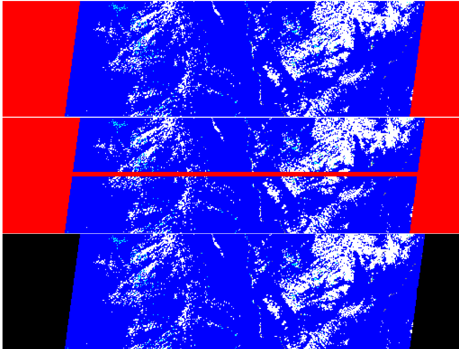
Figure 14. Maps of the RCCM for Path 168, Orbit 92981, Block 101, and camera AF. The linear dimensions of the mapped areas and the color coding are identical to those indicated in Figure 3. Top panel: map of the original RCCM product, which does not contain missing data; middle panel: map of the artificially modified RCCM product, where lines 60 to 64 were declared missing; bottom panel: map of the updated RCCM product, where the inserted missing data have been replaced by estimates.
