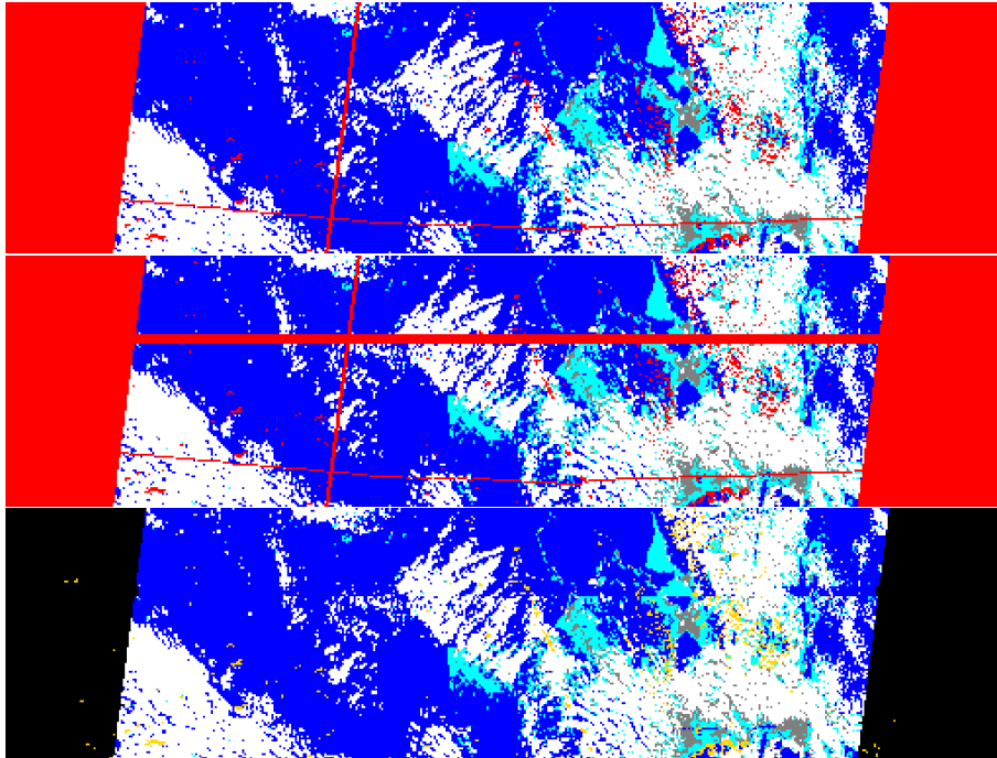
Figure 15. Maps of the RCCM for Path 168, Orbit 92981, Block 102, and camera DA. The linear dimensions of the mapped areas and the color coding are identical to those indicated in Figure 3. Top panel: map of the original RCCM product, which natively contain missing data; middle panel: map of the artificially modified RCCM product, where lines 40 to 44 were declared missing; bottom panel: map of the updated RCCM product, where all missing data have been replaced by estimates.
