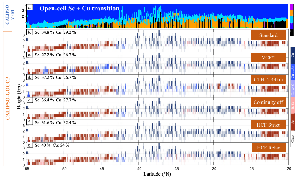
Figure 11: Same as Fig. 5 but for a typical Open-cell Se to Cu transitioning case overlapping the south-east Pacific and the Southern Ocean (~ 55°S to 20°S, 2008-07-14 21:10:19, daytime).
