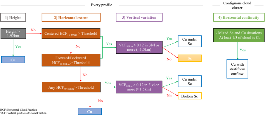
Flow Diagram of the Cu – Sc discrimination
