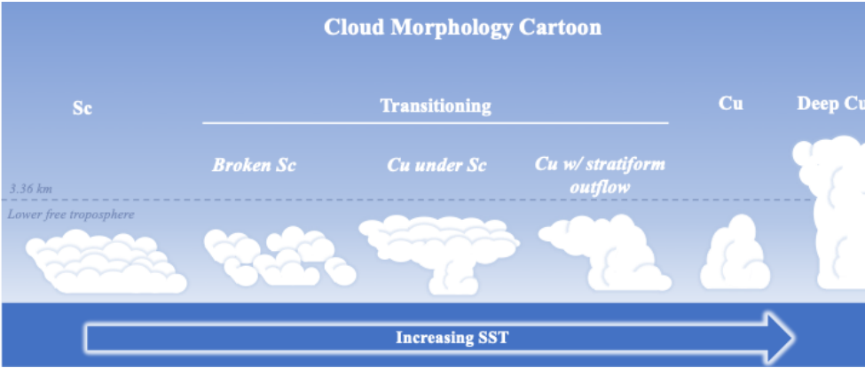
Figure 1: Cartoon representing the different cloud morphologies used in this study. The blue dashed line denotes the upper limit of the low-level clouds following GOCCP definition (3.36 km). Note that the Deep Cu type is not a low cloud, but either a mid- or high-level cloud.
