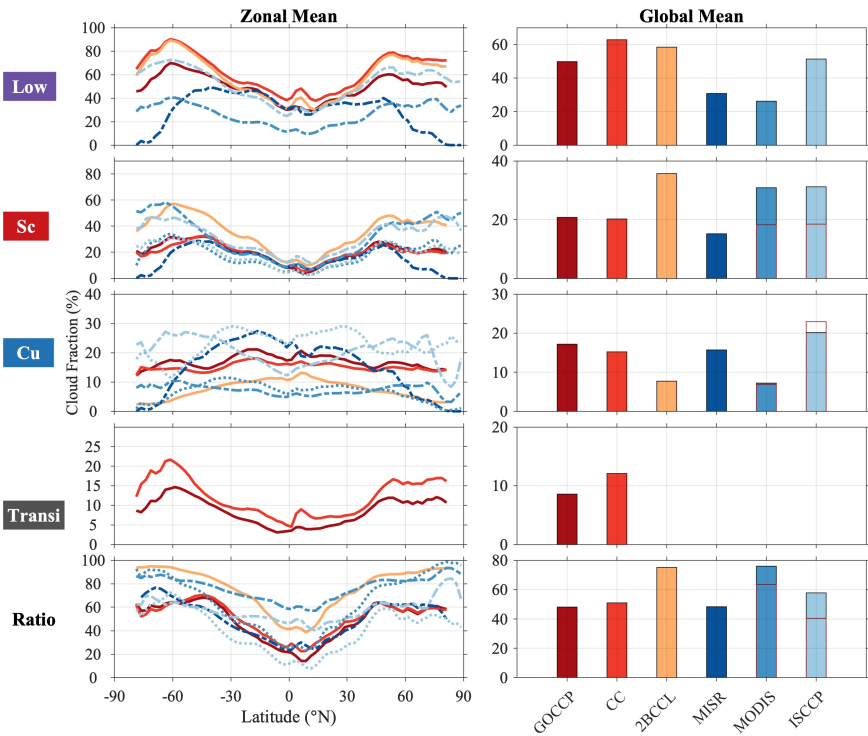
Figure 14: Global zonal mean (% left ) and global area-weighted mean (% right ) of low, Sc, Cu, transitioning (i.e., broken Sc, Cu under Sc and Cu with stratiform outflow) and the ratio Sc to Sc-Cu clouds –from the top to the bottom– for all the satellite datasets using the same time period as in Fig. 13. Active-sensor observations are represented in solid lines as opposed to dashed lines for COT-CTP passive-sensor observations and dotted lines for clustering passive-sensor observations. The clustering area-weighted means are represented by transparent bars with red borders. Note that the y-axis are different in every subplots. All datasets are averaged onto a 2.5°x2.5° grid.
