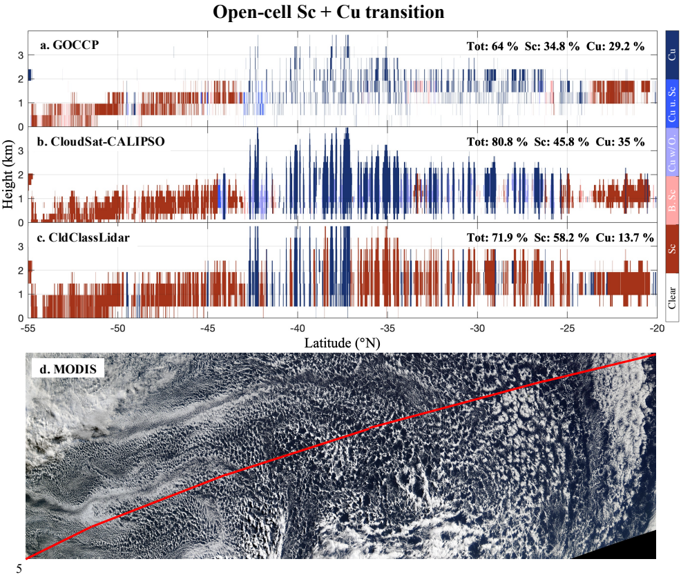
Figure 12: Same as Fig. 6 but for a typical Open-cell Sc to Cu transitioning case overlapping the south-east Pacific and the Southern Ocean (~ 55°S to 20°S, 2008-07-14 21:10:19, daytime).
