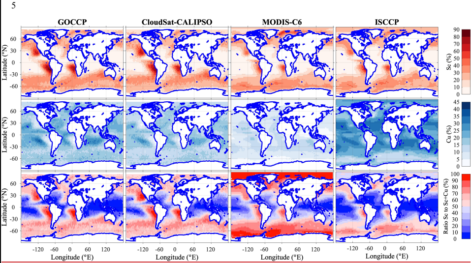
Figure 15: Similar to Fig. 13, maps (x axis, longitude [°E]; y axis, latitude [°N]) of (top to bottom) Sc, Cu and the ratio Sc to Sc-and-Cu cloud fraction (%) for (left to right) GOCCP (2007-2016), RL-GeoProf (2007-2010), MODIS Terra and Aqua Cloud Regime (2003-2015) and ISCCP Weather State (2001-2008).
