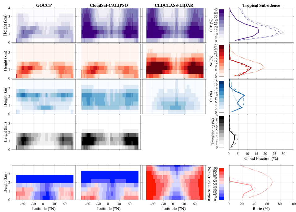
Figure 16: Zonal profiles (x axis, latitude [°N]; y axis, height [km]) of low (first row), Sc (second row), Cu (third row) and transitioning (i.e., broken Sc, Cu under Sc and Cu with stratiform outflow; fourth row) cloud fraction (%) for GOCCP (first column), RL-GeoProf (second column) and 2BCCL (third column). As in Fig. 13, different color bars are used to better separate each type of cloud. The corresponding profiles for tropical subsidence regimes ( \omega_{500} > 10 hPa/day between 35°S/N following Cesana et al., 2019a) are represented in the fourth column for GOCCP (solid line), RL-GeoProf (dashed line) and 2BCCL (dotted line). Note that extratropical profiles are shown in Fig. S10.
