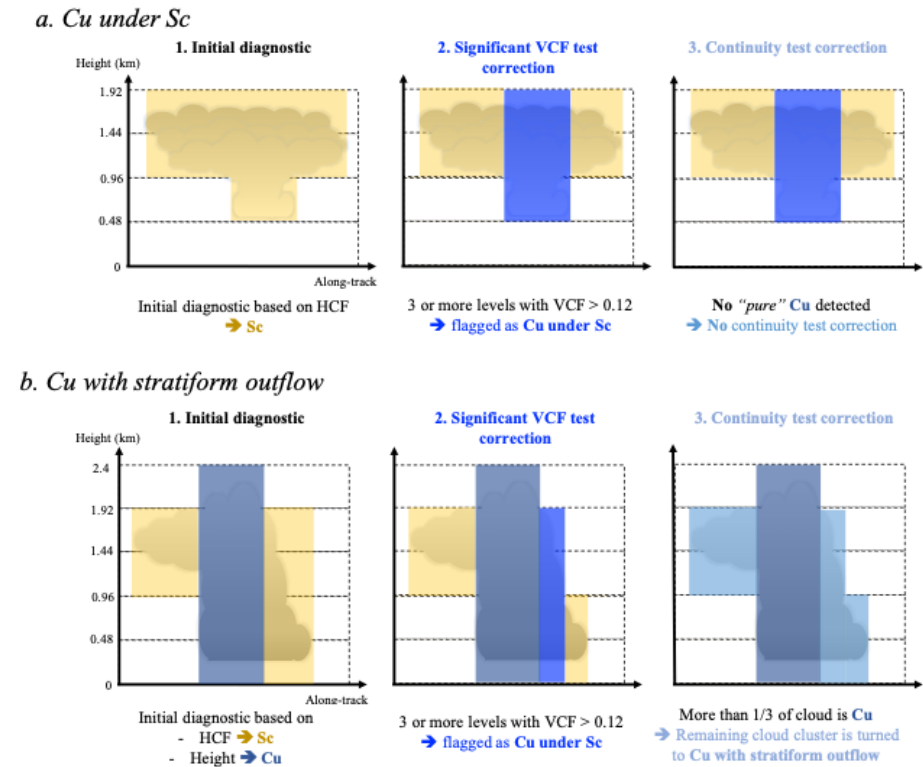
Figure 5: Cartoon of the Cu and Sc mixed situations using additional diagnostics in the DA: a) Cu under Sc and b) Cu with stratiform outflow . After the DA diagnoses (1) an initial cloud type, the additional (2) “significant VCF variability” test and (3) “horizontal continuity” correction are applied to contiguous cloud clusters (See details in section 3.4 and 3.5).
