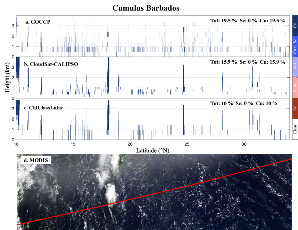
Figure 10: Same as Fig. 8 but for another cumulus case overpassing the Barbados (~ 10°N to 35°N, 2008-07-09 17:34:08 daytime)
