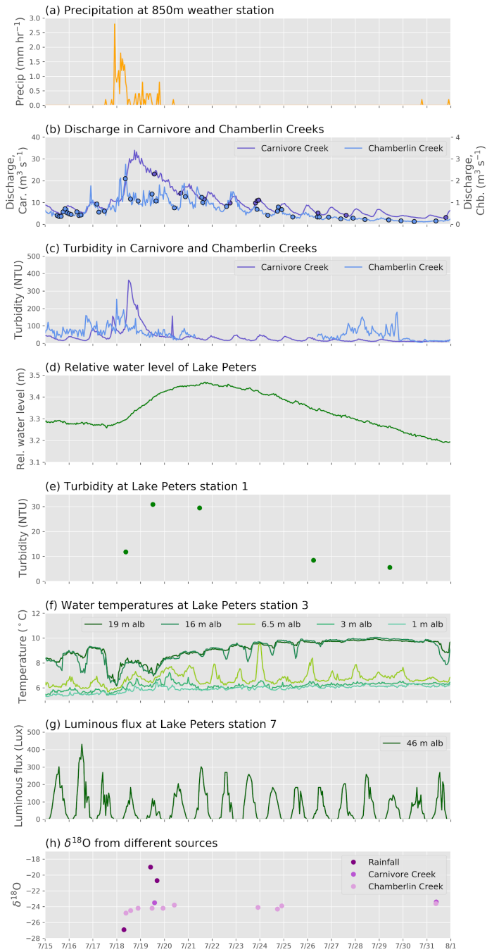
Figure 10. An example of a complementary dataset from Lake Peters observatory, tracing the effects of a precipitation event in July 2015. (a) Rainfall at the 850 m a.s.l. station; (b) Carnivore and Chamberlin Creek discharge and (c) turbidity; (d) Lake Peters relative water level, (e) maximum turbidity at Lake Peters Station 1, (f) water temperatures at different heights above lake bottom (a.l.b.) at Lake Peters Station 3, and (g) luminous flux at Lake Peters Station 7; and (h) \delta^{18}\text{O} at different sites. To complement panel (e), a more detailed sample of turbidity data are shown in Fig. 11.
