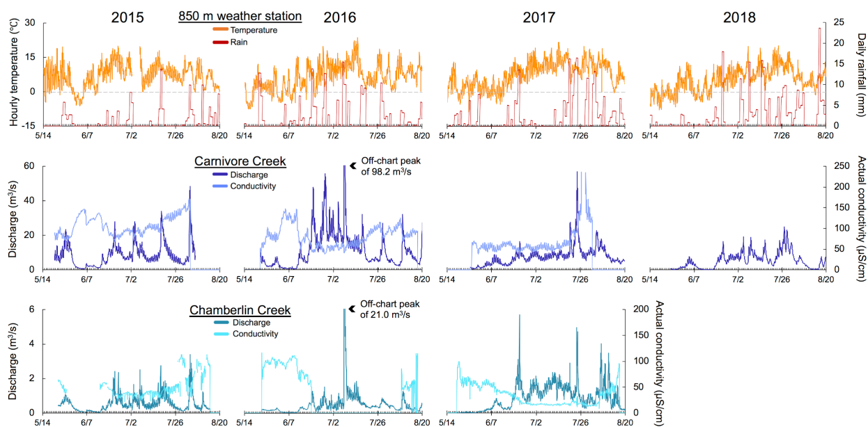
Figure 8. Time series of hourly air temperature and rainfall from the 850 m a.s.l. weather station at Lake Peters shown alongside conductivity and discharge for Carnivore and Chamberlin Creeks, 2015-2018. The gray line in the top row indicates 0°C.
