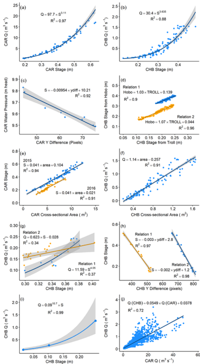
570 Figure 7. Regression relations and associated confidence bands used to create continuous discharge (Q) time series throughout the 2015-2018 open-channel seasons in Carnivore (CAR) and Chamberlin (CHB) Creeks. (a) discharge – stage (S) relation for CAR (2015); (b) discharge – stage relation for CHB (2015); (c) water-pressure (from TROLL) – vertical difference (y-diff; shown on photographs) relation for CAR (2015); (d) relations of stage calculated from Hobo U20 water pressure against stage calculated from TROLL 9500 water pressure for CHB (both 2015); (e) stage – cross-sectional area linear relation for CAR (2015 and 2016); 575 (f) discharge – cross-sectional area linear relation for CHB (2015); (g) discharge – stage (from Hobo) power relation for CHB (2016); (h) Stage – vertical difference (y-diff; shown on photographs) linear relations for CHB (both 2016); (i) discharge – stage exponential relation for CHB (2016); and (j) Relation of discharge in CHB against discharge in CAR with a 2-hour lag (2015 and 2016). Refer to Thurston (2017) for additional information.
