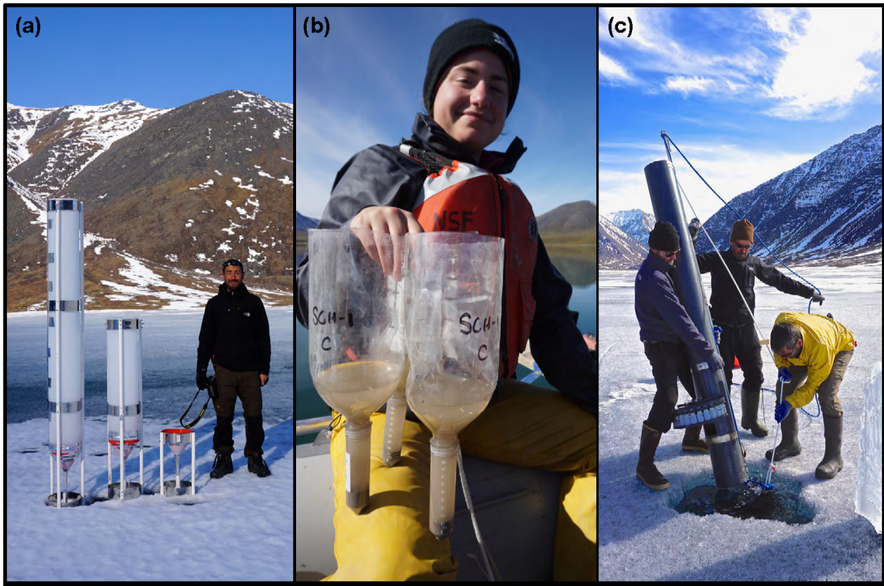
Figure 9. Examples of the types of sediment traps installed in Lake Peters: (a) static traps used to investigate the effect of collection-tube aspect ratio, (b) 2L-bottle static traps upon retrieval, and (c) installation of an incrementing trap.
