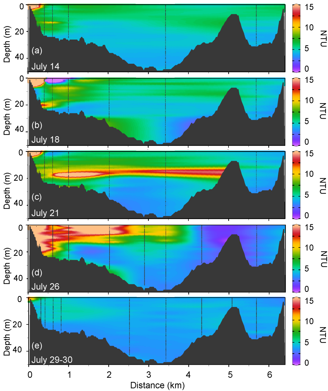
Figure 11. Turbidity in Lake Peters over the course of a precipitation event in July 2015; turbidity data are shown for (a) July 14, (b) July 18, (c) July 21, (d) July 26, and (e) composite data from July 29 and July 30. Black shading indicates lake bathymetry, and black dashed lines indicate locations of TROLL casts. The x-axis indicates north-south distance across the lake from the outflow of Carnivore Creek. Figure created using Ocean Data View (ODV) software.
