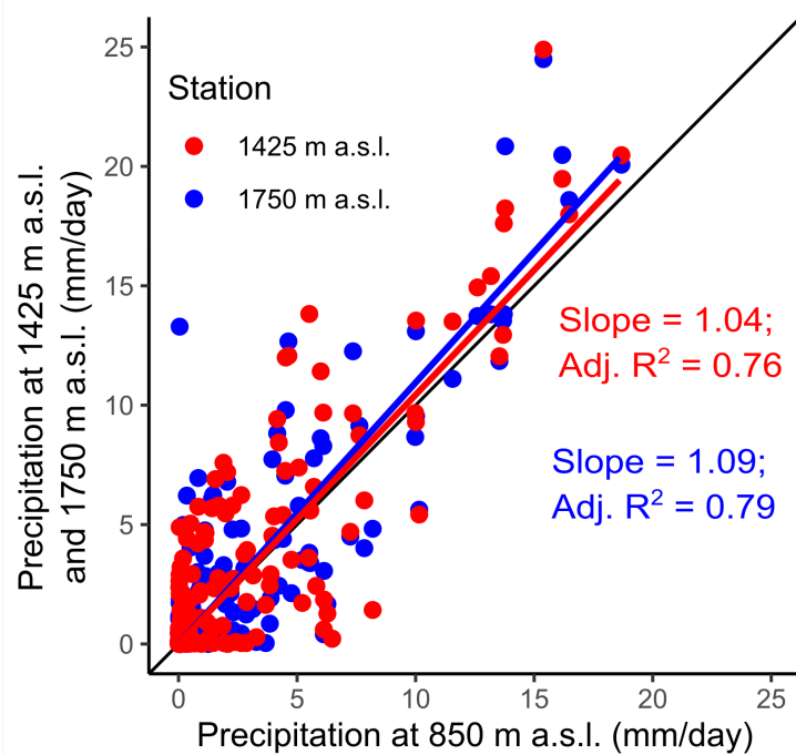
Figure 4. Correlations between daily precipitation at 1425 m a.s.l. (red) and 1750 m a.s.l. (blue) with daily precipitation at 850 m a.s.l. Lines are least-squares regressions. Also shown in black is the 1:1 line.
