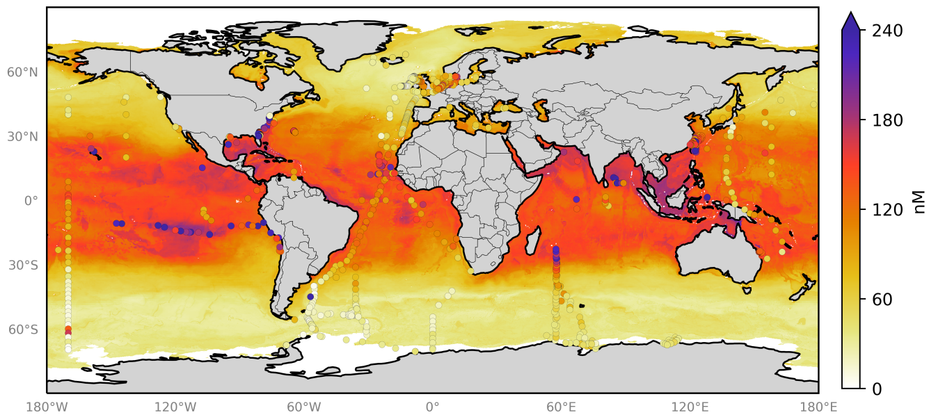
Figure 6. Annual average predicted sea-surface iodide by the 10-member ensemble of models (“RFR(Ensemble)”), overlaid with iodide observations from Chance et al. (2019a) without outliers. Outliers are defined here as values greater than 3rd quartile plus 1.5 times the interquartile range (Frigge et al., 1989). Only locations that are entirely water are included in the spatial average.
