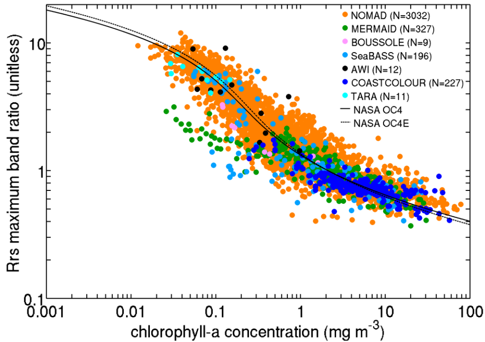
Figure 11. A remote-sensing reflectance maximum band ratio (as defined in text) ([443,490,510]/555 or [443,490,510]/560 if 555 not available) as a function of chlorophyll-a concentration. All chlorophyll data were considered, but for a given station, HPLC data were selected if available. Data within 2 nm of the wavelengths were used. For reference, the solid and dotted lines show the NASA OC4 and OC4E v6 standard algorithms, respectively ( http://oceancolor.gsfc.nasa.gov/cms/atbd/chlor_a ). The total number of points was 3,814, of which 79% were from NOMAD.
