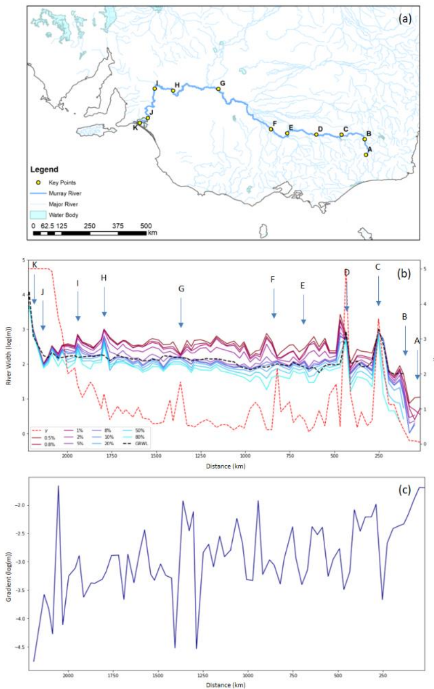
Figure 8. Longitudinal profile of the Murray River showing (a) location of river and selected locations; (b) profile of width at different frequencies and river morphology parameter \gamma , and (c) profile of river gradient. Values are averaged for 30 km sections along the river channel. Letters indicate: (A) source according to our data; (B) source according to GRWL data (Allen and Pavelsky, 2018); (C) Lake Hume; (D) Yarrowonga Weir; (E) and (F) anabranching locations; (G) Mildura; (H–I) Lower Murray wetlands; (J–K) Lake Alexandrina.
