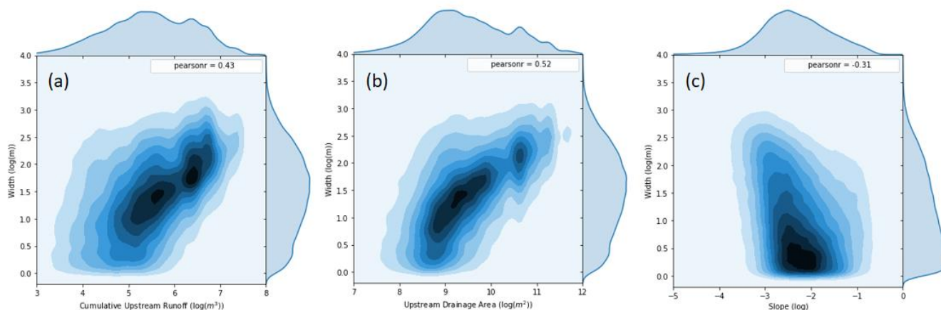
5 Figure 4 The relationships between maximum river width and cumulative upstream runoff (a), upstream drainage area (b) and river gradient (c) (The color coding is related to data counts with highest in dark blue, lowest in light blue, which is corresponding to the histogram on the axes).
