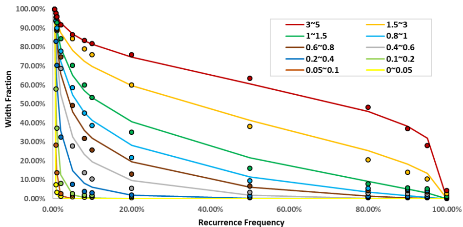
Figure 7 Curves characteristics for different river morphology categories (line: prediction; dot: observation).
