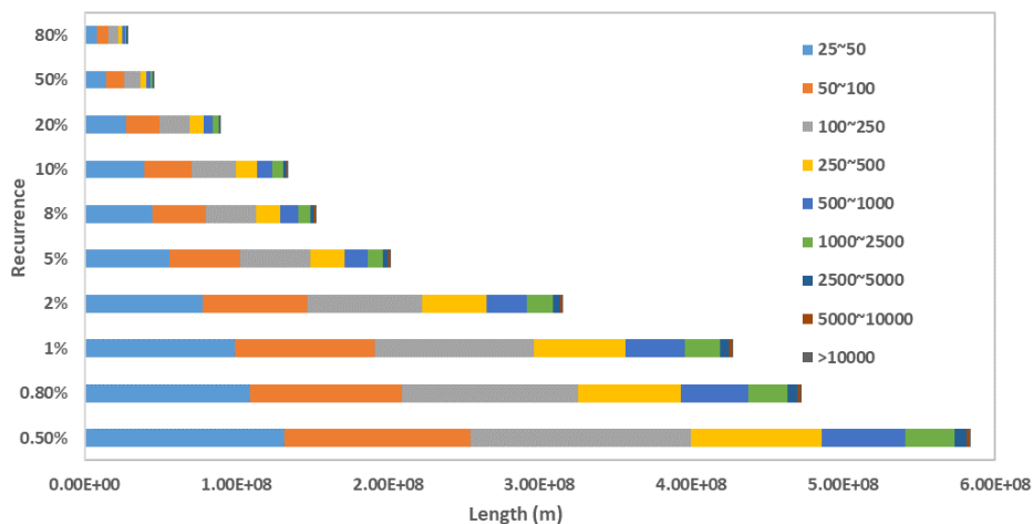
Figure 3 The total lengths in different width ranges at different recurrence frequencies for Australia.
