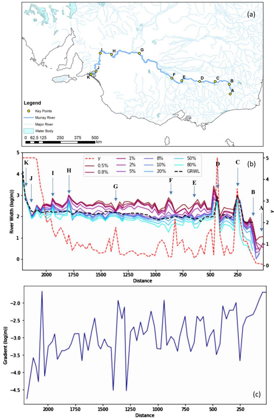
Figure 11. Longitudinal profile of the Murray River showing (a) location of river and selected locations; (b) profile of width at different frequencies and river morphology parameter \gamma , and (c) profile of river gradient. Values are averaged for 30 km sections along the river channel. Letters indicate: (A) source according to our data; (B) source according to GRWL data (Allen and Pavelsky, 2018); (C) Lake Hume; (D) Yarrowonga Weir; (E) and (F) anabranching locations; (G) Mildura; (H–I) Lower Murray wetlands; (J–K) Lake Alexandrina.
