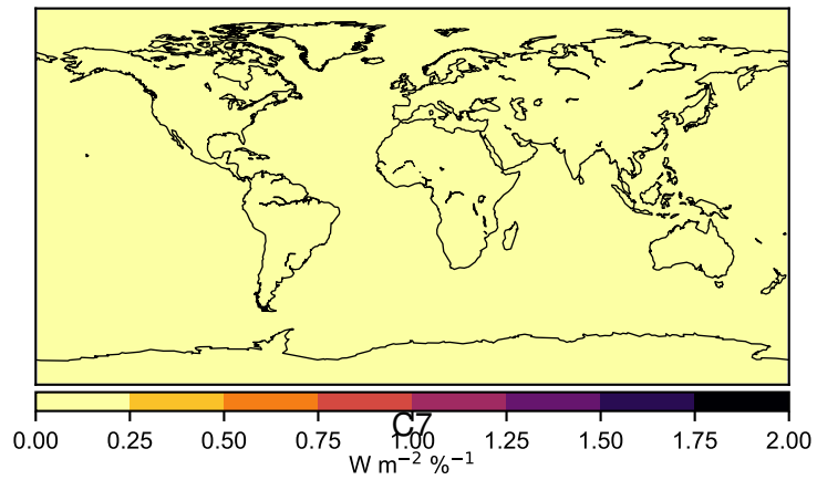
(2e - 2f) All-sky minus clear-sky surface surface temperature kernel
