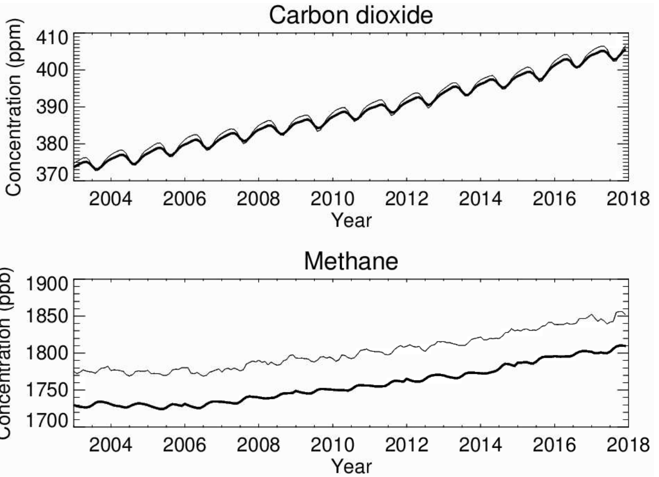
Figure 2: Time series of globally and monthly averaged concentrations of (top) carbon dioxide, in ppm, and (bottom) methane, in ppb, over the period 2003-2017. Bold lines show mass-weighted total column averages for the CAMS Greenhouse Flux Inversion products. Thin lines show background surface measurements from NOAA's Earth System Research Laboratory for carbon dioxide and the Advanced Global Atmospheric Gases Experiment for methane, respectively.
