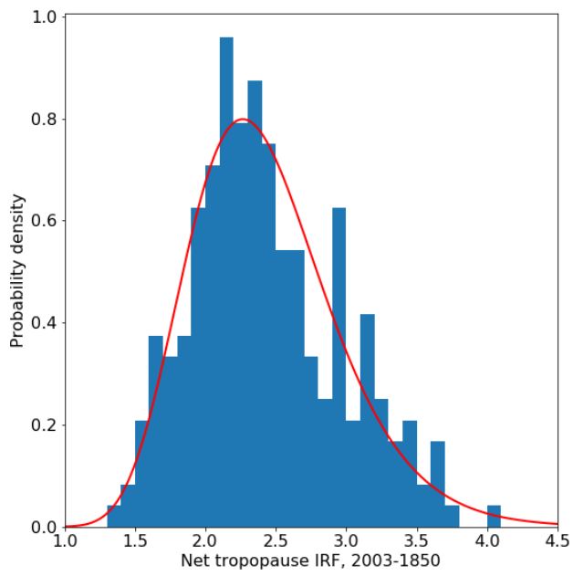
1110 Figure 9: Probability density function for the global annual mean instantaneous radiative forcing ( \text{W m}^{-2} ) for the year 2003, resulting from the CAMS Climate Forcing Perturbed Parameter Ensemble. A lognormal fit to the distribution is shown in red.
