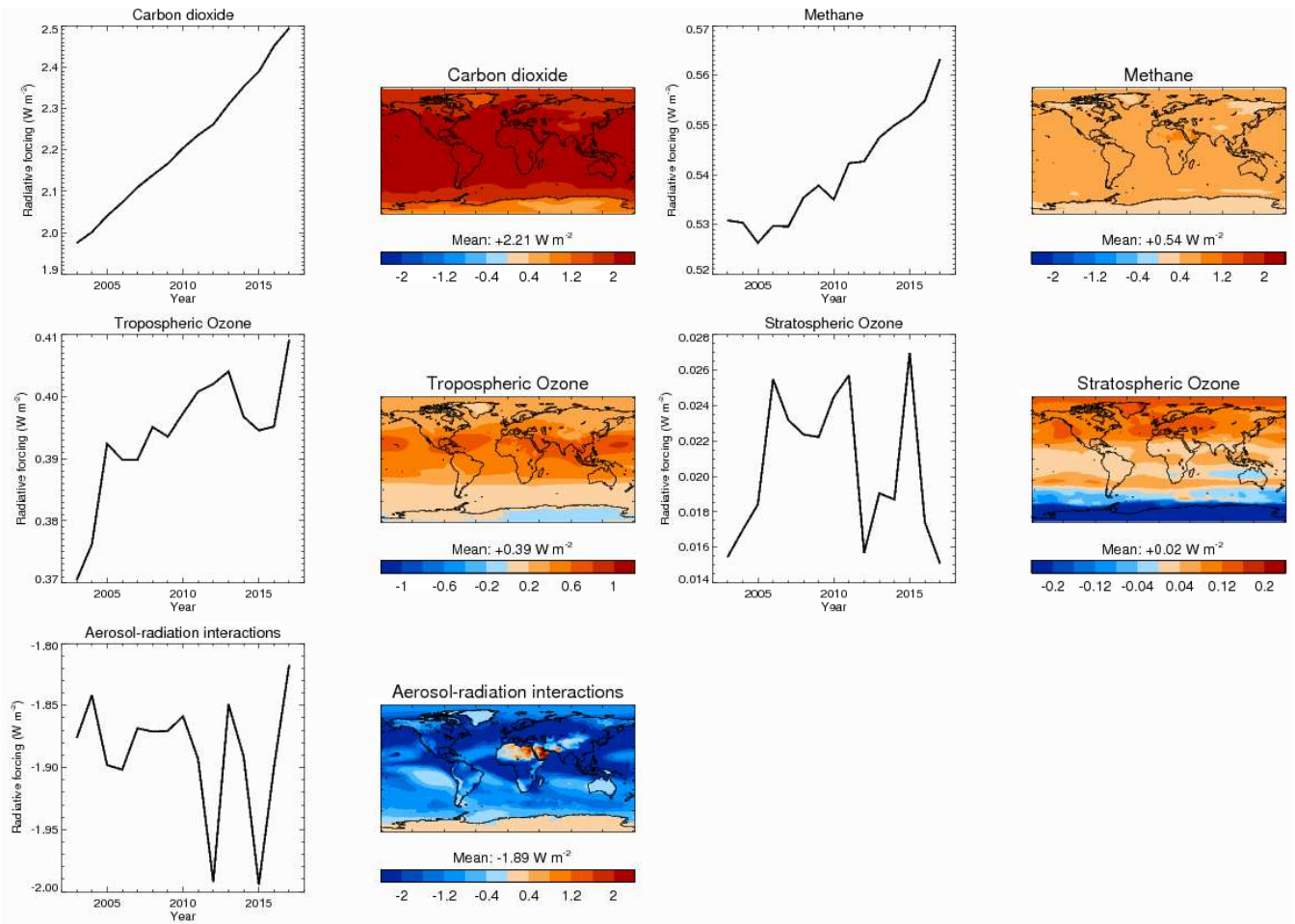
1120 Figure 11: As Figure 10, but for cloud-free conditions. Note that radiative forcing of aerosol-cloud interactions is undefined in the absence of clouds, so is not shown here.
