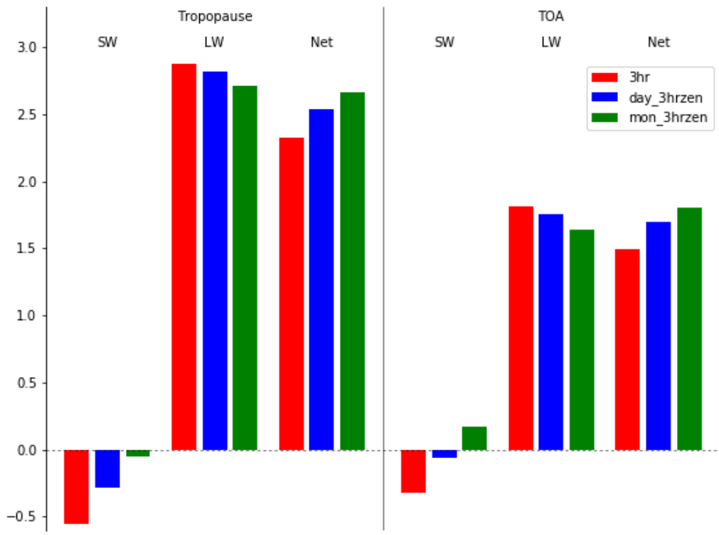
1105 Figure 8: Year 2003 global-mean instantaneous radiative forcing, in W m^{-2} , at the tropopause and top of atmosphere for 3-hourly solar zenith angle timesteps for 3-hourly, daily and monthly climatologies.
