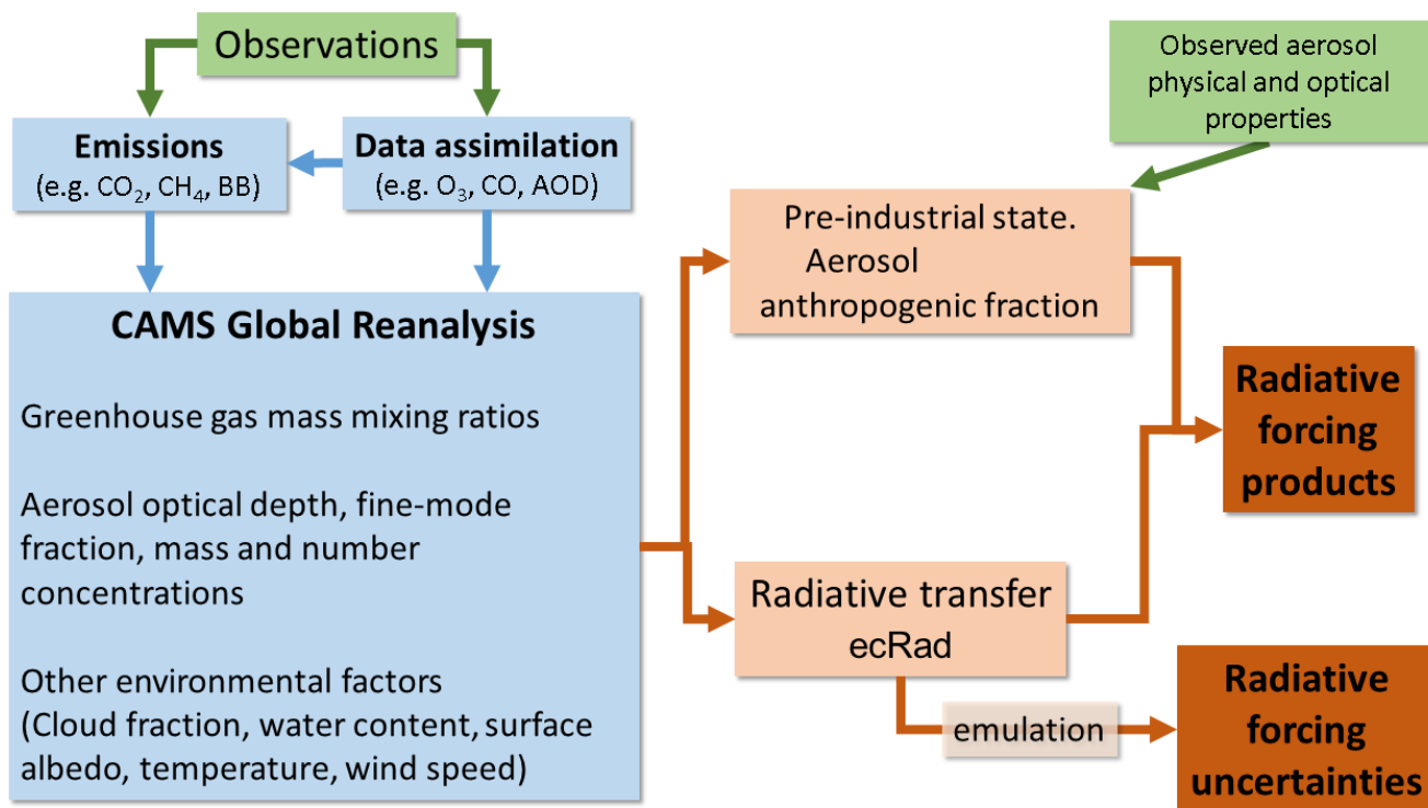
1070 Figure 1: Diagram of the radiative forcing production chain (light orange), which takes inputs from the CAMS Global Reanalysis (blue) and produces radiative forcing estimates and their uncertainties (dark orange). Green boxes indicate observational constraints. BB stands for biomass burning and AOD for aerosol optical depth. ecRad is the radiative transfer code used by the ECMWF IFS.
