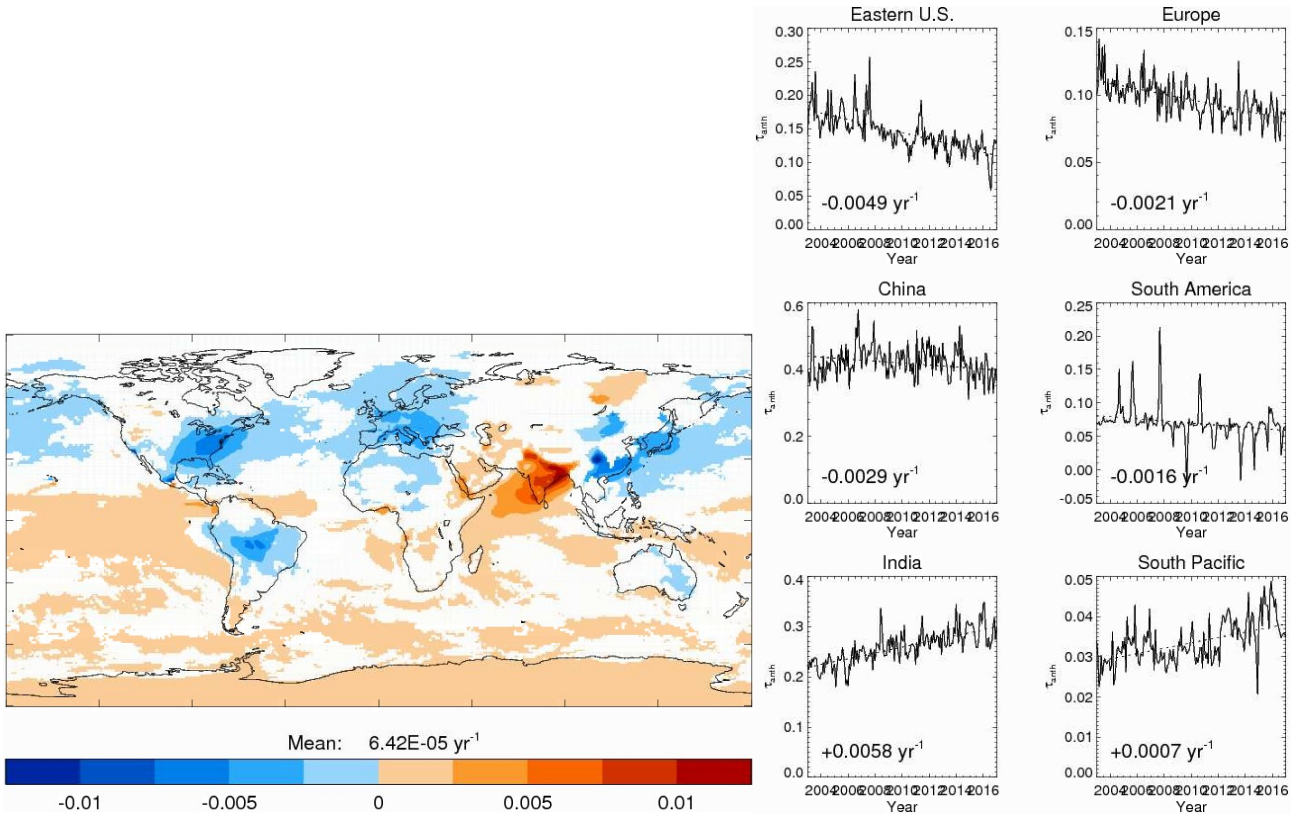
Figure 15: Linear trends, in \text{yr}^{-1} , in anthropogenic aerosol optical depth at 0.55 \mu\text{m} over the period 2003-2017 according to the CAMS Climate Forcing aerosol origin identification algorithm. Regions where trends are statistically insignificant are masked in white. Right-hand side plots show time series of anthropogenic aerosol optical depth, \tau_{anth} , (solid lines) and their linear fits (dashed lines) in selected regions.
