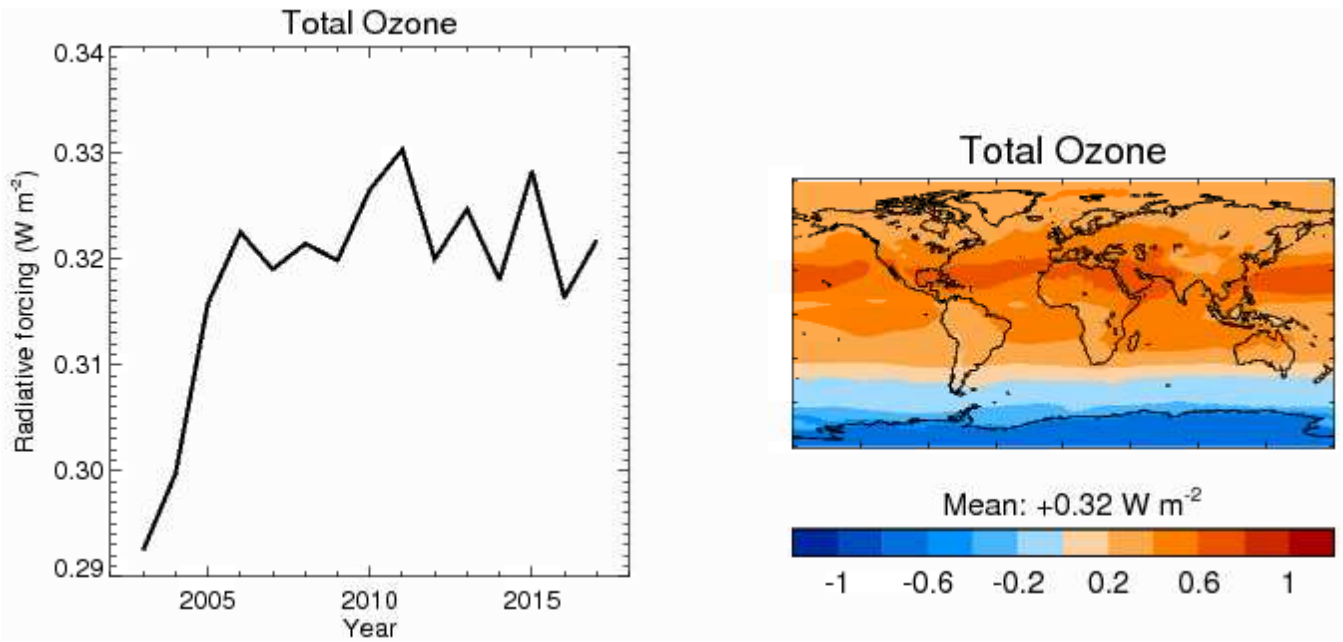
Figure 14: Annual and global-mean time series and average distribution for the CAMS Reanalysis period 2003–2017 of the stratospherically adjusted radiative forcing, relative to 1750 and in \text{W m}^{-2} , of ozone, calculated as the sum of tropospheric and stratospheric ozone radiative forcing. Radiative forcing is given for shortwave plus longwave.
