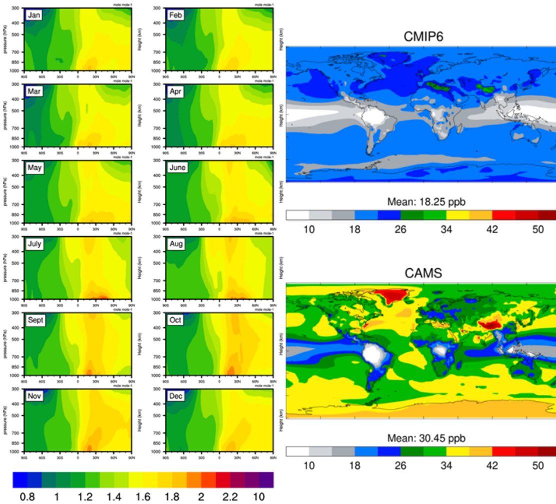
Figure 6: Left: Monthly-averaged zonal cross-sections of ratios of present-day (2008–2014) to preindustrial (1850–1900) ozone mass-mixing ratios from the CMIP6 inputs4MIPs climatology. Right: Surface ozone volume mixing ratios, in ppb, in (top) the CMIP6 inputs4MIPs climatology, and (bottom) scaled from the CAMS Reanalysis using the ratios shown on the left.
