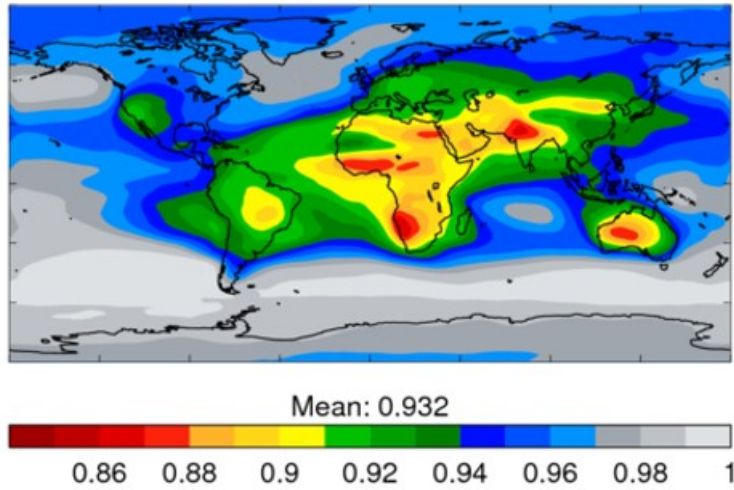
Figure 5: Annually averaged distribution of column-averaged single-scattering albedo at 0.55 μm used to characterize absorption of anthropogenic aerosols.
