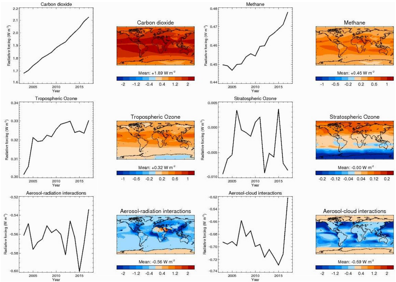
1115 Figure 10: Annual and global-mean time series and average distribution for the CAMS Reanalysis period 2003–2017 of the stratospherically adjusted radiative forcing, relative to 1750 and in W m^{-2} , of carbon dioxide, methane, tropospheric ozone, stratospheric ozone, aerosol-radiation interactions, and aerosol-cloud interactions. Radiative forcing is given for shortwave plus longwave, except for aerosols where it is given for shortwave only.
