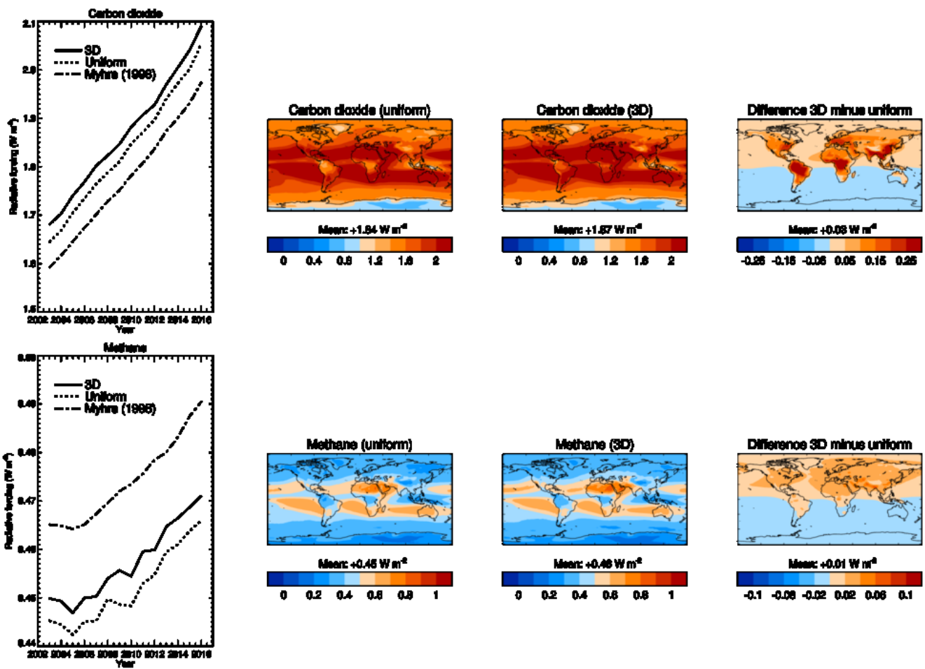
Figure 13: Comparison of stratospherically adjusted radiative forcing, in W m^{-2} , of carbon dioxide (top) and methane (bottom) based on either the three-dimensional distributions produced by CAMS Greenhouse Gas Flux or the surface measurements of the NOAA Earth System Research Laboratory for carbon dioxide and the Advanced Global Atmospheric Gases Experiment for methane. Corresponding concentrations time series are shown in Figure 2. Left panels show time series for 2003-2016, with radiative forcing from three-dimensional distributions shown as the solid line, from uniform concentrations as the dashed line, and from the simplified expressions of Myhre et al. (1998) as the dot-dashed line. Maps show, from left to right, the distributions from three-dimensional distributions, from uniform concentrations, and their difference.
