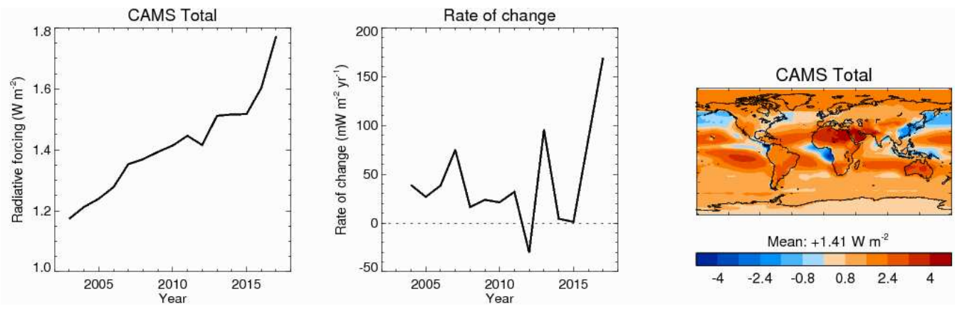
1125 Figure 12: (Left) Time series of globally, annually averaged total stratospherically adjusted radiative forcing, in the shortwave and longwave spectra and in \text{W m}^{-2} , for the period 2003-2017. Total radiative forcing is here defined as the sum of the radiative forcing components shown in Figure 10. (Middle) Rate of change in total radiative forcing, calculated as the change in total radiative forcing from one year to the next and given in \text{mW m}^{-2} \text{yr}^{-1} . (Right) Distribution of total stratospherically adjusted radiative forcing, averaged over the period 2003-2017, in \text{W m}^{-2} .
