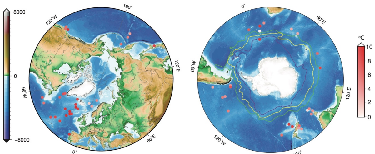
Figure 7: Mid- to high-latitude sea surface temperature (SST) difference between late Marine Isotope Stage 6 and maximum values of the early Last Interglacial (Stage 5). Map made using Generic Mapping Tools (GMT) (Wessel et al., 2013).
