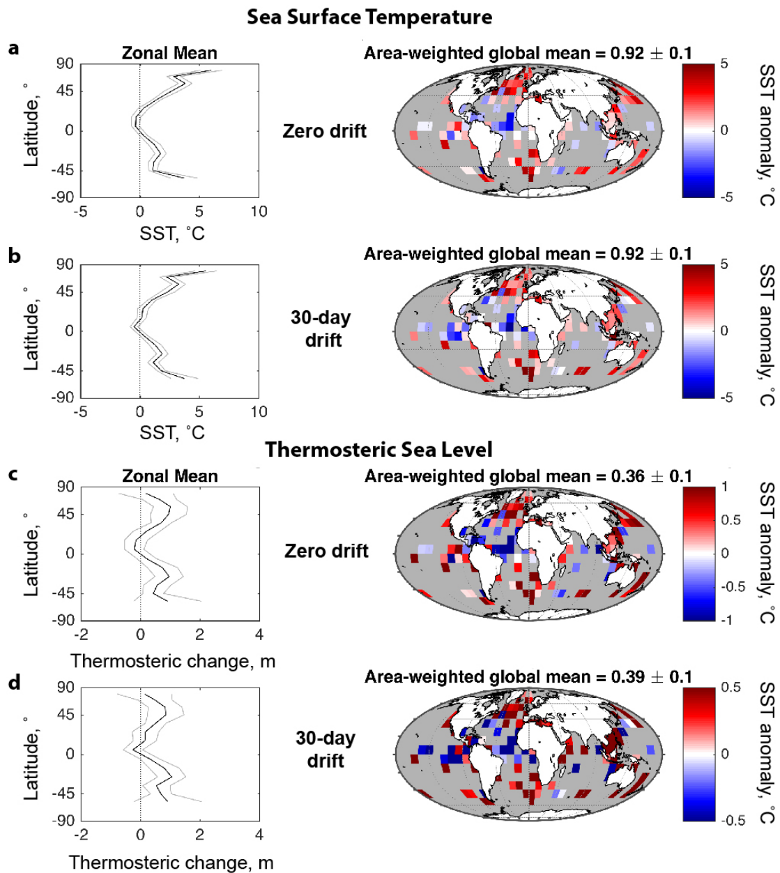
Figure 6: Global and zonal mean annual sea-surface temperature (SST) anomalies and thermosteric sea level change during the early Last Interglacial. Temperature anomalies reported as uncorrected (panels a and c respectively) and after applying 30-day (panels b and d respectively) temperature offsets arising from ocean current drift. Uncertainty for zonal average reconstructions given at 1\sigma . Here ocean warming is assumed to have penetrated to 2000 m depth, on average. Temperature estimates relative to the modern period (CE 1981-2010).
