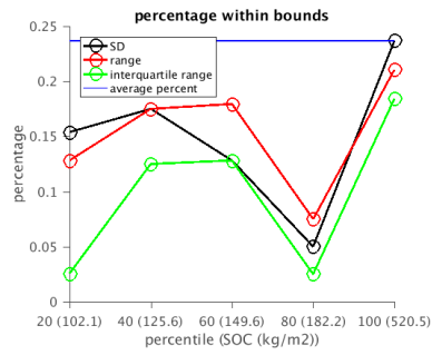
1075 Figure S12: The same as Figure 3 except for using ISCN data and model ensemble of A, C, D, E and F to predict soil carbon storage from 200cm to deep soil.
