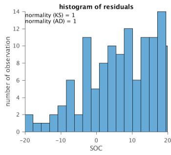
1075 Figure S12: The same as Figure 3 except for using ISCN data and model ensemble of A, C, D, E and F to predict soil carbon storage from 200cm to deep soil.
