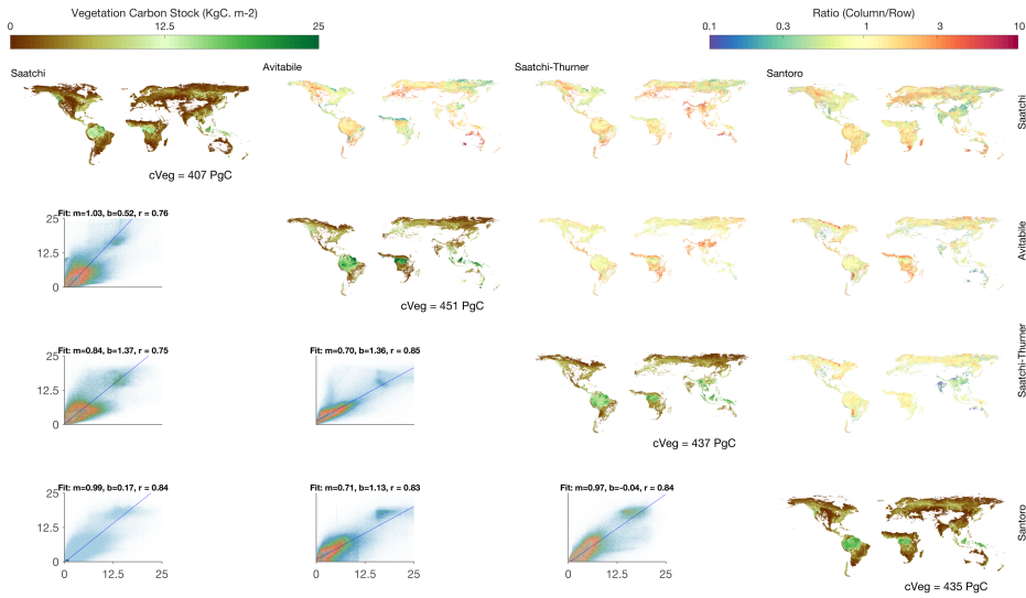
915 Figure 3: The spatial distribution of vegetation carbon stock and relative uncertainty (interquartile range/mean). The total amount of carbon stock of vegetation (AGB+BGB+herbaceous) is shown in the bottom of each diagonal subplot. The upper off-diagonal are the ratios between each pair of datasets (column/row). The bottom off-diagonal subplots show the major axis regression between each pair of datasets (m: slope, b: intercept, r: correlation coefficient).
