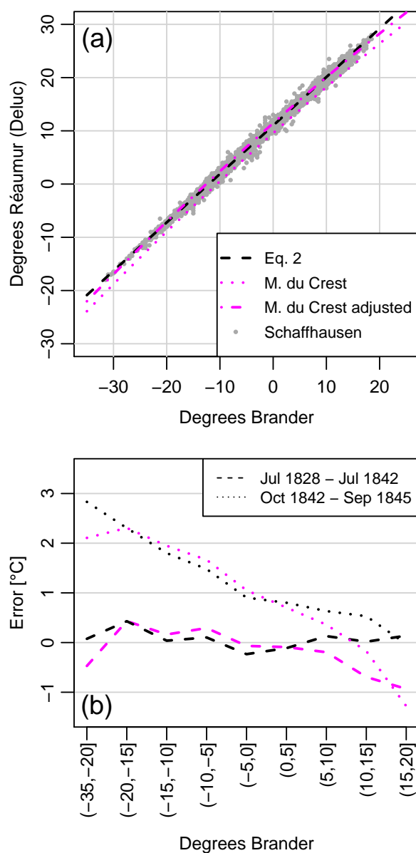
Figure 5. a) Scatter plot of parallel observations in Schaffhausen between a thermometer with Brander scale and one with Réaumur scale, made between 1828–1842; the lines represent different possible conversion functions discussed in the text. b) Median of differences between the parallel observations when using Eq. 2 (black lines) or a bias-adjusted Micheli du Crest scale (purple lines) for conversion, for different intervals of temperature.
