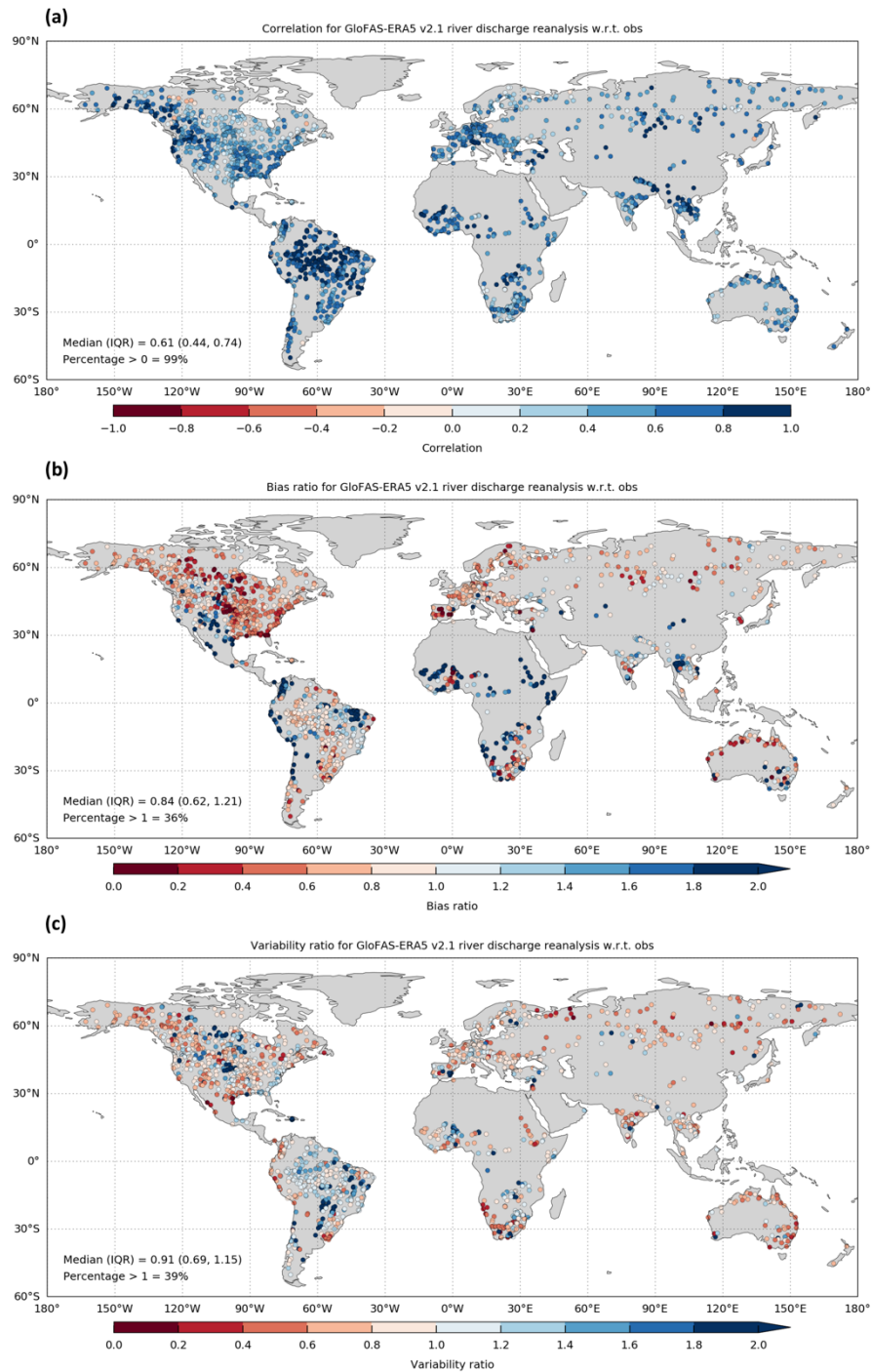
Figure 6: Decomposition of the Modified Kling-Gupta Efficiency KGE' into its three components, Pearson correlation (a), bias ratio (b), and variability ratio (c) for GloFAS-ERA5 river discharge reanalysis against 1801 observation stations. Optimum values for each of the three KGE' components is 1. Blue (red) dots represent positive (negative) values.
