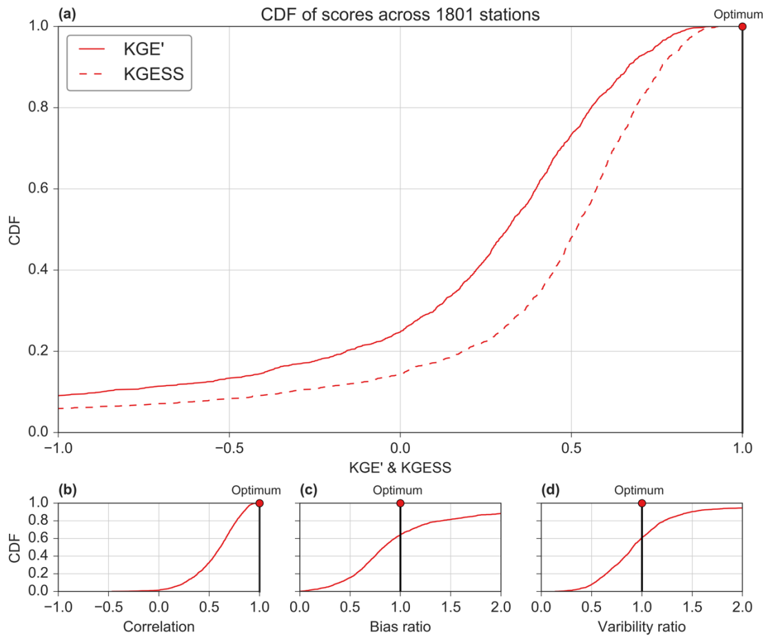
245 Figure 4: Cumulative distribution function of performance metrics across all 1801 stations. Modified Kling-Gupta Efficiency (KGE') and Skill Score (KGESS) (a) with decomposition of KGE' into Pearson correlation (b), bias ratio (c), and variability ratio (d). The red dot marks the optimum value for each metric.
