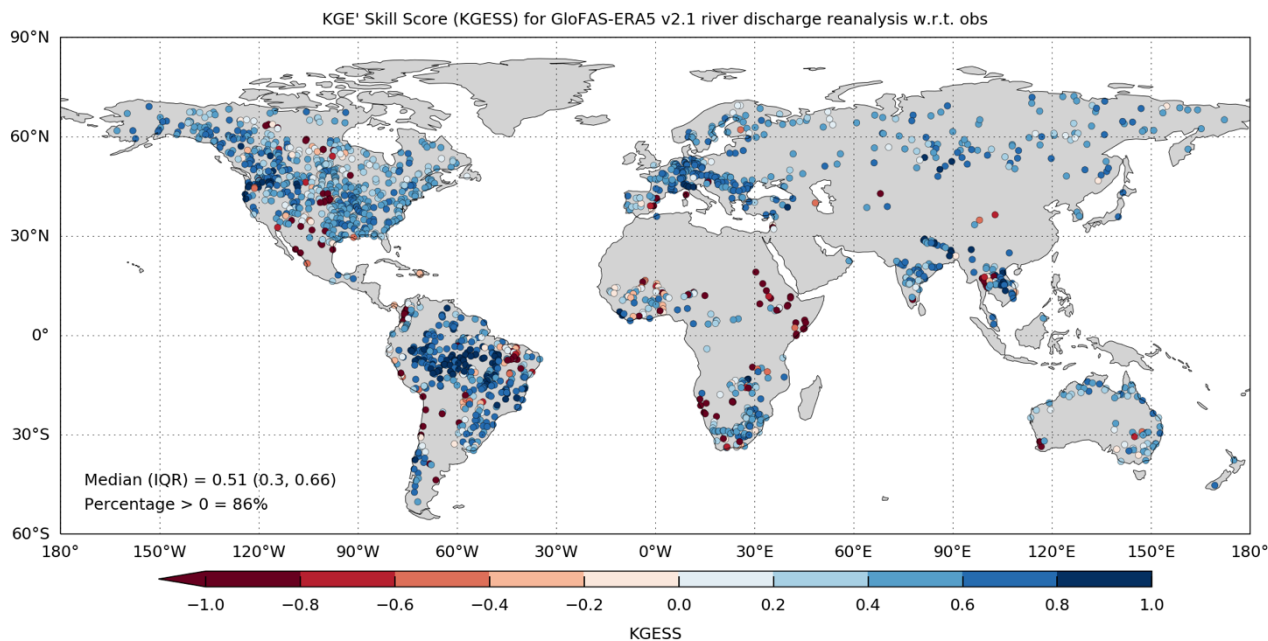
250 Figure 5: Modified Kling-Gupta Efficiency Skill Score (KGESS) for GloFAS-ERA5 river discharge reanalysis against 1801 observation stations. Optimum value of KGESS is 1. Blue (red) dots show catchments with positive (negative) skill.
