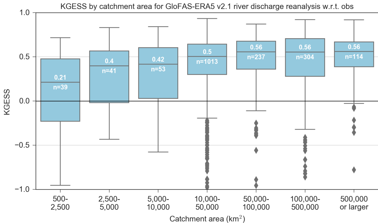
Figure 10: Modified Kling-Gupta Efficiency Skill Score (KGESS) grouped into seven catchment area categories. Boxes and whiskers description as in Fig. 8.
