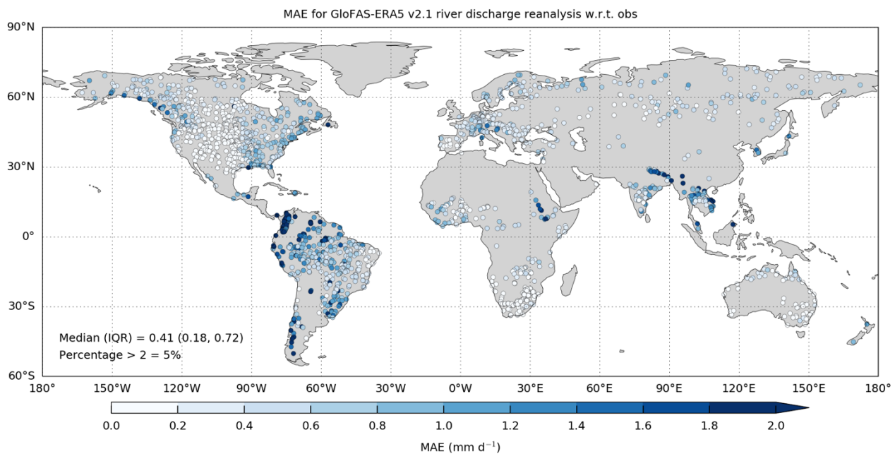
Figure 7: Mean Absolute Error (MAE) for GloFAS-ERA5 reanalysis against 1801 observation stations. Units for both reanalysis and observations have been converted from \text{m}^3 \text{s}^{-1} to runoff depth across the catchment area ( \text{mm d}^{-1} ) to allow direct comparison of the magnitude of errors. Optimum value of MAE is 0, catchments with larger magnitude of errors are darker shades of blue dots.
