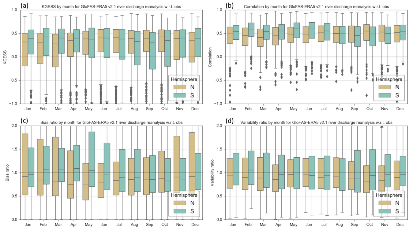
Figure 9: As in Fig. 8 but by hemisphere. Northern hemisphere (n=1268 stations) brown boxes and southern hemisphere (n=533 stations) as green boxes.
