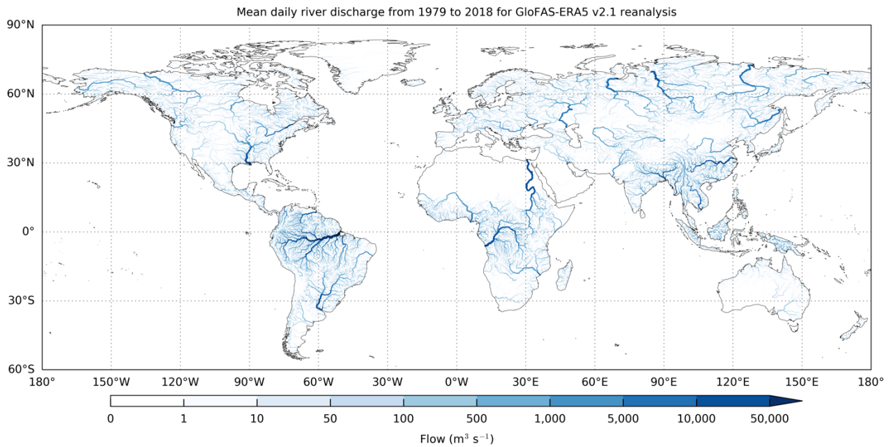
Figure 2: Mean GloFAS-ERA5 daily river discharge over 1979 to 2018 for each GloFAS river grid cell with an upstream area greater than 1000 km 2 . Darker blue river sections have larger river discharge.
