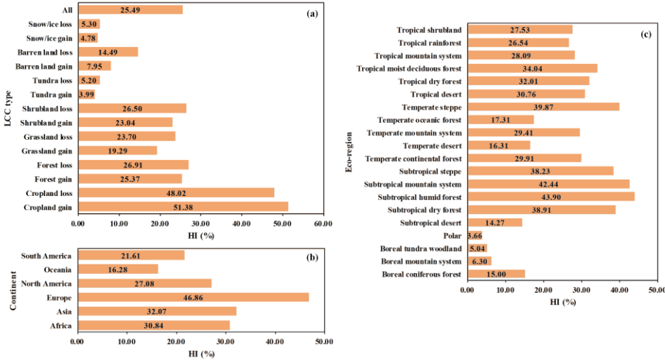
950 Figure 13: The mean human impact (HI) of regions with significant land cover change on the scale of (a) LCC, (b) continents, and (c) eco-regions.
