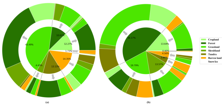
940 Figure 12: Land cover conversions with significant land cover change (LCC) between 1982 and 2015, The inner pie in (a) shows the percentages of different gross gain for each land cover, and the outer ring indicates which land cover the gross gain came from. The inner pie in (b) shows the percentage of different gross loss for each land cover, and the outer ring indicates which land cover the gross loss went to.
