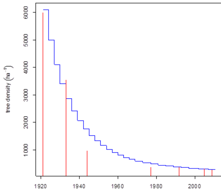
Figure SOM2. Reconstruction of the tree density at Sorø, division 335. During the years from 1921 to, at least, 1944 there was a canopy of old trees. The blue step function is the reconstructed series using the thinning intervals as in Møller (1933) and thinning intensities that match the observations best (red bars, see Table SOM14).
