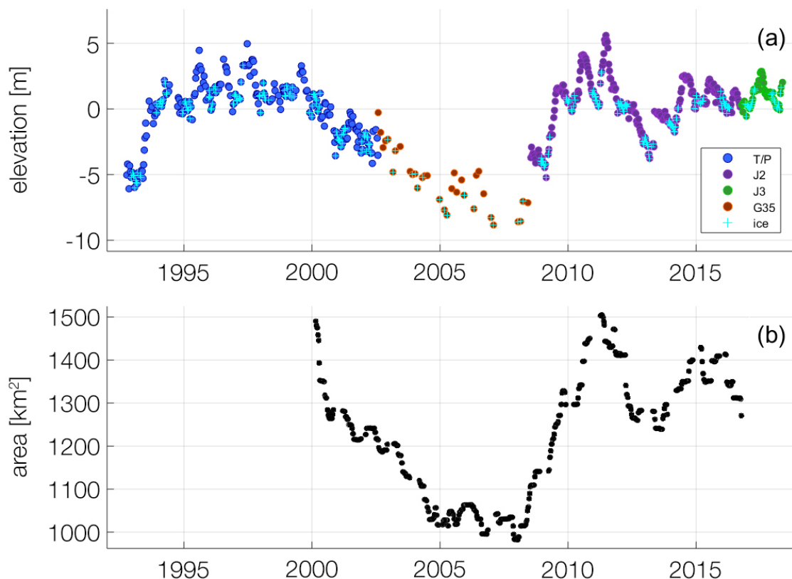
5 Figure 5: Time series of (a) water elevation variation by mission (1144 records) and (b) MODIS-estimated surface area (578 records) for Lake Sakakawea. Presence of surface ice is indicated by a light blue cross.
