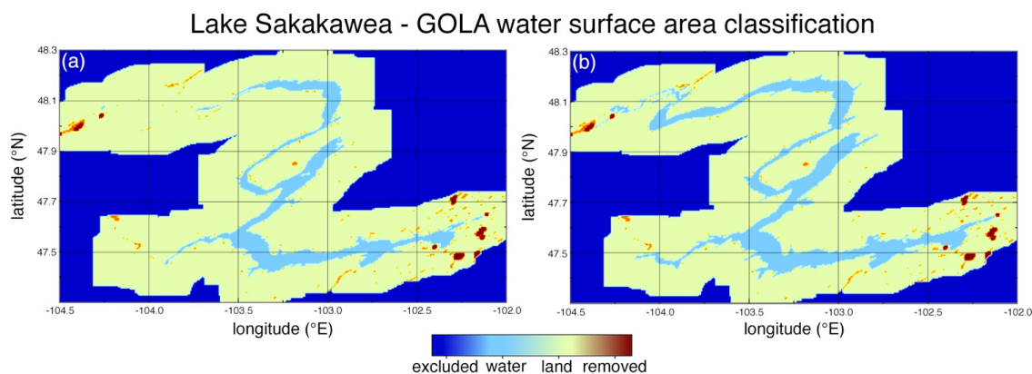
10 Figure 3: Examples of the GOLA WSA classification results for Lake Sakakawea: (a) dry scenario (November 1st, 2008); (b) wet scenario (April 25th, 2011). Differences in WSA estimates are noticeable in the northwestern and southwestern branches of the reservoir, the farthest from the Garrison Dam.
