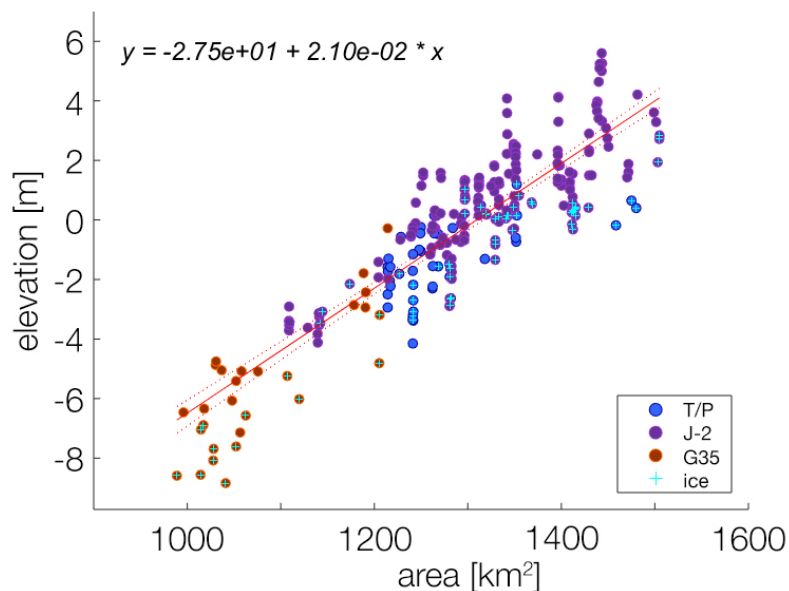
Figure 6: Water elevation and surface area relationship for Lake Sakakawea (277 records).
