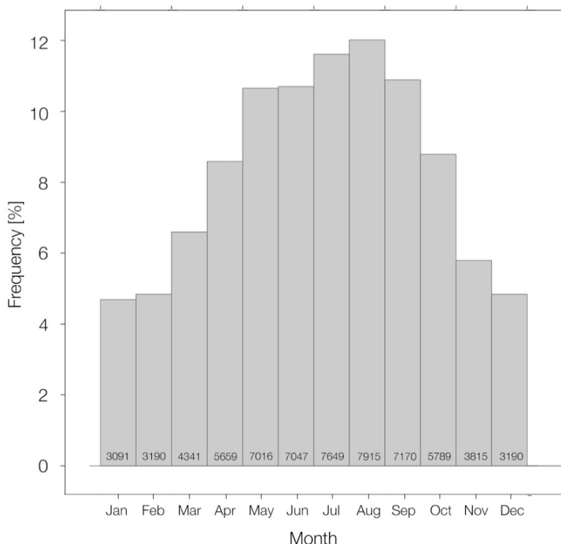
5 Figure 4: Monthly frequency of the observations used to create the hypsometric curve for the 347 targets analyzed in this study, with total number of observations for each month.
