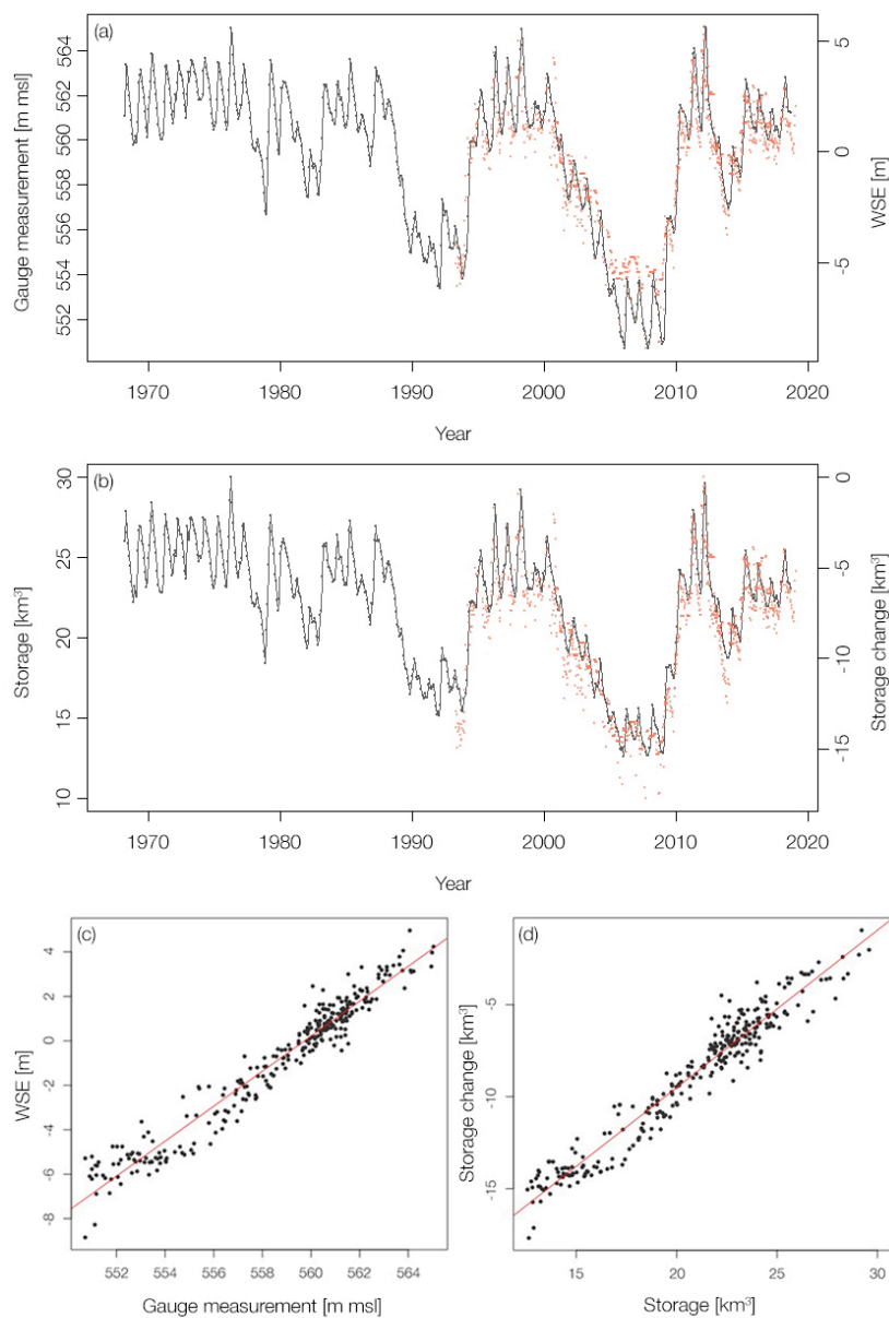
5 Figure 8: Water levels and storage at Lake Sakakawea. (a) In situ monthly water levels (black) versus WSE records (red); (b) in situ monthly water storage (black) versus \Delta V records (red); (c) linear regression of monthly average WSE records and concurrent in situ monthly water levels, with linear regression in red; (d) linear regression of monthly average \Delta V records and concurrent in situ monthly water storage, with linear regression in red.
