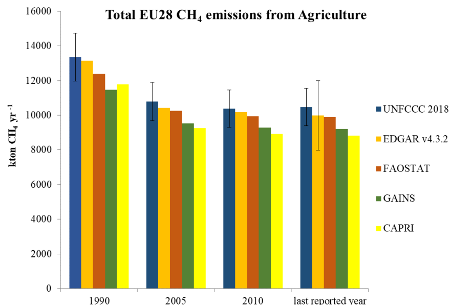
Figure 2. Total EU28 Agriculture CH 4 emissions from five data sources, UNFCCC NGHGI 2018 submissions, EDGAR, FAOSTAT, CAPRI and GAINS. The relative error on the UNFCCC value, computed with the 95% confidence interval method, is 10 %. It represents the NGHGI 2018 uncertainty for the agriculture data reported to UNFCCC. Uncertainty for EDGAR v4.3.2 was calculated for 2012 and is 20 %; it represents the 95 % confidence interval of a lognormal distribution. Last reported year in this study refers to 2016 (UNFCCC and FAOSTAT), 2012 (EDGAR), 2015 (GAINS) and 2013 (CAPRI). The positive values represent a source.
