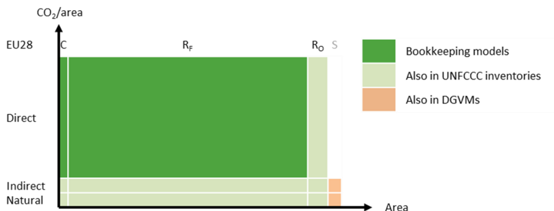
Figure 14: A conceptual extension of Figure 12, applied to EU28, to disaggregate the managed land into the components reported in the UNFCCC inventories. The vertical axis represents density, horizontal axis area, and the area of each box is the CO_2 emissions. The diagram is conceptual and not to scale, but it does give an indication of how the components may look in the EU28. The converted land (C) is equivalent to afforestation plus deforestation. Remaining land is split into remaining forestry ( R_F ) and remaining other (ecological and social functions) ( R_o ) and the sink (S) belongs to unmanaged land. Bookkeeping models consider only direct effects (dark green), but do not include transitions between cropland and pasture or land management changes (increasing tillage, introducing irrigation etc.). UNFCCC CRFs include all dark and light green components (direct, indirect, natural on managed land) while DGVMs in principle can include all components including the sink (pink).
