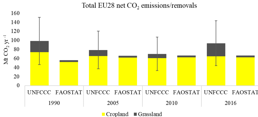
Figure 11: Total EU28 net CO 2 emissions/removals from FAOSTAT and UNFCCC NGHGI 2018 submission estimates of Cropland and Grassland for 1990, 2005, 2010 and 2016. The relative error on the UNFCCC value, computed with the 95 % confidence interval method, is 53 %. It represents the NGHGI 2018 uncertainty for the CL and GL data pool reported to UNFCCC.
