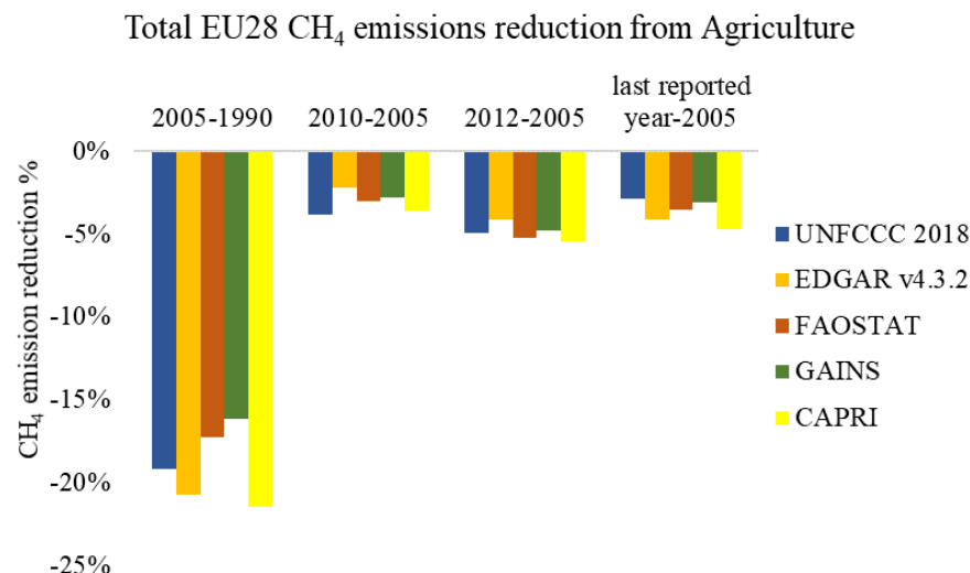
Figure 3: Change of EU28 total agricultural CH 4 emissions between different years. 2012 is the last common year when all sources have estimates. Last reported year in this study refers to 2016 (UNFCCC and FAOSTAT), 2012 (EDGAR), 2015 (GAINS) and 2013 (CAPRI).
