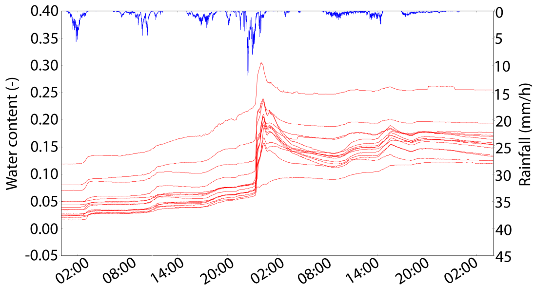
Figure 8. Rainfall and Volumetric Water Content ( \text{m}^3 \cdot \text{m}^{-3} ) for 16 TDR sensors on the 29-30 th April 2018 event
