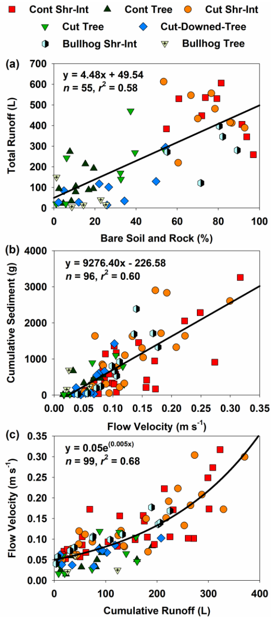
Figure 5. Example relationships/correlations in runoff and bare ground (bare soil plus rock cover; a ), cumulative sediment and overland flow velocity ( b ), and overland flow velocity and runoff ( c ) derived from a subset of the overland flow dataset for Marking Corral and Onaqui sites, as presented in Williams et al. (2019a). Data from overland flow simulations on untreated/control (Cont) plots, cut treatment (Cut) plots without and with a cut, downed tree (Cut-Downed Tree), and bullhog plots (Bullhog, Onaqui site only) in tree (Tree) and intercanopy (shrub-interspace, Shr-Int) microsites 9 yr after respective tree removal treatments. The data demonstrate that, for the studied conditions, runoff is largely regulated by bare ground, sediment delivery is controlled by flow velocity, and flow velocity is strongly correlated with the amount or runoff.
