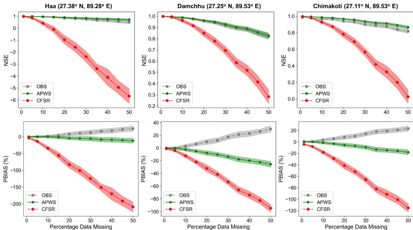
Fig. 7 NSE and PBIAS in WRB computed using reference flows and simulated flows using weather statistics from OBS, APWS and CFSR for different scenarios of missing data (bands here represent the NSE and PBIAS values computed for 100 bootstraps) in WRB
