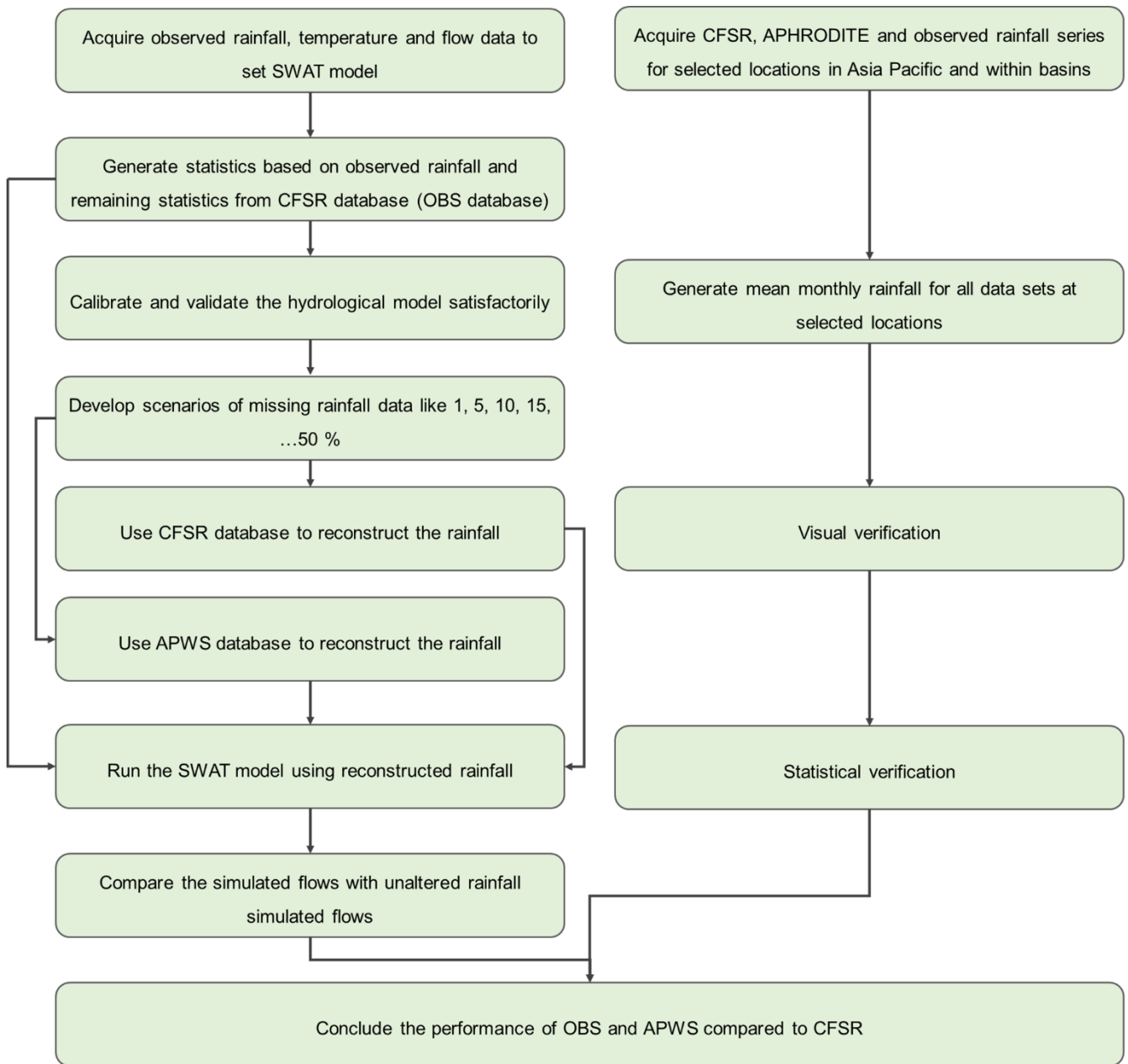
Fig. 3 Performance evaluation of APWS for selected river basins of Asia
