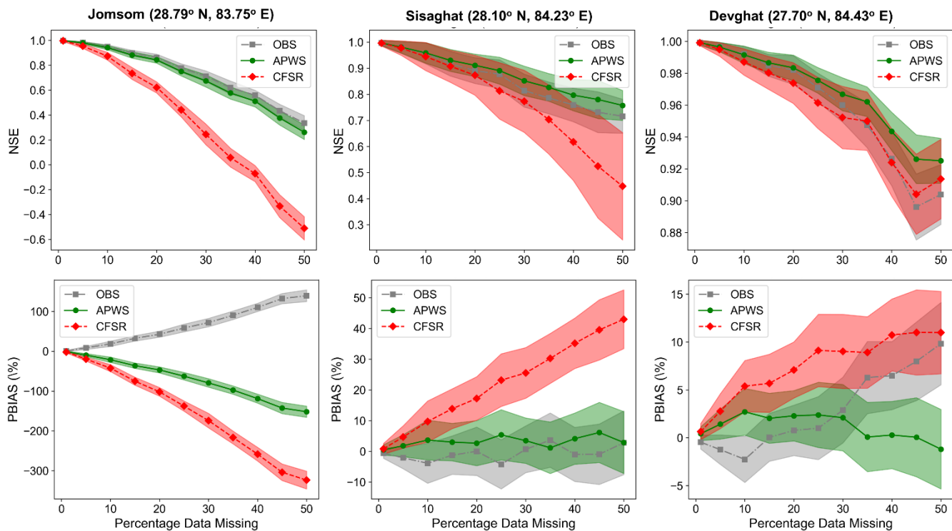
600 Fig. 8 NSE and PBIAS in NRB computed using reference flows and simulated flows using weather statistics from OBS, APWS and CFSR for different scenarios of missing data (bands here represent the NSE and PBIAS values computed for 100 bootstraps) in NRB
