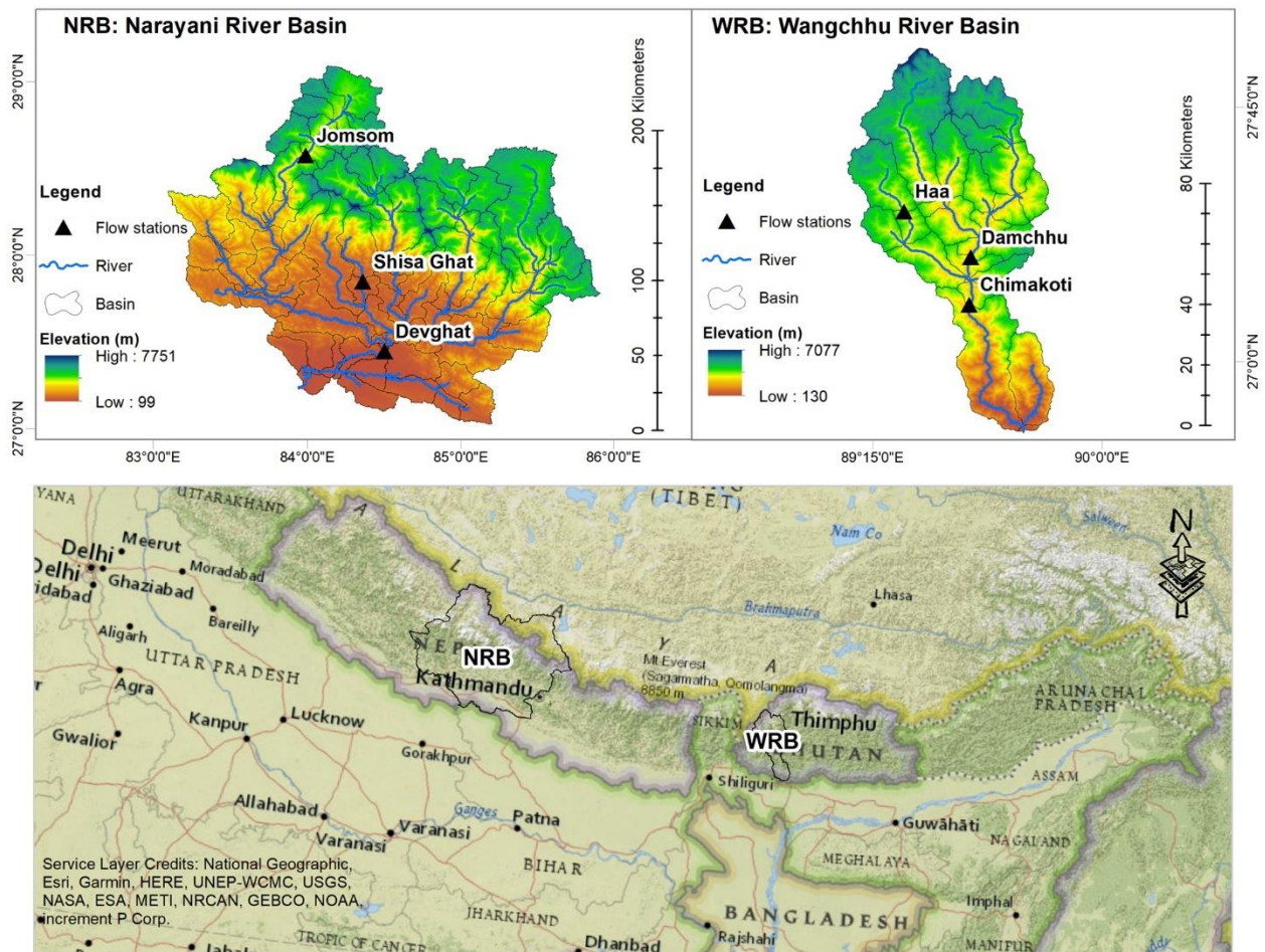
580 Fig. 4 Location of the test basins in Asia Pacific region and their elevational information
