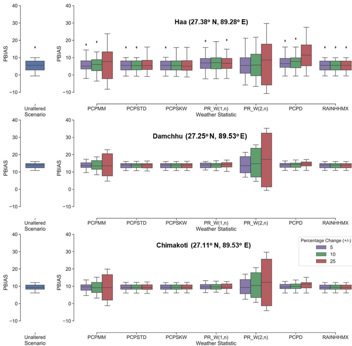
Fig. 9 Sensitivity analysis of rainfall statistics in simulating daily flows at Haa, Damchhu and Chimakoti flow stations in the Wangchhu river basin, Bhutan
