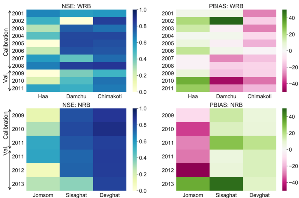
Fig. 6 NSE (left column) and PBIAS (right column) computed from daily simulated and observed flows for each year in top, middle and lower parts (left to right of each plot) in WRB (top row) and NRB (bottom row)
