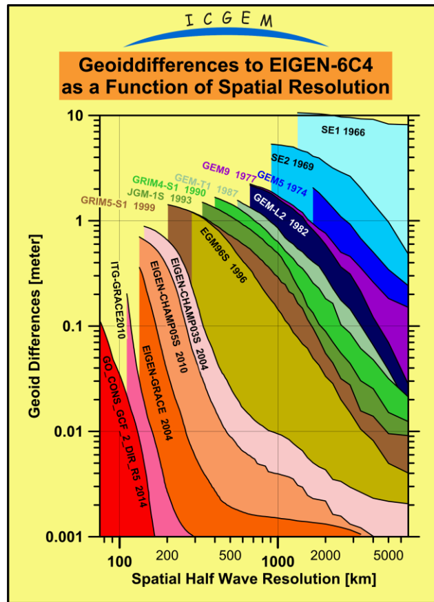
Figure 1: a) Number of static gravity field models released per year since 1966. Note the increased number of models due to the launch of the dedicated satellite gravity missions (CHAMP, GRACE and GOCE) after 2003 and 2011. b) The history of the improvement of the spatial resolution and the accuracy of the satellite only gravity field models. Signal amplitude difference over the years w.r.t. one of the latest combined global gravity field models, EIGEN-6C4 is shown ( http://icgem.gfz-potsdam.de/History.png ). Note that the EIGEN-6C4 is not the truth but a better approximation to the real gravity field, because it is a combination of data retrieved from satellite missions, terrestrial measurements, and altimetry-derived gravity field information. The uncertainties of the geoid signal have been reduced together with improved spatial resolution. See also the large improvement between the EGM96S and EIGEN-CHAMP03 due to the contribution of the CHAMP measurements.
