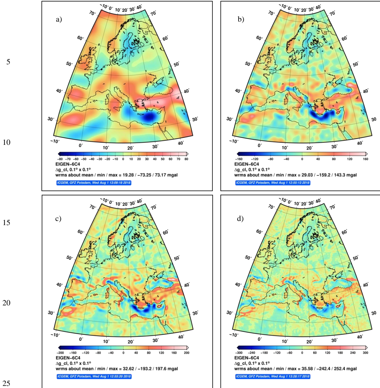
Figure 8: Geographical distribution of gravity anomalies in mGal with different spectral ( l_{max} ) and spatial resolution (half wavelength \lambda_{min}/2 ) of EIGEN-6C4. Spherical harmonic degree expansions for the four examples are as follows: a) 50 b) 150 c) 250 d) 500 which correspond to 400, ~133, 80 and 40 km half wavelength spatial resolution, respectively. See the refined features and better spatial localisation as the model expansion increases. For instance, topographical features such as mountains are well resolved in Figure 8d, whereas they are not precisely located in Figure 8a. The transmission borders of higher and lower anomalies in Alps and Mediterranean Sea are better resolved in Figure 8d, whereas it is not possible to distinguish and locate them precisely in Figure 8a. Note the different colour scales which have not been changed and kept as retrieved from ICGEM.
