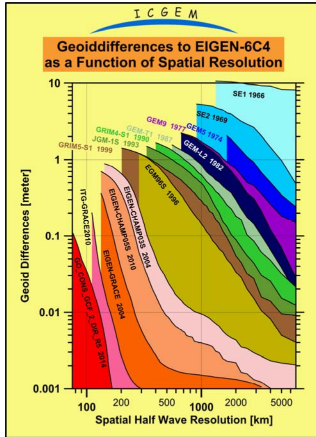
Figure 1: a) Number of static gravity field models released per year since 1966. Note the increased number of models due to the launch of the dedicated satellite gravity missions (CHAMP, GRACE and GOCE) after 2003 and 2011. b) The history of the improvement of the spatial resolution and the accuracy of the satellite only gravity field models. Signal amplitude difference over the years w.r.t. one of the latest combined global gravity field models, EIGEN-6C4 is shown ( http://icgem.gfz-potsdam.de/History.png ). Note that the EIGEN-6C4 is not the truth but a better approximation to the real gravity field, because it is a combination of data retrieved from satellite missions, terrestrial measurements, and altimetry-derived gravity field information. The uncertainties of the geoid signal have been reduced together with improved spatial resolution. See also the large improvement between the EGM96S and EIGEN-CHAMP03 due to the contribution of the CHAMP measurements.
