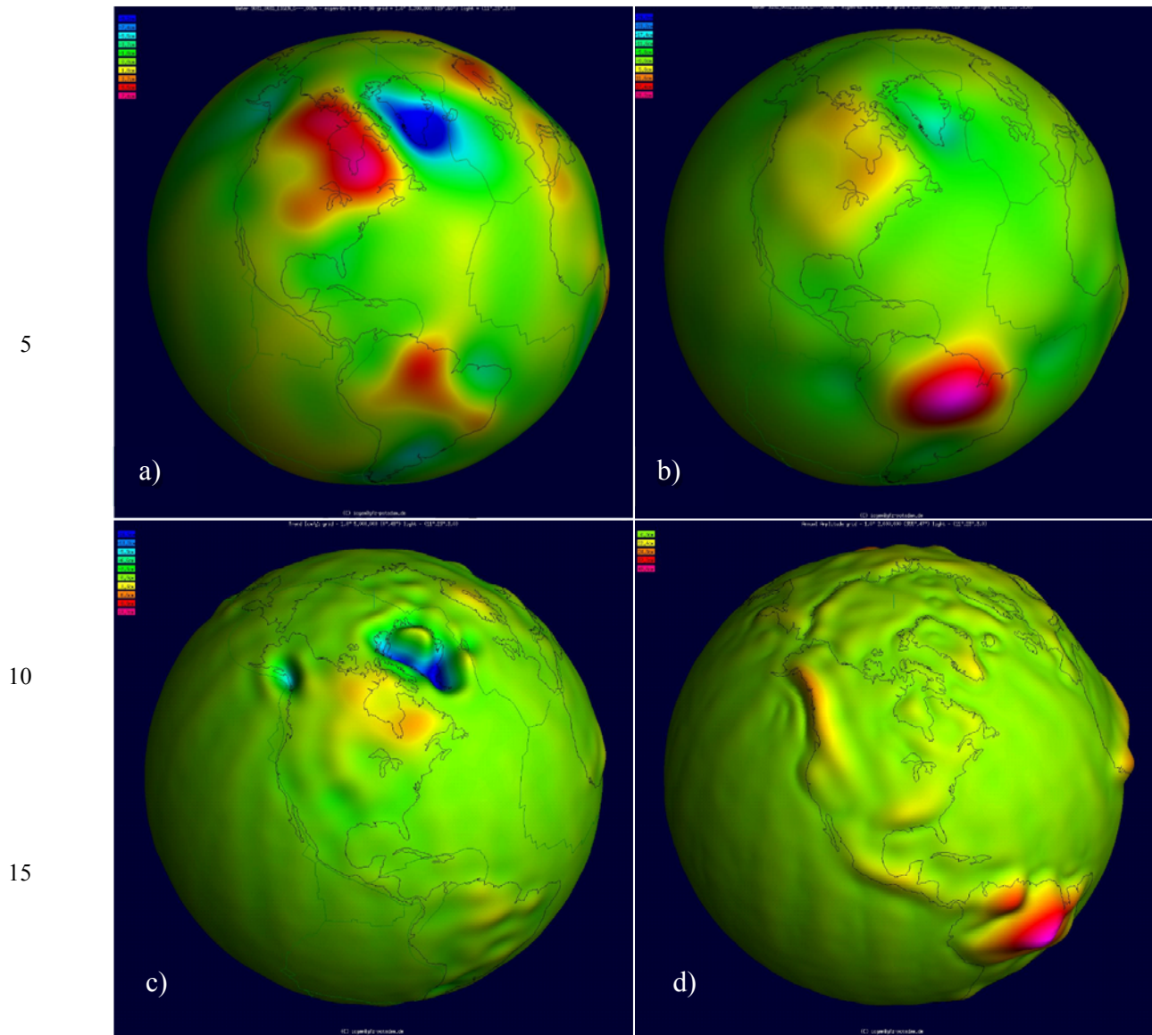
20 Figure 15: Snapshot of Visualisation Service for temporal models a) EWH in January 2009 b) EWH in May 2009, note that the EWH difference between the two months represents the mass change, c) trend, note the strong effect due to the GIA in Hudson Bay area, Canada and Alaska and ice melting in Greenland d) annual amplitude, where the large signal amplitude in the Amazon region is noticeable.
