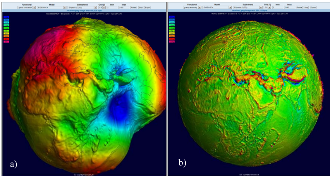
Figure 13: Examples of Visualisation Service for a) geoid undulation and b) gravity anomaly computed from a high resolution combined static gravity field model.
