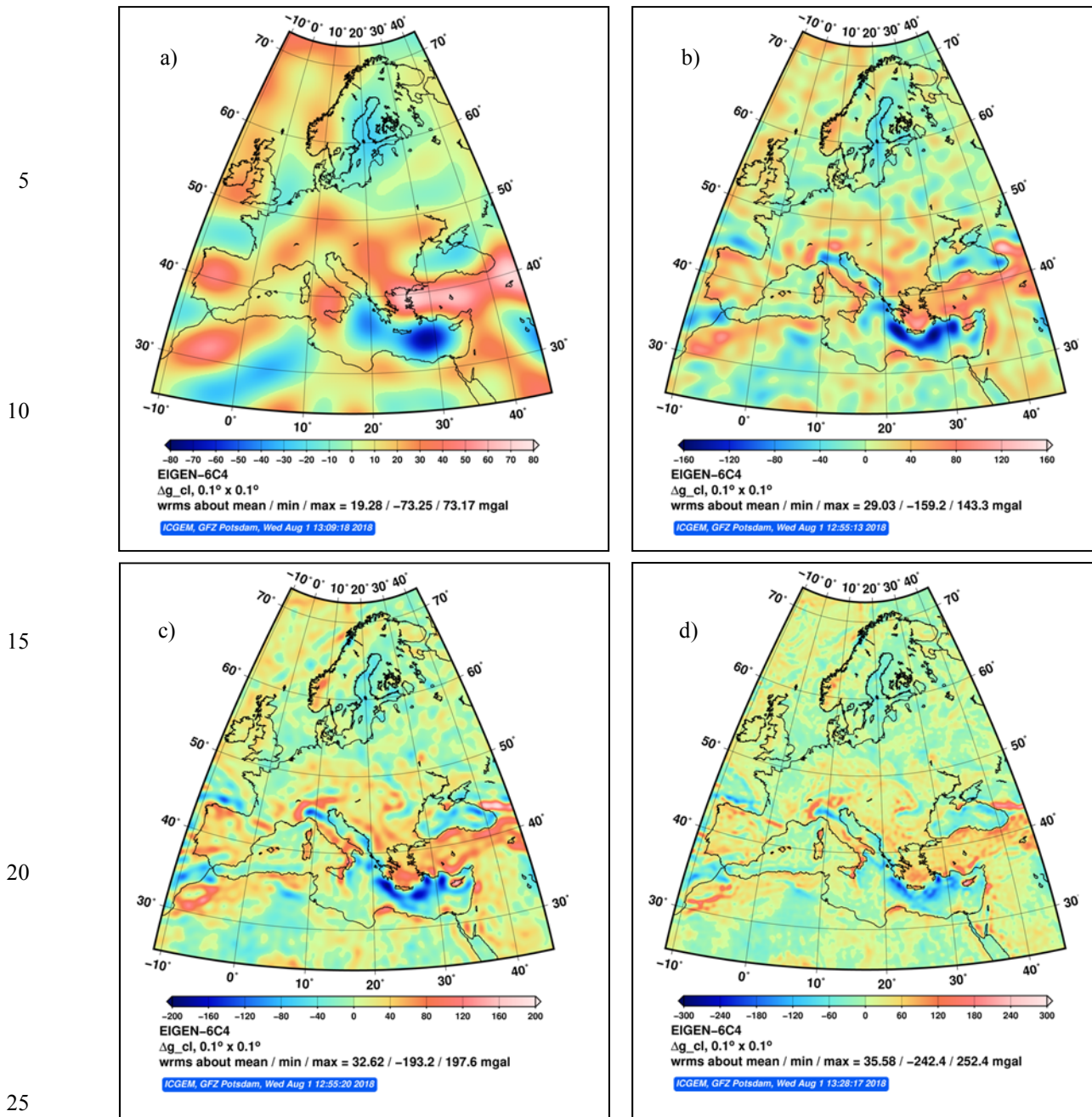
Figure 8: Geographical distribution of gravity anomalies in mGal with different spectral ( l_{\max} ) and spatial resolution (half wavelength \lambda_{\min}/2 ) of EIGEN-6C4. Spherical harmonic degree expansions for the four examples are as follows: a) 50 b) 150 c) 250 d) 500 which correspond to 400, ~133, 80 and 40 km half wavelength spatial resolution, respectively. See the refined features and better spatial localisation as the model expansion increases. For instance, topographical features such as mountains are well resolved in Figure 8d, whereas they are not precisely located in Figure 8a. The transmission borders of higher and lower anomalies in Alps and Mediterranean Sea are better resolved in Figure 8d, whereas it is not possible to distinguish and locate them precisely in Figure 8a. Note the different colour scales which have not been changed and kept as retrieved from ICGEM.
