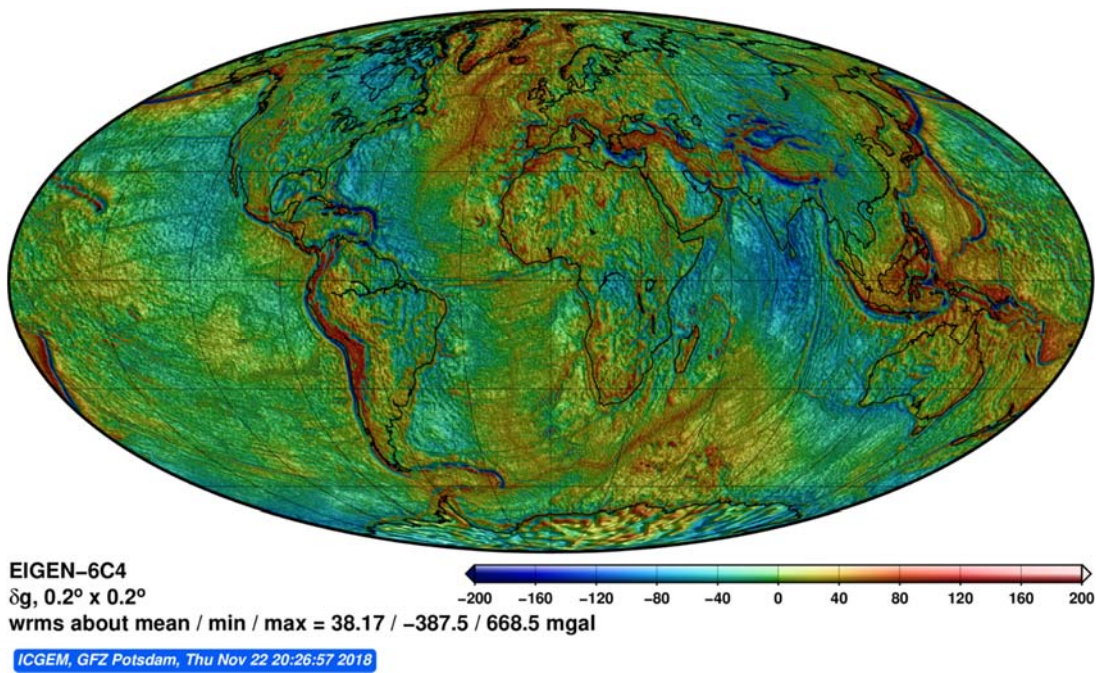
5 Figure 78: Gravity disturbance computed on the Earth surface from EIGEN-6C4 combined gravity field model expanded up to degree and order 2190.
