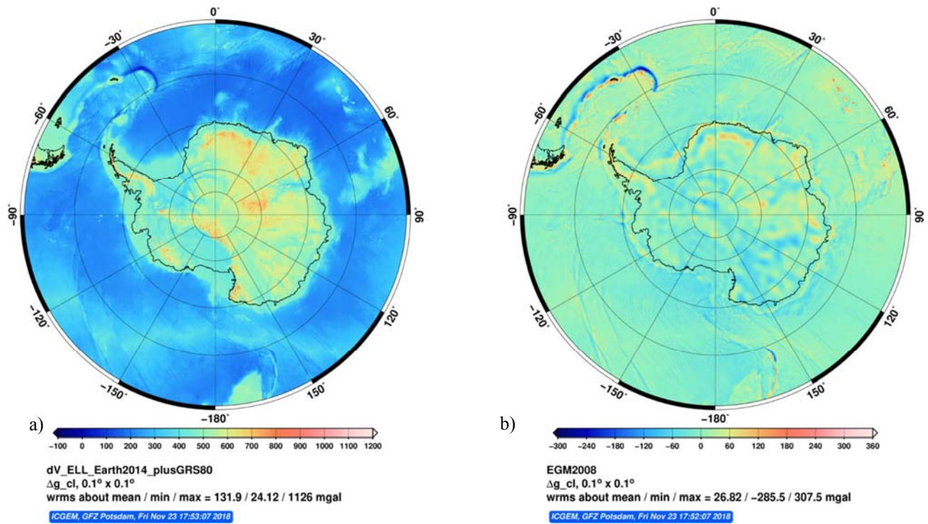
Figure 210: The classical gravity anomalies which are also known as free air gravity anomalies computed on the Earth’s surface based on a) topographic model dV_ELL_Earth2014_plusGRS80 and b) EGM2008 using models highest degree/order available , 2190. It is clearly seen that the features in Antarctica are better resolved in a. Note that the scale is left-kept as is for individual cases on purpose since the current-present forms shape of the figures are what exactly the ICGEM Calculation Service provides.
