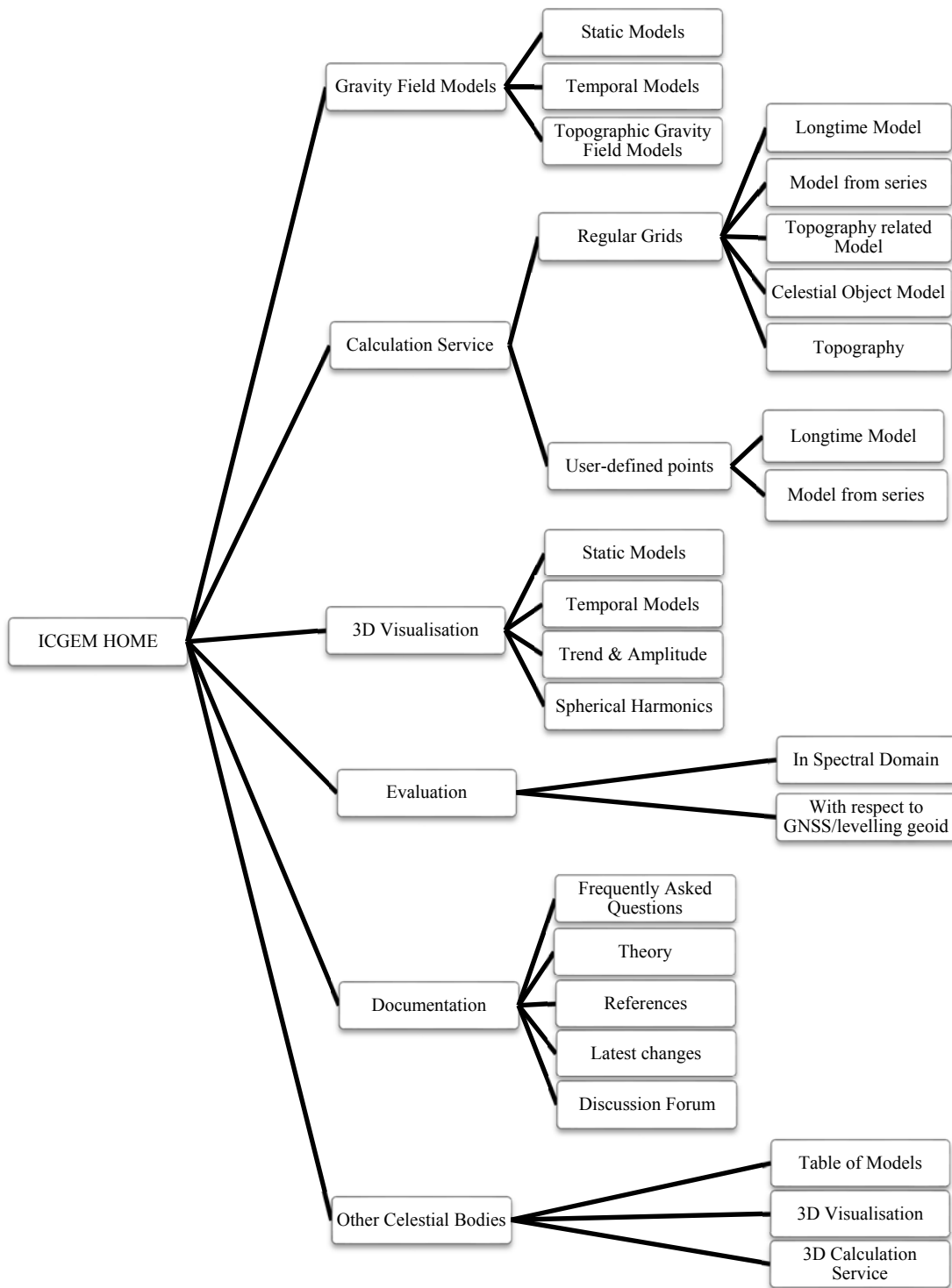
Figure 34: The homepage structure of the new ICGEM service website.
