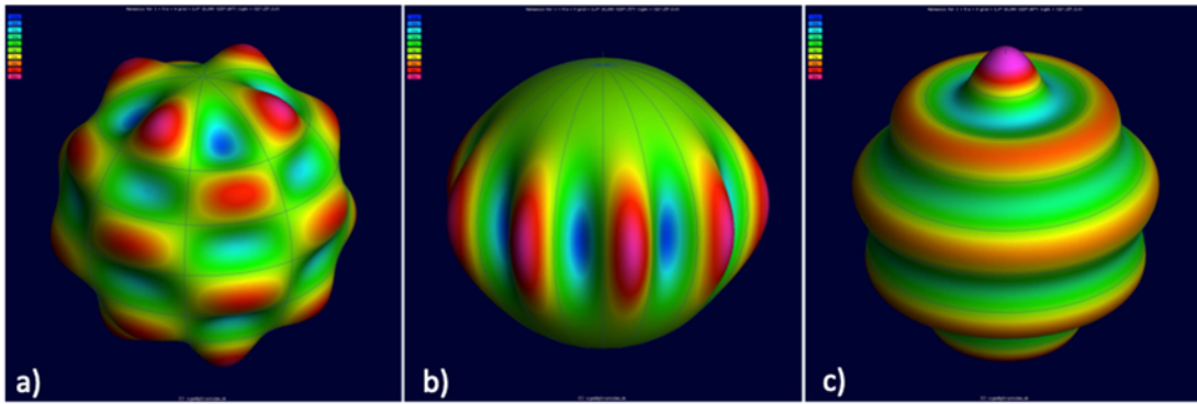
Figure 45: 3D Visualisation of spherical harmonics as tutorial. The images show one specific surface spherical harmonic of degree l and order m such as a) tesseral ( l=9, m=4 ) b) sectorial ( l=9, m=9 ) c) zonal ( l=9, m=0 ) spherical harmonics.
