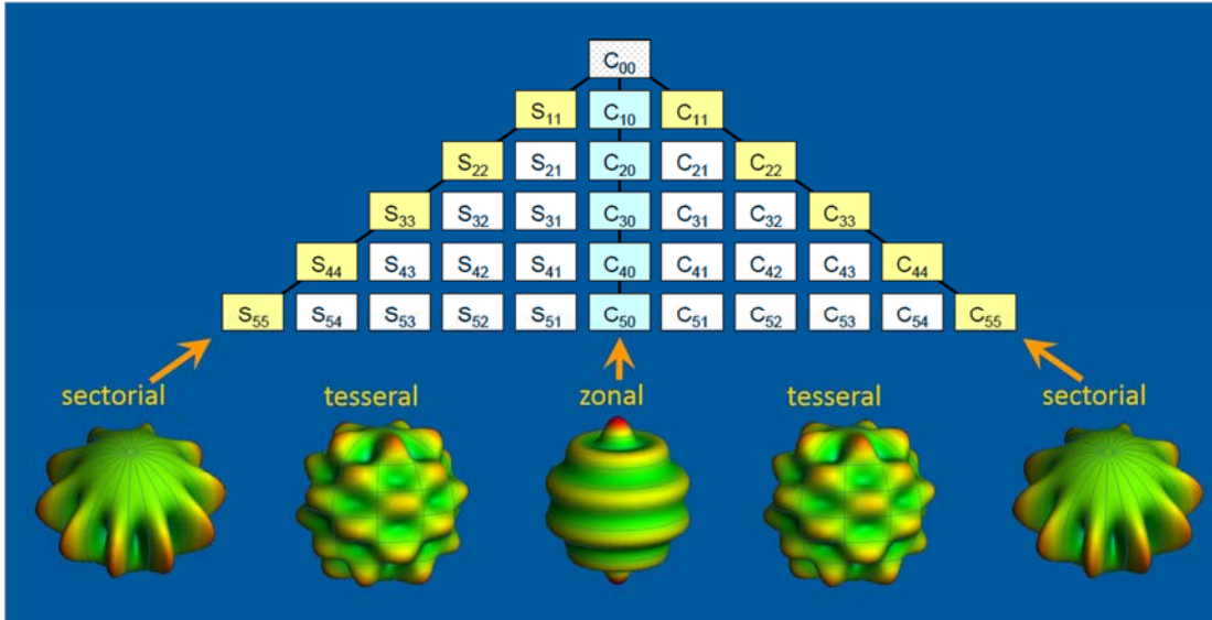
5 Figure 56: Mathematical representation of gravitational field potential using sectorial, tesseral and zonal spherical harmonics. A spherical approximation of the gravitational field up to maximum degree of l_{max} consists of (l_{max}+1)^2 coefficients (credit Barthelmes, F.).
