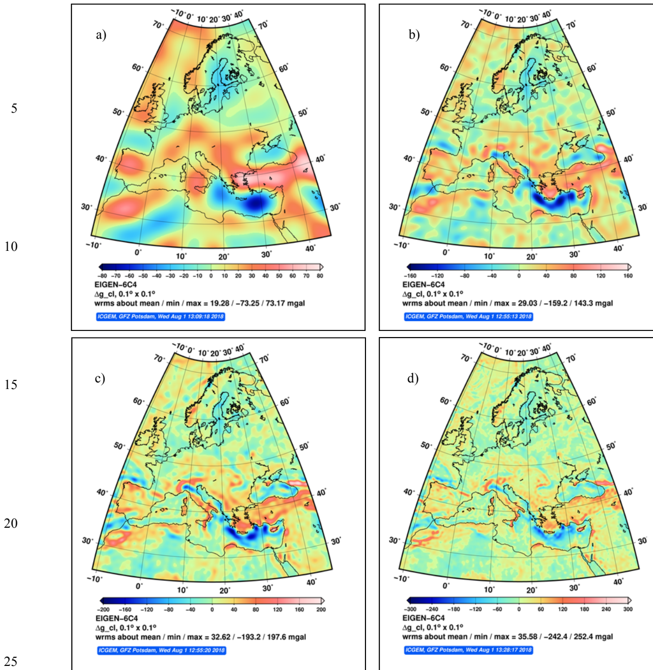
Figure 89: Geographical distribution of gravity anomalies in mGal with different spectral ( l_{\max} ) and spatial resolution (half wavelength \lambda_{\min}/2 ) of EIGEN-6C4. Spherical harmonic degree expansions for the four examples are as follows: a) 50 b) 150 c) 250 d) 500 which correspond to 400, ~133, 80 and 40 km half wavelength spatial resolution, respectively. See the refined features and better spatial localisation as the model expansion increases. For instance, topographical features such as mountains are well resolved in Figure 9a8d, whereas they are not precisely located in Figure 9a8a. The transmission borders of higher and lower anomalies in Alps and Mediterranean Sea are better resolved in Figure 9d8d, whereas it is not possible to distinguish and locate them precisely in Figure 9a8a. Note the different colour scales which have not been changed and kept as retrieved from ICGEM.
