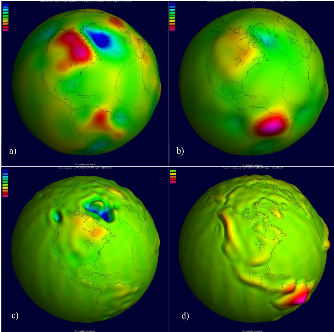
25 Figure 1516: Snapshot of Visualisation Service for temporal models a) EWH in January 2009 b) EWH in May 2009, note that the EWH difference between the two months represents the mass distributionschange , c) trend, note the strong effect due to the GIA in Hudson Bay area , Canada and Alaska and ice melting in Greenland d) annual amplitude, where the large signal amplitude in the Amazon region is noticeable.
