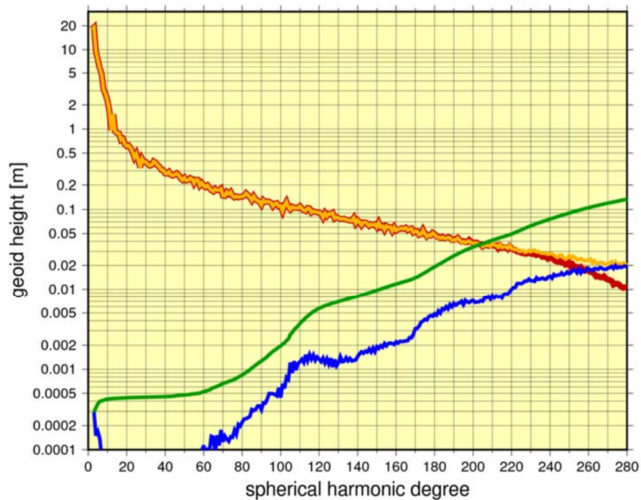
Figure 1617: Spectral comparison of two static global gravity field models, GOCO05S and EIGEN-6C4. Note that the comparisons are performed for each degree separately. GOCO05S is a satellite only model, whereas the EIGEN6C4 is a combined model that uses both the satellite and terrestrial measurements. The blue curve represents the difference in the amplitude of the GOCO05S and EIGEN-6C4 combined static gravity field models per degree, whereas the green line represents the cumulative difference amplitudes as a function of the maximum degree of the two models as a function of maximum degree . See the increasing difference as the degree increases due to the contribution of the terrestrial gravity data to EIGEN-6C4.
