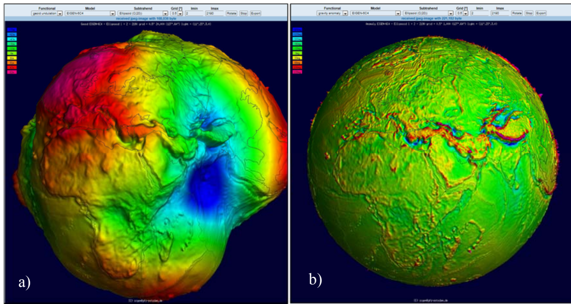
5 Figure 131314: Examples of Visualization Service for a) geoid undulation and b) gravity anomaly computed from a high resolution combined static gravity field model.
