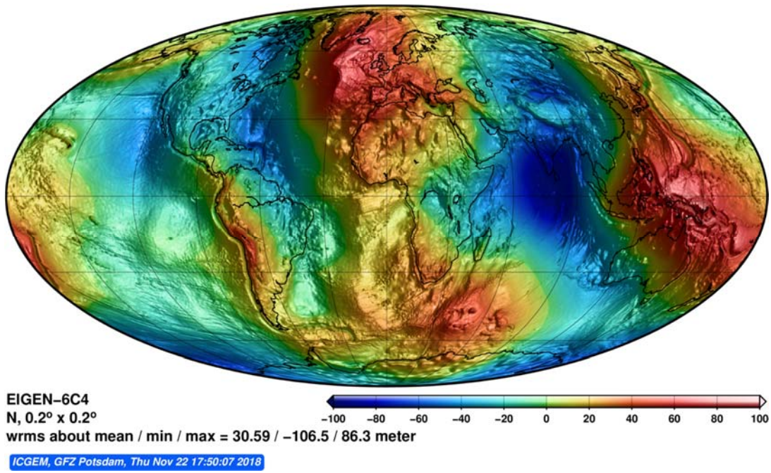
Figure 67: Geoid undulation computed from EIGEN-6C4 combined gravity field model expanded up to degree and order 2190.
