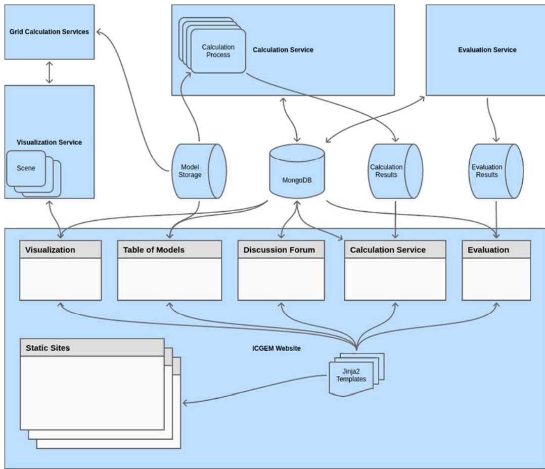
Figure 2021: Illustration of the scheme of the ICGEM Website in terms of its web programming. Arrows indicate the direction of data flows. Cylinders are the default symbol for Databases and sideways cylinders are used for file-based data stores. Model Storage is file based, the Calculation Results are the calculated Grid files and the images converted from them. Evaluation Results are only the generated images on the Spectral domain page, the values in the GNSS/levelling page derive from the MongoDB. At the bottom of the scheme, every grey-white rectangle represents a subpage on the Website. Similar pages, like the different Visualization pages or the Tables of Models, are presented together, and we included only the static pages, that are more interesting from a technical perspective.
