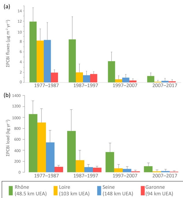
Figure 5. Comparison of specific \Sigma\text{PCBi} flux ( \mu\text{g m}^{-2} \text{yr}^{-1} ) (a) and the mean annual load ( \text{kg yr}^{-1} ) (b) on the French rivers. Fluxes and loads are estimated at the lower station upstream of the tidal influence: Arles–Beaucaire for the Rhône, Montjean for the Loire, Poses–Poissy for the Seine and La Réole–Lamagistère for the Garonne (see locations in Fig. 1). The distance of each station to the sea is expressed as kilometres upstream of estuarine areas (km UEA).
