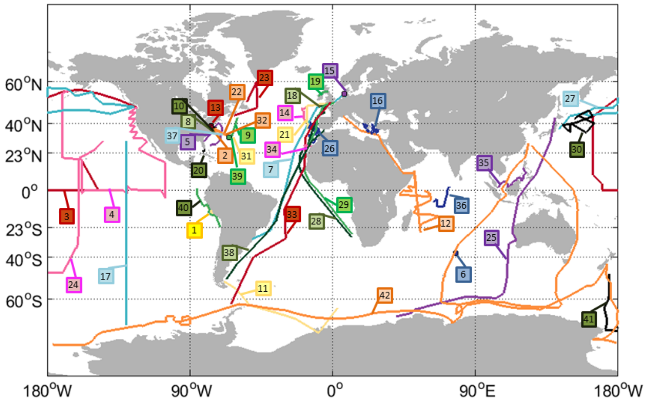
Figure 1: Tracks of all cruises with OCS and/or CS 2 measurements included in the database (points depict stationary measurements). Labels indicate the cruise ID (compare Tab. 1).
