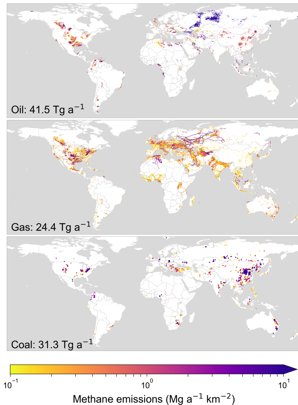
Figure 4. Global distribution of 2016 methane emissions from oil, gas, and coal in our inventory. The inventory is at 0.1° x 0.1° grid resolution but coal is shown here at 1° x 1° resolution for visibility. Emissions below 10 -1 Mg a -1 km -2 are not shown.
