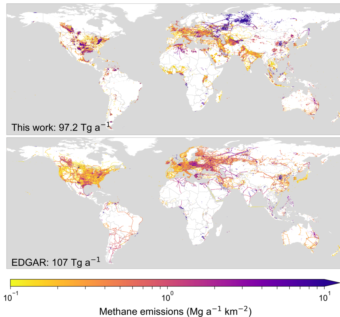
Figure 5. Total methane emissions from fuel exploitation (sum of oil, gas, and coal) in 2016 from this work (top) and in 2012 from EDGAR v4.3.2 (bottom; European Commission, 2017). Emissions below 10^{-1} Mg a -1 km -2 are not shown.
