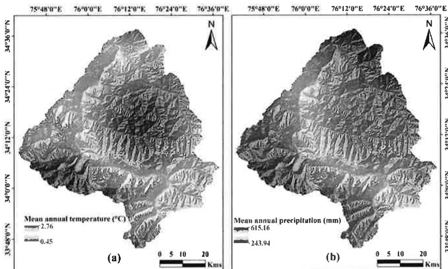
542 Figure 9: Spatial variation in meteorological data recorded for 15 grids in the SSB during the period 1901-2017. 543 Map showing the long term mean annual (a) temperature (°C) and (b) precipitation (mm) data within the sub- 544 basin suggesting the existence of significant local climate variability in the region. Glacier boundaries are shown 545 as: GHR (red) and LR (yellow). 546
