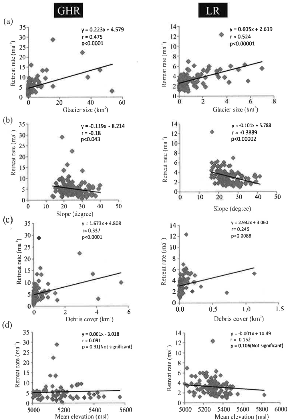
Figure R4b. Scatter plots displaying the relation between topographic factors with retreat rate during the period 1971-2017. All the relationships were found to be significant at confidence level, i.e., \alpha < 0.05 (Except mean elevation).
