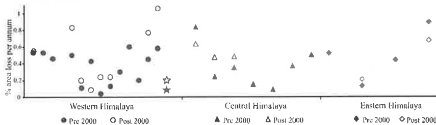
479 Figure 8: Annual rate of percentage area loss of glaciers in three major sections of Himalaya before and after 480 2000. Details of the same have been mentioned in Table S3 of Supplementary sheet. Results from the present 481 study have been star marked in the western Himalaya. 482 483
