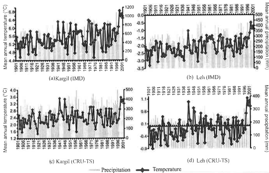
294 Figure 5: Analysis of meteorological (mean annual temperature and precipitation) datasets derived from Indian 295 Meteorological Department (IMD) stations at (a) Kargil & (b) Leh and the respective [(c) Kargil and (d) Leh] 296 gridded data obtained from climate research unit (CRU)-time series (TS). 297
