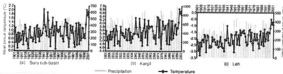
281 Figure 4: Mean annual temperature and precipitation patterns of CRU-TS derived gridded data in (a) Suru sub- 282 basin and IMD recorded station at (b) Kargil and (c) Leh.
