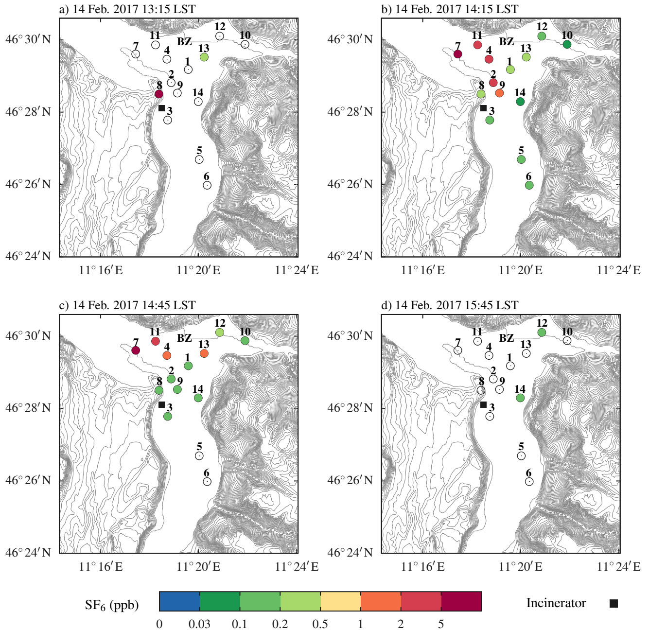
Figure 10. Spatial distribution of the tracer concentrations measured during the release performed in the afternoon of 14 February 2017. The position of the city of Bolzano is indicated in the map with the label BZ.
