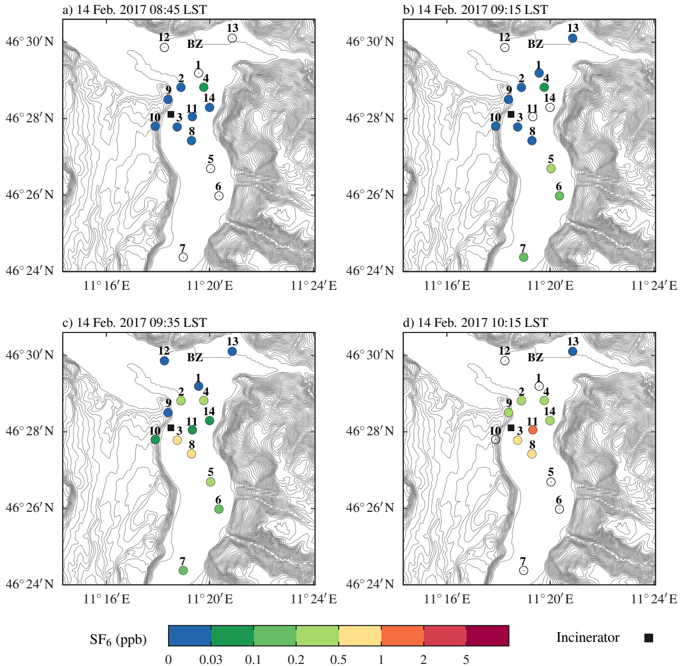
Figure 9. Spatial distribution of the tracer concentrations measured during the release performed in the morning of 14 February 2017. The position of the city of Bolzano is indicated in the map with the label BZ.
