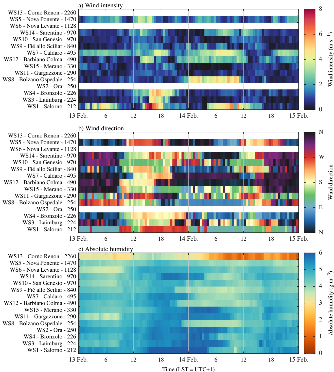
Figure 6. Time evolution of the wind intensity (a), of the wind direction (b) and the absolute humidity (c) measured by the 15 ground surface weather stations used during BTEX (see Tab. 1). The absolute humidity was computed from data of relative humidity, air temperature and atmospheric pressure. Weather stations are ordered according to their elevation, aiming at displaying a pseudo-vertical distribution of the observed quantities.
