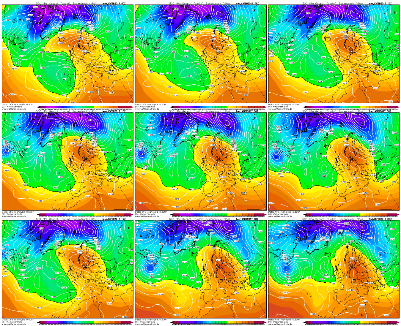
Figure 5. CFS reanalyses of geopotential height at 500 hPa from 20170213 00 UTC to 20170215 00 UTC ( www.wetterzentrale.de ).
