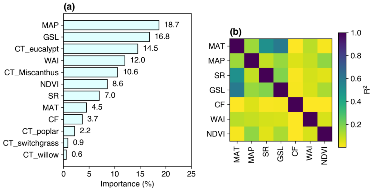
750 Figure 2: Variable importance in the trained RF model (a) and R^2 from the regressions between different explanatory variables (Table 1) in the training data (b). The importance of one variable is calculated based on the sum over the number of splits across all trees that include this variable, weighted by the number of samples it splits. The relative contributions of each explanatory variable (summed to 100%) are shown here.
