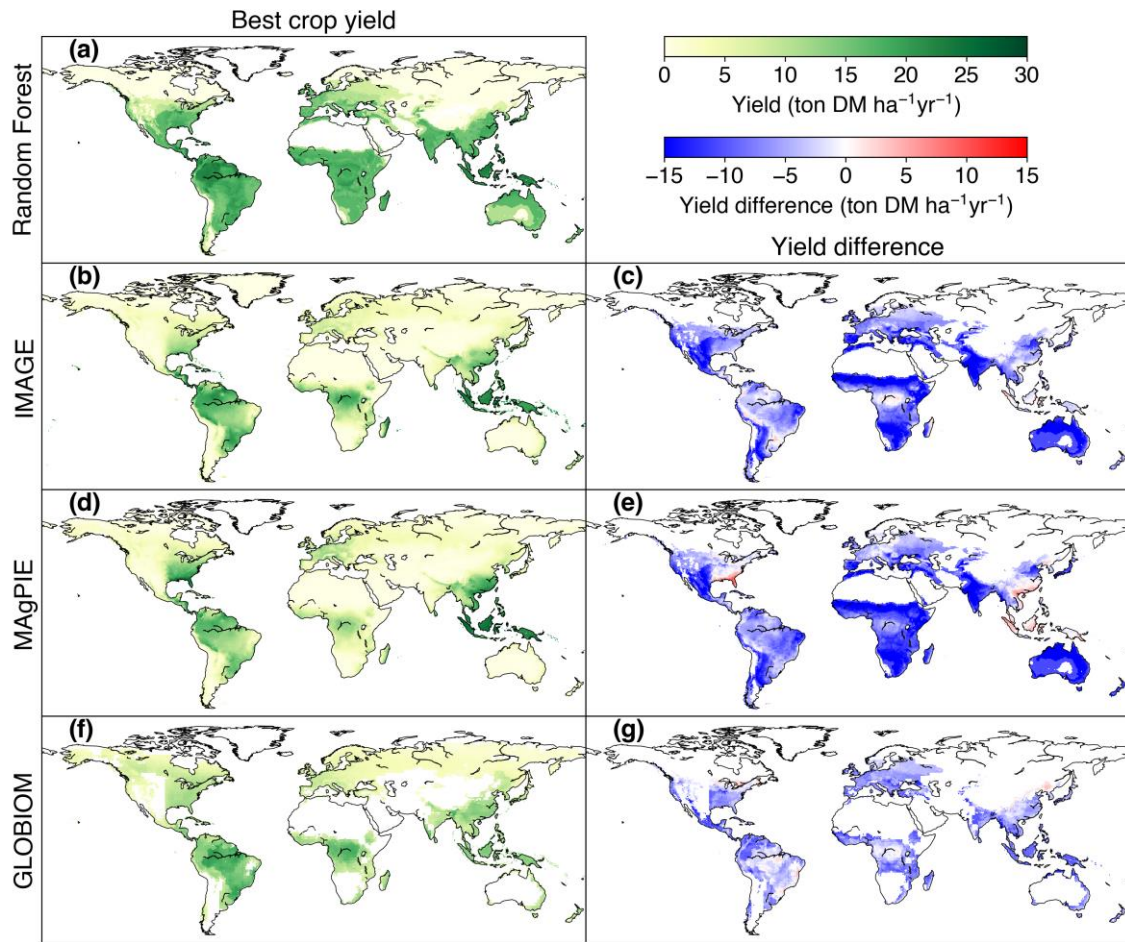
765 Figure 4: Comparison of bioenergy crop yields between the RF map and maps used in three IAMs (IMAGE, MAgPIE and GLOBIOM). The left panel (a, b, d, f) is the best crop yields from each dataset, and the right panel (c, e, g) refers to the yield differences between RF and each IAM maps (IAM yields minus RF yields where yields are available in both paired maps). The best crop yield map from RF (a) is the same as Fig. 3f. The best crop yields in IMAGE and MAgPIE (b, d) are the higher yields between woody and herbaceous bioenergy crops in each grid cell. The best crop yields in GLOBIOM (f) are the yields of woody crops (short-rotation trees) since there is no herbaceous bioenergy crop in GLOBIOM.
