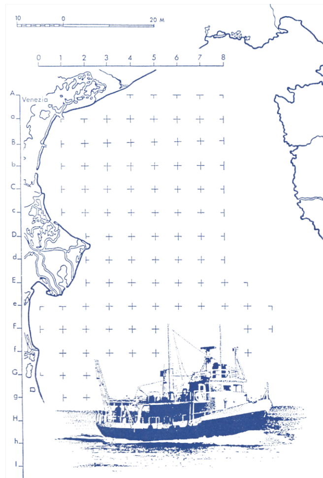
177 178 179 Figure 2 - An example of sampling stations based on the regular grid created in the NAS for the cruises from 1966 to 1980 180 (from Franco, 1972). 181
