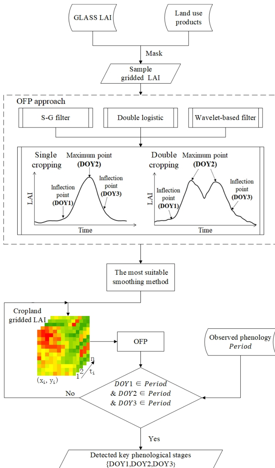
510 Fig.2: Flow chart of procedures for data analysis and crop phenological dates identification.
