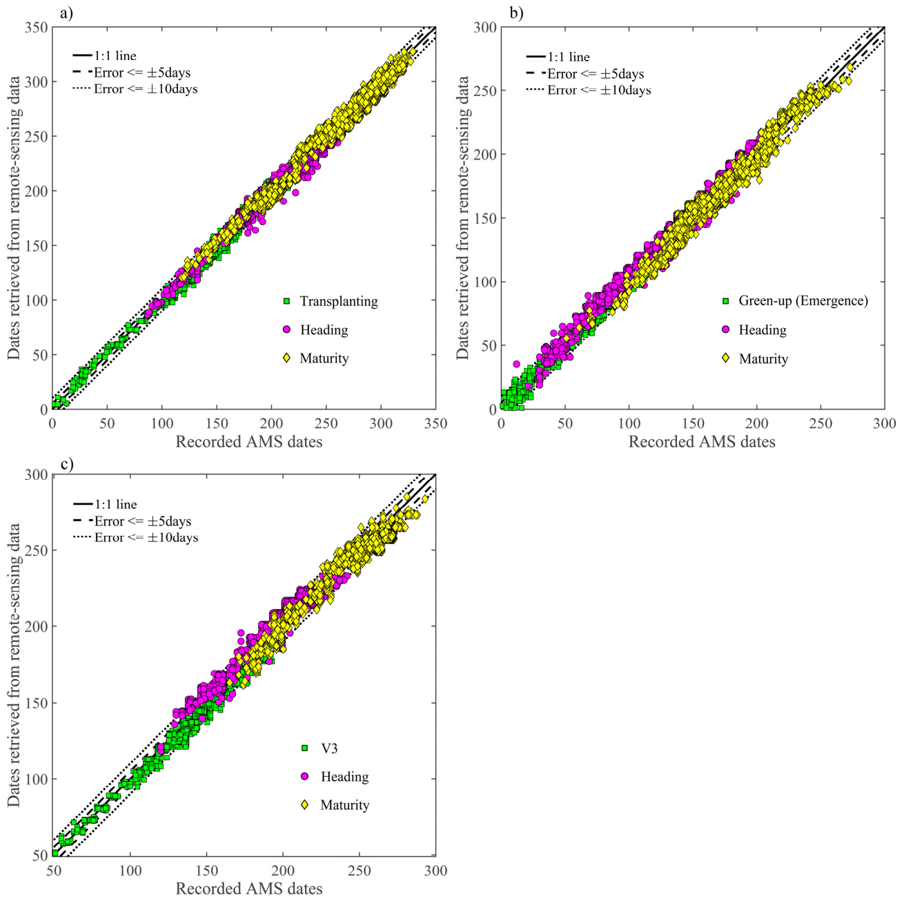
560 Fig.5: Comparisons between retrieved and observed phenological dates for rice (a), wheat (b), and maize (c).
