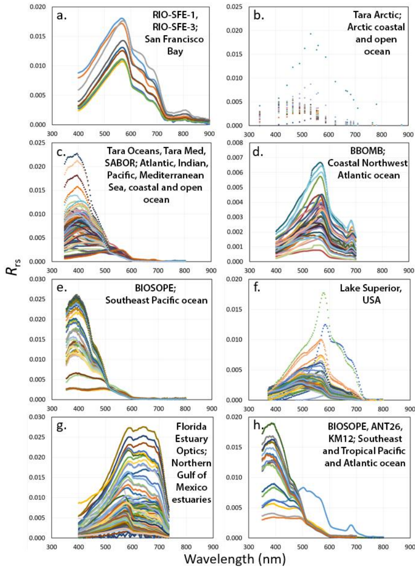
840 Figure 4: Plots demonstrate spectral reflectance diversity of inland, estuary, and ocean environments. (location information is provided in the Figure 3 global map) . Reflectance distribution plots display R_{rs} data from (a.) San Francisco Bay waters (Ackleson) , (b.) Arctic coastal and open ocean (Boss/Chase Arctic) , (c.) Atlantic, Indian, Pacific, Mediterranean Sea, coastal and open ocean (Boss/Chase) , (d.) coastal northwest Atlantic ocean (Craig) , (e.) Southeast Pacific ocean (Lewis) , (f.) Lake
