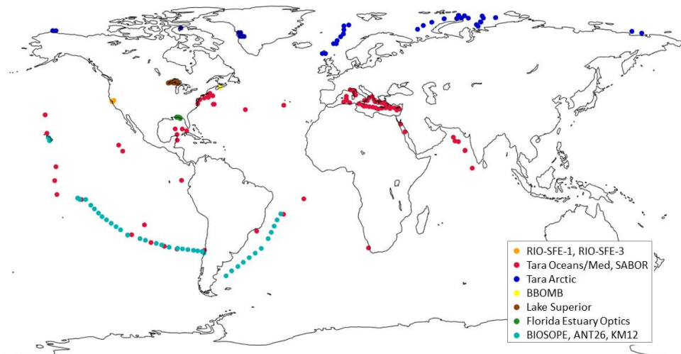
Figure 3: Global geographic distribution of coincident IOP/AOP data.
