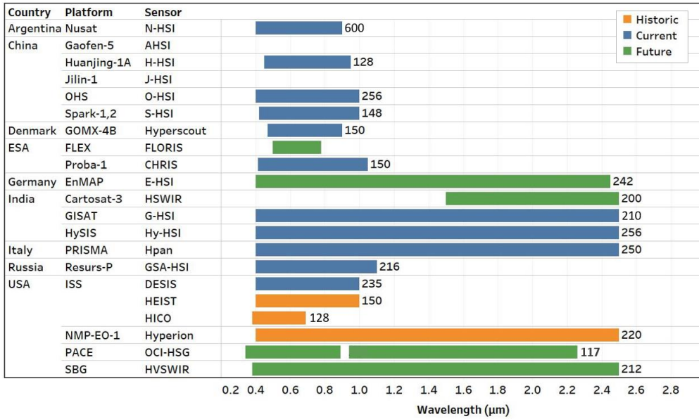
Figure 2: Listing of the spectral wavelength range and total number of sensor bands (right of each bar) where presently known for each of the high spectral resolution satellite missions.
