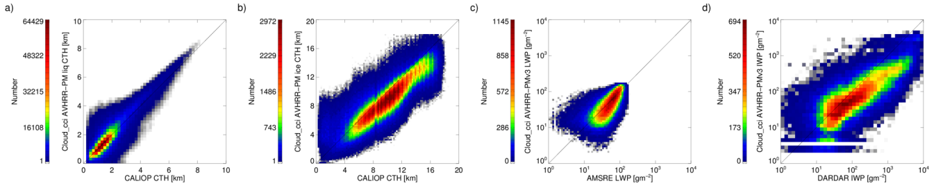
Figure 3. Two-dimensional frequency distributions of AVHRR-PMv3 cloud properties (panel a: cloud top height (CTH) of liquid clouds; panel b: cloud top height of ice clouds; c: liquid water path (LWP); d: ice water path (IWP)) collocated with corresponding reference products of CALIOP, AMSR-E and DARDAR.
