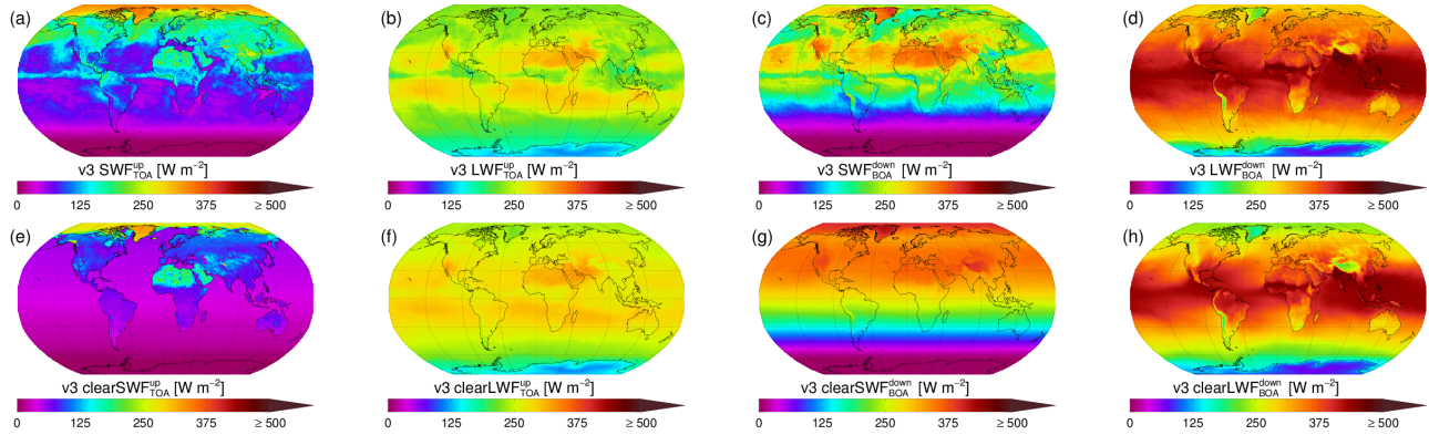
Figure 4. Examples of Level-3C (monthly means) Cloud_cci AVHRR-PMv3 data of SWF_{TOA}^{up} , LWF_{TOA}^{up} , SWF_{BOA}^{down} , LWF_{BOA}^{down} (a-d). clearSWF_{TOA}^{up} , clearLWF_{TOA}^{up} , clearSWF_{BOA}^{down} , clearLWF_{BOA}^{down} are shown in (e-h) representing the same fluxes as in (a-d) but for clear-sky conditions. All data is from June 2014.
