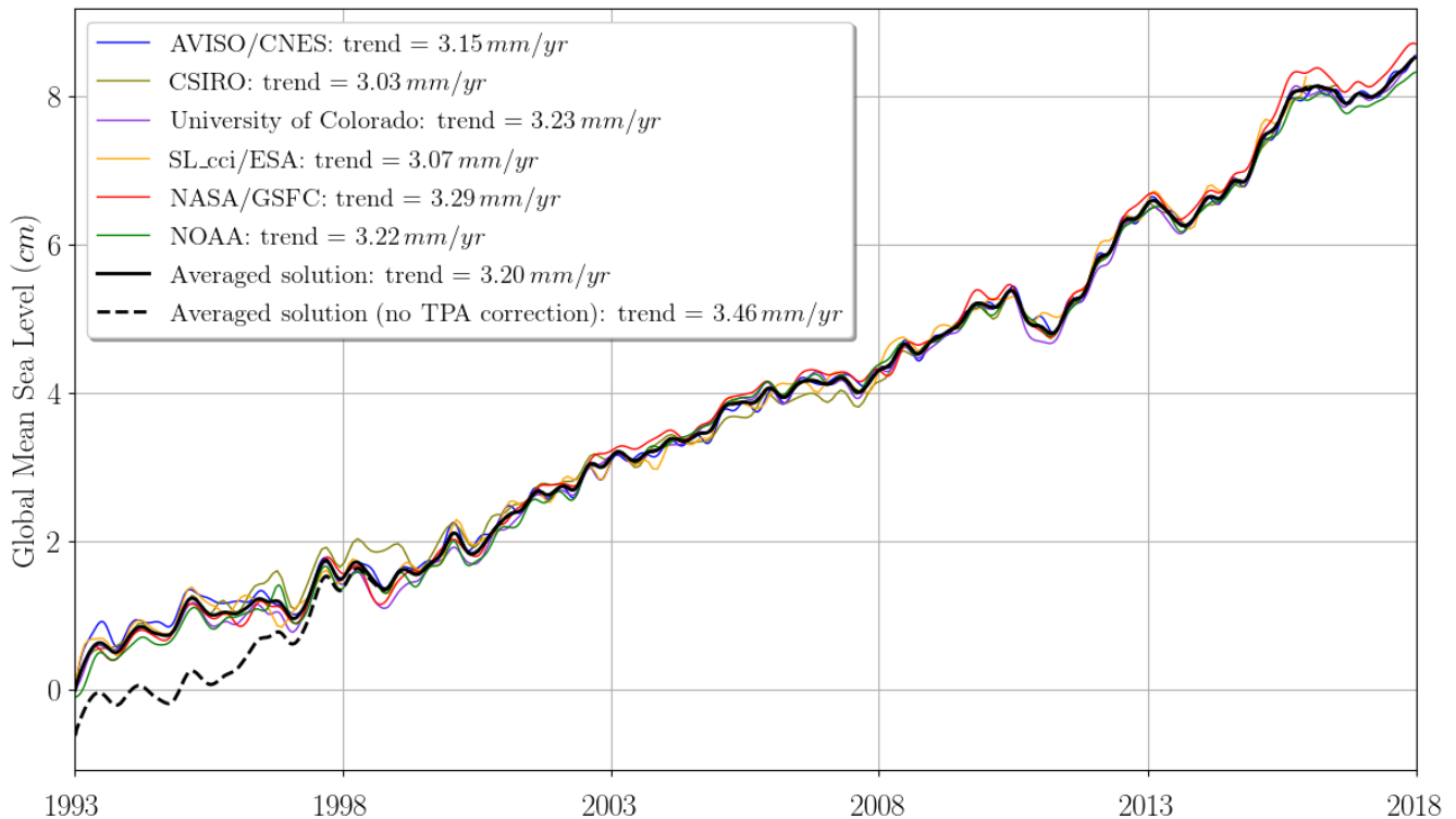
Figure 1: Evolution of GMSL time series (corrected for TOPEX-A drift using Ablain (2017) TOPEX-A correction) from six different groups (AVISO/CNES, CSIRO, University of Colorado, SL_cci/ESA, NASA/GSFC, NOAA) products. The SL_cci/ESA covers a period from January 1993 to December 2016 while all other products cover the full 25-year period (January 1993 to December 2017). Seasonal (annual and semi-annual) signals have been removed and a 6-month smoothing has been applied. An averaged solution has been computed from the six
