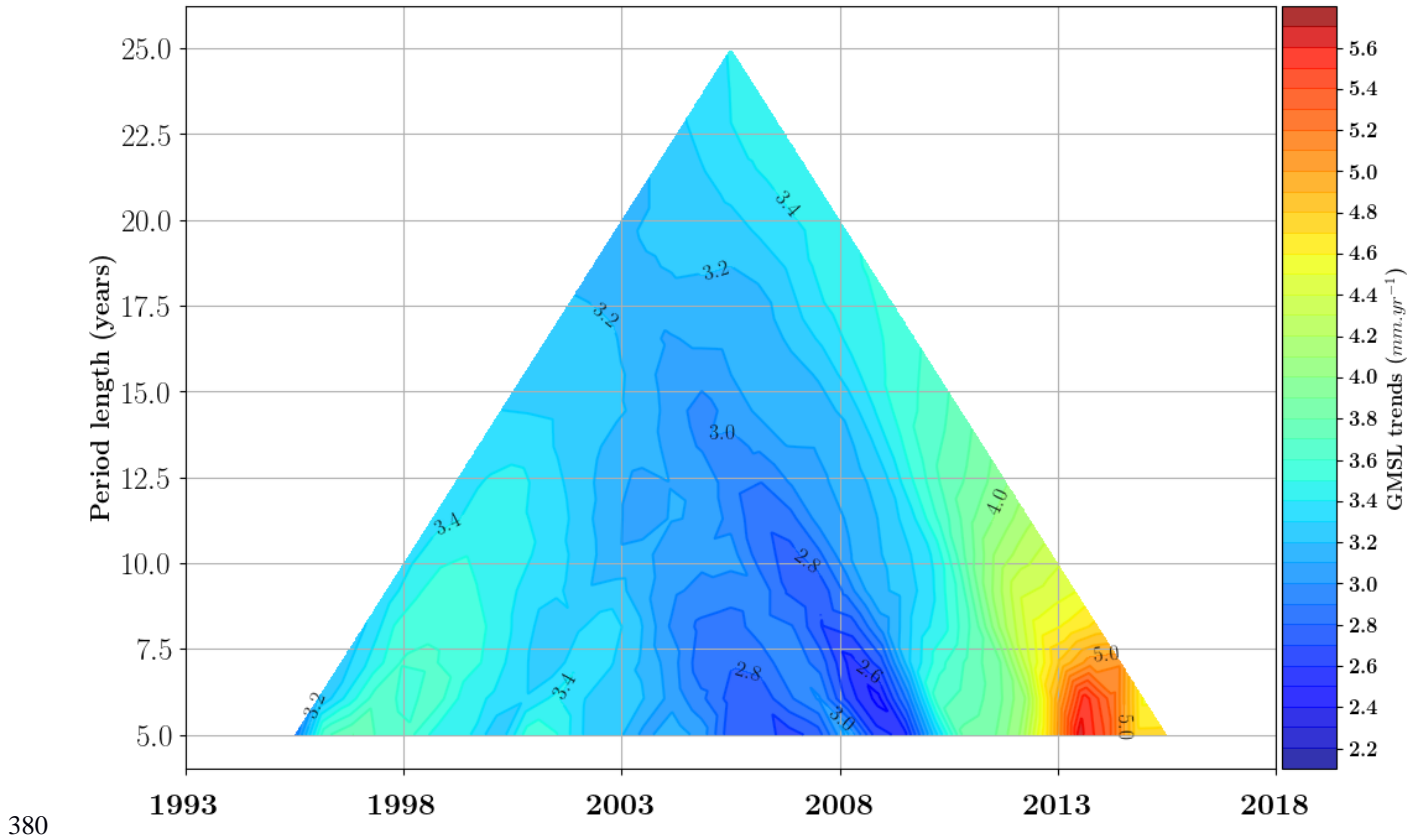
Figure 9. In periods when the acceleration is not significant, the second order polynomial that we used as a predictor to estimate the trend and the acceleration does not hold anymore in principle. For these periods, we should turn out a first order polynomial. The use of a first order polynomial does not affect the trend estimates, but only the trend uncertainty estimates. We checked for differences in trend uncertainty when using either second order or first
