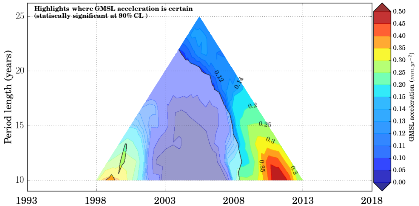
880 Figure 8: GMSL acceleration using the AVISO GMSL time series corrected for the TOPEX-A drift using the correction proposed by Ablain (2017): the acceleration in the shaded areas is not significant (lower than the acceleration uncertainties at the 90% confidence level). The length of the window (in years) is represented on the vertical axis and the central date of the used window (in years) is represented on the horizontal axis.
