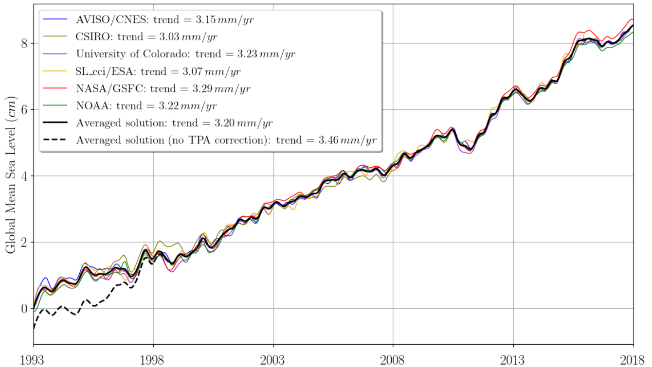
810 Figure 1: Evolution of GMSL time series (corrected for TOPEX-A drift using Ablain (2017) TOPEX-A correction) from six different groups (AVISO/CNES, CSIRO, University of Colorado, SL_cci/ESA, NASA/GSFC, NOAA) products. The SL_cci/ESA covers a period from January 1993 to December 2016 while all other products cover the full 25-year period (January 1993 to December 2017). Seasonal (annual and semi-annual) signals have been removed and a 6-month smoothing has been applied. An averaged solution has been computed from the six groups. GMSL time series have the same average on the 1993-2015 period (common period) and the averaged solution starts at zero in 1993. The averaged solution without TOPEX-A correction has also been represented. A GIA correction of -0.3 mm/yr has been subtracted to each data set. A correction of +0.10 mm/yr due to the deformations of the ocean bottom in response to modern melt of land ice (Frederikse et al., 2017; Lickley et al., 2018) has also been added. 815
