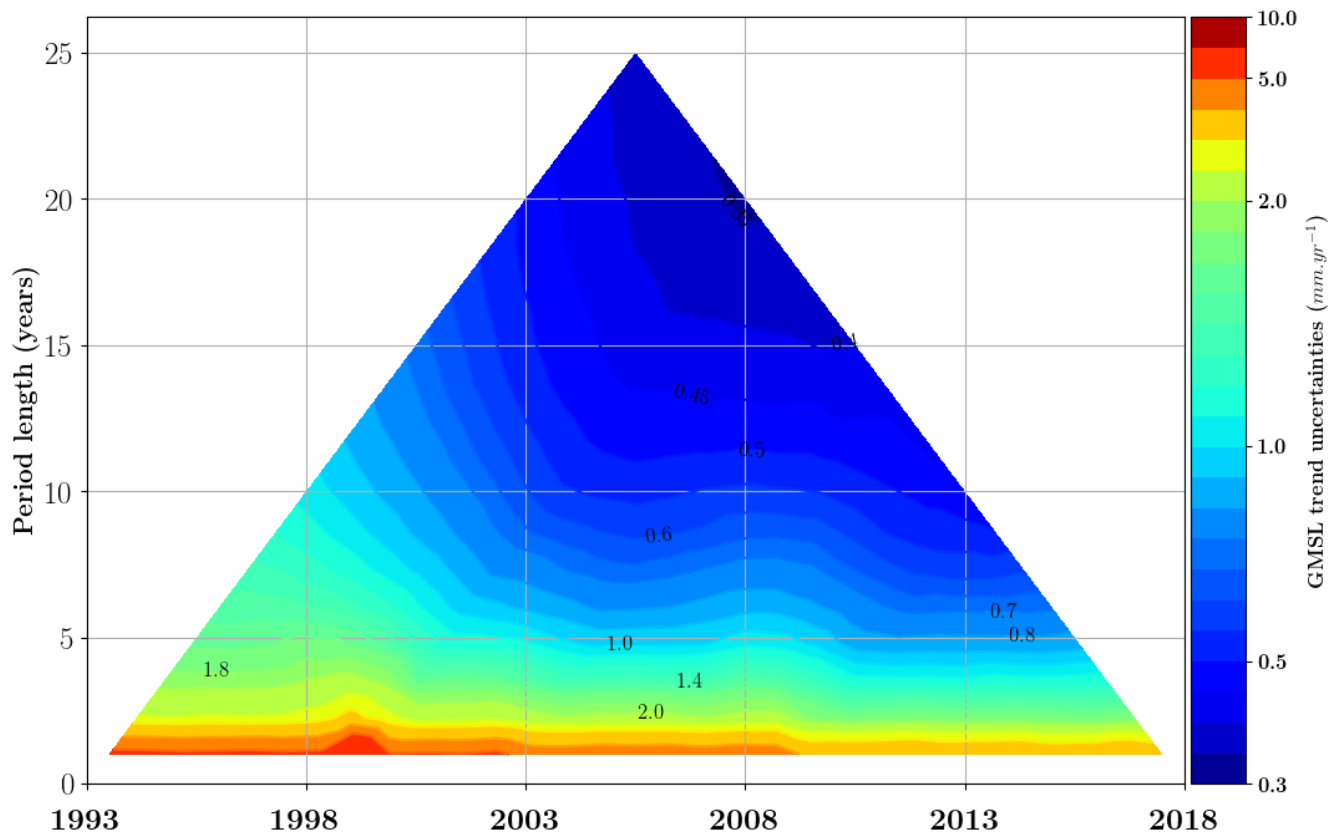
850 Figure 5: GMSL trend uncertainties (mm/yr) estimated for all altimeter periods within the 25-year period (January 1993 to December 2017). The confidence level is 90 % ( 1.65\sigma ). Each colored pixel represents respectively the half-size of the 90% confidence range in the GMSL trend. Values are given in mm/yr. The vertical axis indicates the length of the period (ranging from 1 to 25 years) considered in the computation of the trend, while the horizontal axis indicates the centre date of the period (for example 2000 for the 20-year period 1990-2009).
