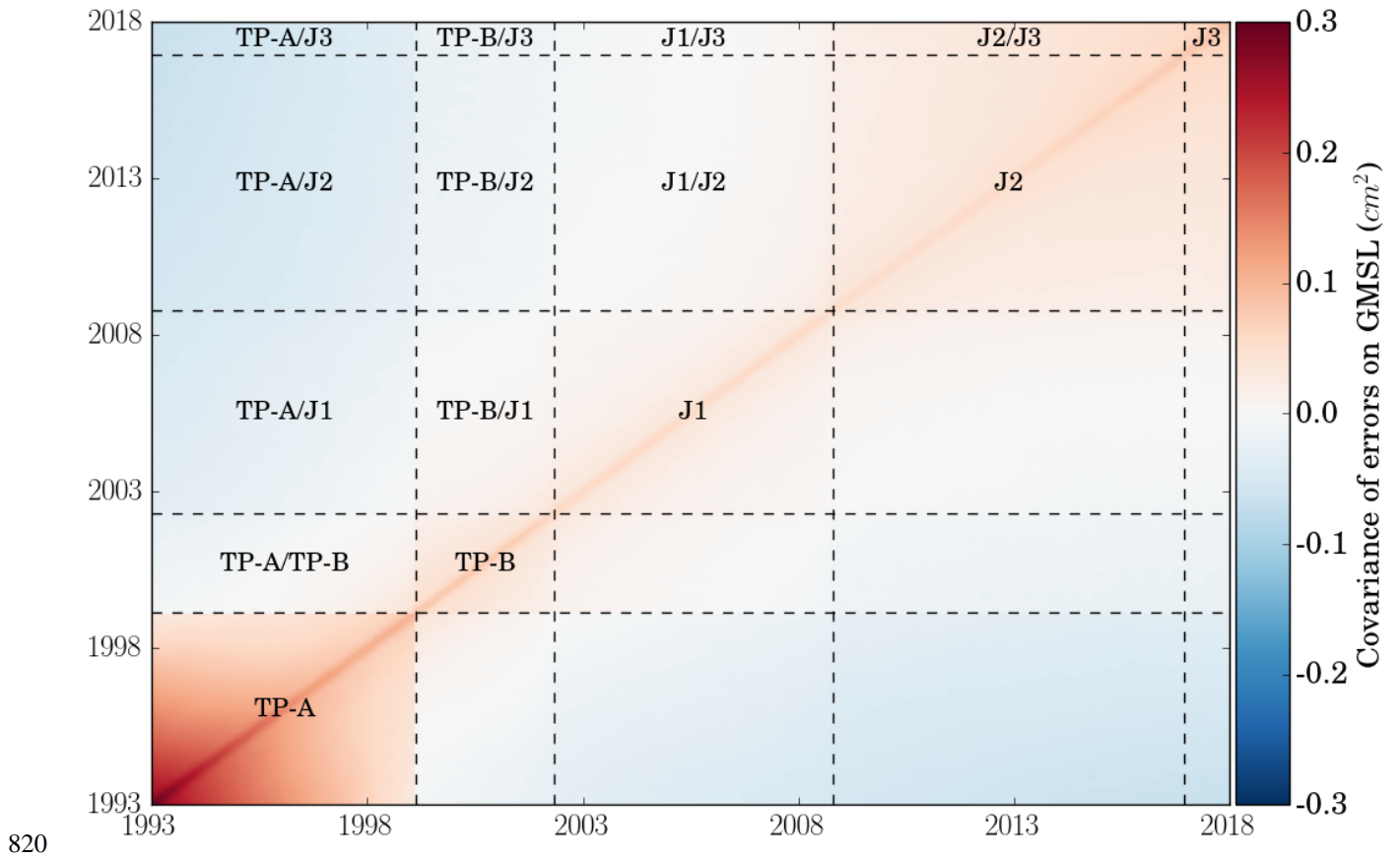
Figure 2: Error variance-covariance matrix of altimeter GMSL on the 25-year period (January 1993 to December 2017).
