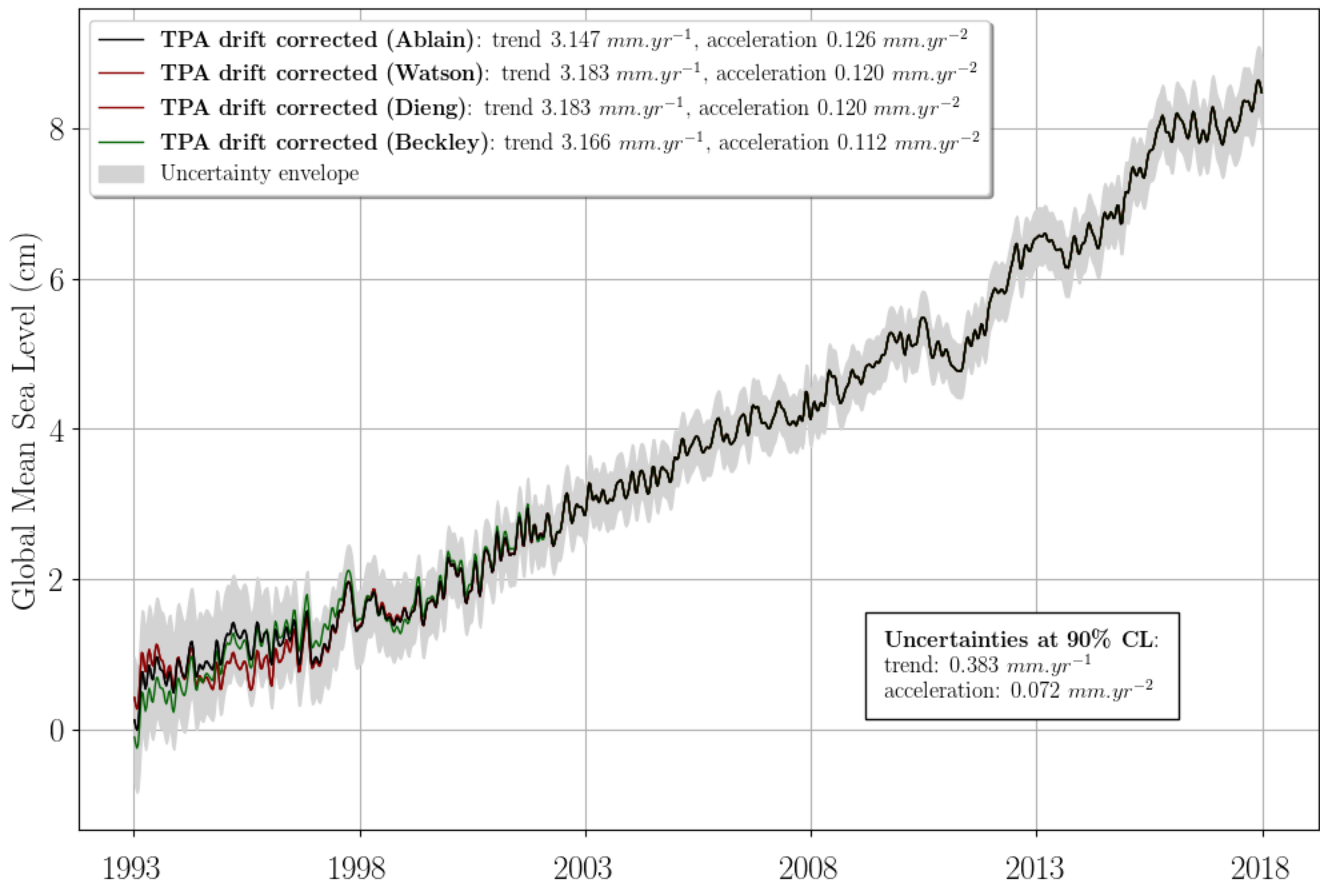
Figure 4: Evolution of the AVISO GMSL with different TOPEX-A corrections. On the black, red and green curves, the TOPEX-A drift correction has been respectively applied based on Ablain (2017), Watson et al. (2015), Dieng et al. (2017) and Beckley et al. (2017). The uncertainty envelope, as well as the trend and acceleration uncertainties are given to a 90% confidence level ( 1.65\sigma ). Seasonal (annual and semi-annual) signals removed and 6-month smoothing applied. A GIA correction of -0.3 \text{ mm/yr} has been subtracted to each data set. A correction of +0.10 \text{ mm/yr} due to the deformations of the ocean bottom in response to modern melt of land ice (Frederikse et al., 2017; Lickley et al., 2018) has also been added.
