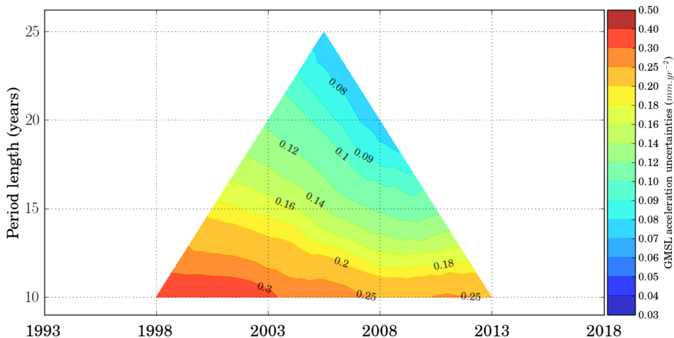
860 Figure 6: GMSL acceleration uncertainties (mm/yr 2 ) estimated for all the altimeter periods within the 25-year period (January 1993 to December 2017). The confidence level is 90 % ( 1.65\sigma ). Each colored pixel represents respectively the half-size of a 90% confidence range in the GMSL acceleration. Values are given in mm/yr 2 . The vertical axis indicates the length of the period (ranging from 1 to 25 years) considered in the computation of the acceleration while the horizontal axis indicates the centre date of the period (for example 2000 for the 20-year 865 period 1990-2009).
