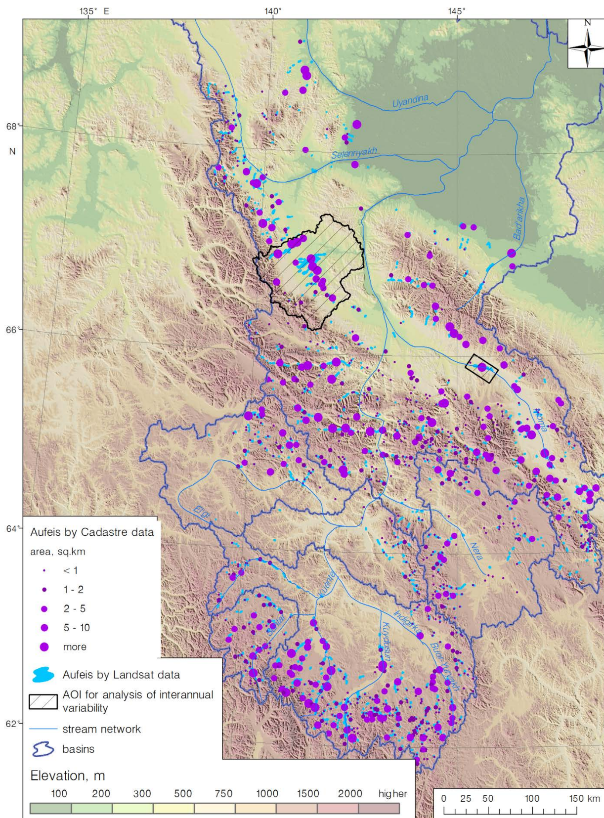
Fig. 8 Augeis in the Indigirka River basin according to the Cadastre and Landsat images. Black outlines with section lining represent the zones where augeis area interannual variability was assessed
