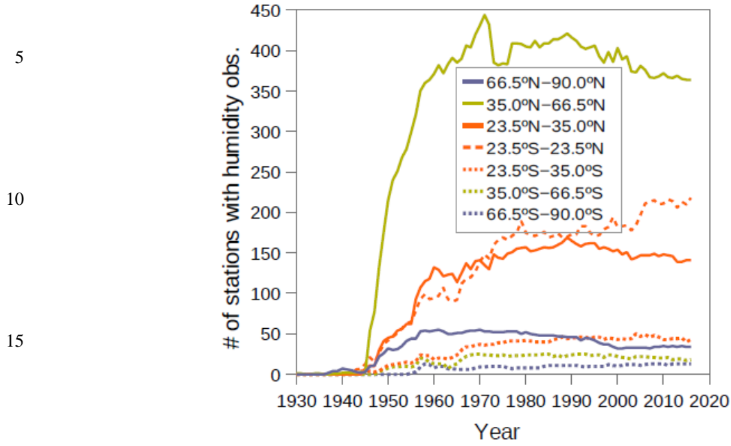
20 Figure 4 Yearly number of fixed stations reporting humidity observations in each climatic zone, since the time of the earliest humidity data in IGRA.
