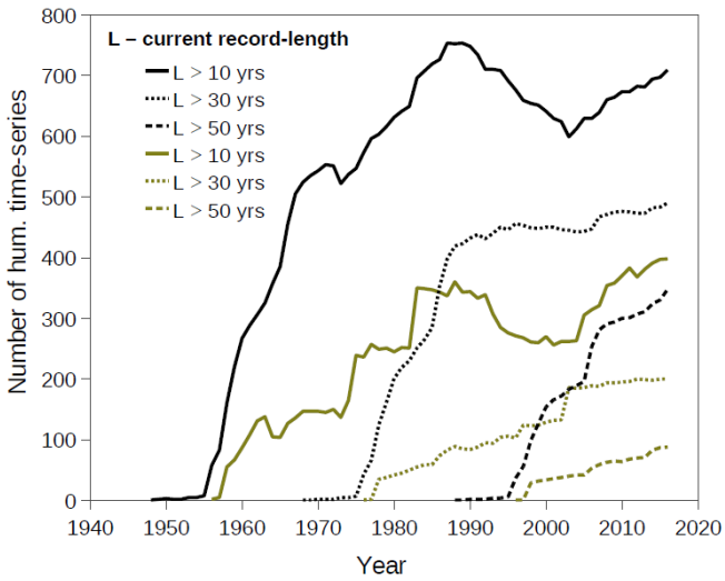
(a) Time-series with any humidity data in the year (no gap years) Idem, but restricted to data in at least 90% of days in year
