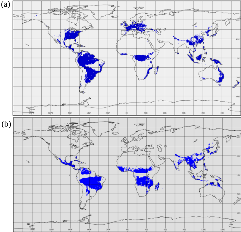
Figure 7. Overlap of global lands with >10 annually summed NDVI and >0.5 SI-TaP (a) and overlap of global lands with >10 annually summed NDVI and monsoon regions (b).
