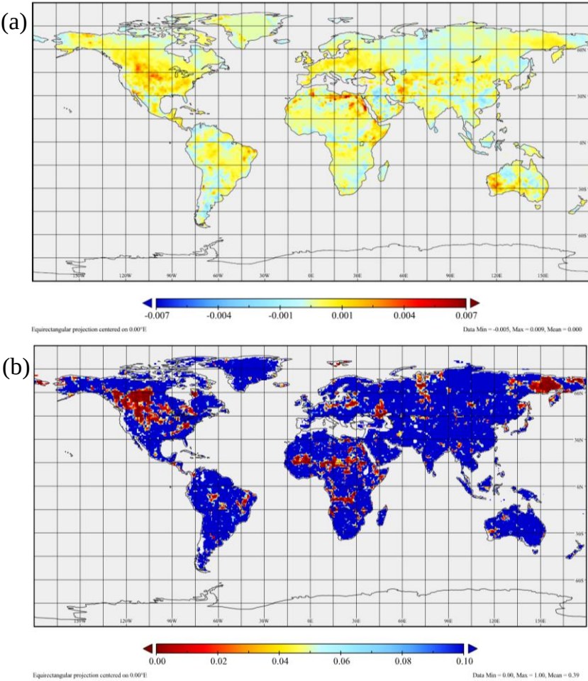
Figure 4. Yearly trend of SI-TaP based on the Mann-Kendall test (a) and p -values from the Mann-Kendall test on SI-TaP (b).
