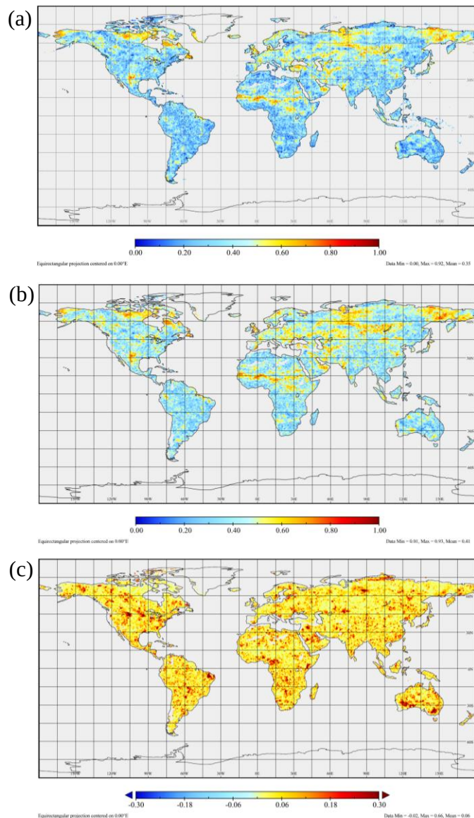
Figure 5. Coefficient of determination ( R^2 ) for linear regression of annually summed NDVI against annual > 0°C accumulated temperature and annual precipitation (a), R^2 for linear regression of annually summed NDVI against annual > 0°C accumulated temperature, annual precipitation, and SI-TaP (b), and change in R^2 after involving SI-TaP (c).
