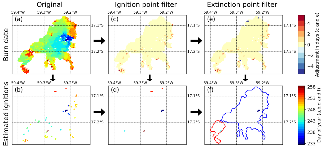
Figure 2: Algorithm example accounting for uncertainty in the “day of burn” and identifying individual fires within large clusters of adjacent burned pixels. (a) The original MCD64A1 collection 6 day of burn for one burned patch in the Brazilian Cerrado (in the year 2015), and (b) local minima or “ignition points” identified within the original day of burn data layer. (c) Burn date adjustment based on the filter that removes local minima that do not progress continuously through time and space (positive adjustment), and (d) the corresponding estimate of ignition points based on the adjusted day of burn field. (e) Further burn date adjustment based on the removal of outliers along the edge of the fire (negative adjustment of extinction points), and (f) the final estimate of ignition locations and date by the Global Fire Atlas based on the combined adjustments shown in (e). In (f), the red and blue lines indicate the final fire perimeters.
