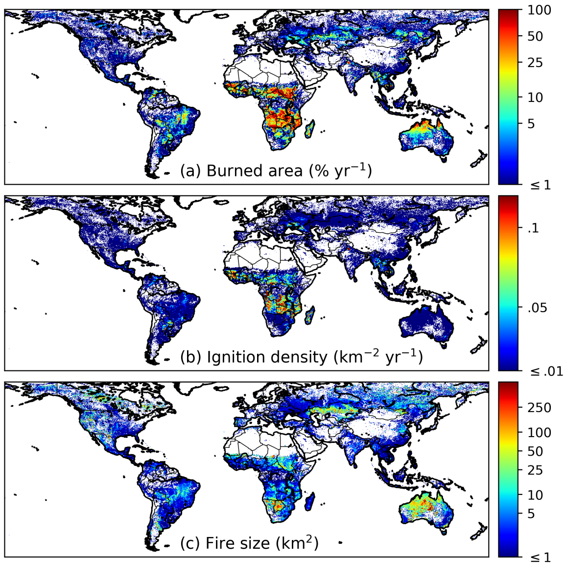
Figure 8: Average global burned area (MCD64A1), ignition density, and fire size over the study period 2003 – 2016. For any given location, burned area in panel (a) can be represented as the product of ignitions per year shown in (b) and fire size shown in (c).
