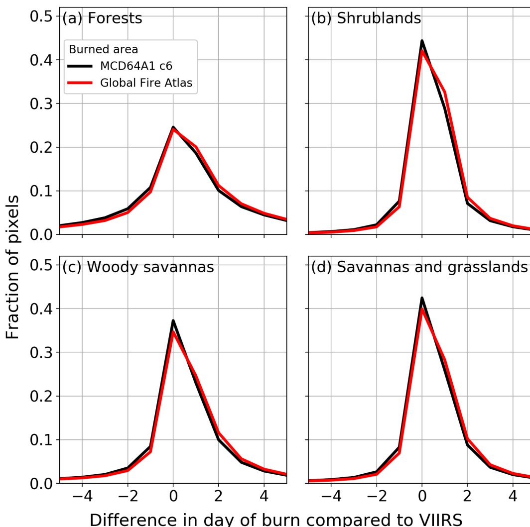
340 Figure 4: Global comparison of burn dates derived from the MCD64A1 burned area product, adjusted burn dates of the Global Fire Atlas, and VIIRS active fire detections (2012 – 2016). (a) Forests, (b) shrublands, (c) woody savannas, and (d) savannas and grasslands. Negative values indicate pixels with a burned area day of burn earlier than the corresponding VIIRS active fire detection, zero indicates no difference in day of burn between both datasets, and positive numbers indicate a delayed detection of burned area compared to active fire detections.
