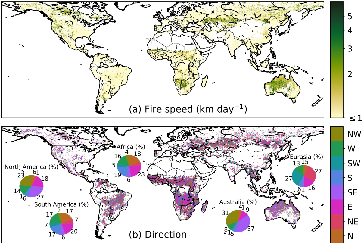
Figure 10: Average fire speed (a) and the dominant direction of fire spread (b) over the study period 2003 – 2016. For each 0.25° grid cell the direction was estimated as the dominant fire spread direction of fires larger than 10 km 2 within the grid cell. We focused on larger fires ( \geq 10 km 2 ) to determine the dominant spread direction, because large fires will generally express a clearer spatiotemporal structure of fire spread at 500 m daily resolution. Pie charts show the fraction of individual larger fires ( \geq 10 km 2 ) by dominant spread direction for each continent.
