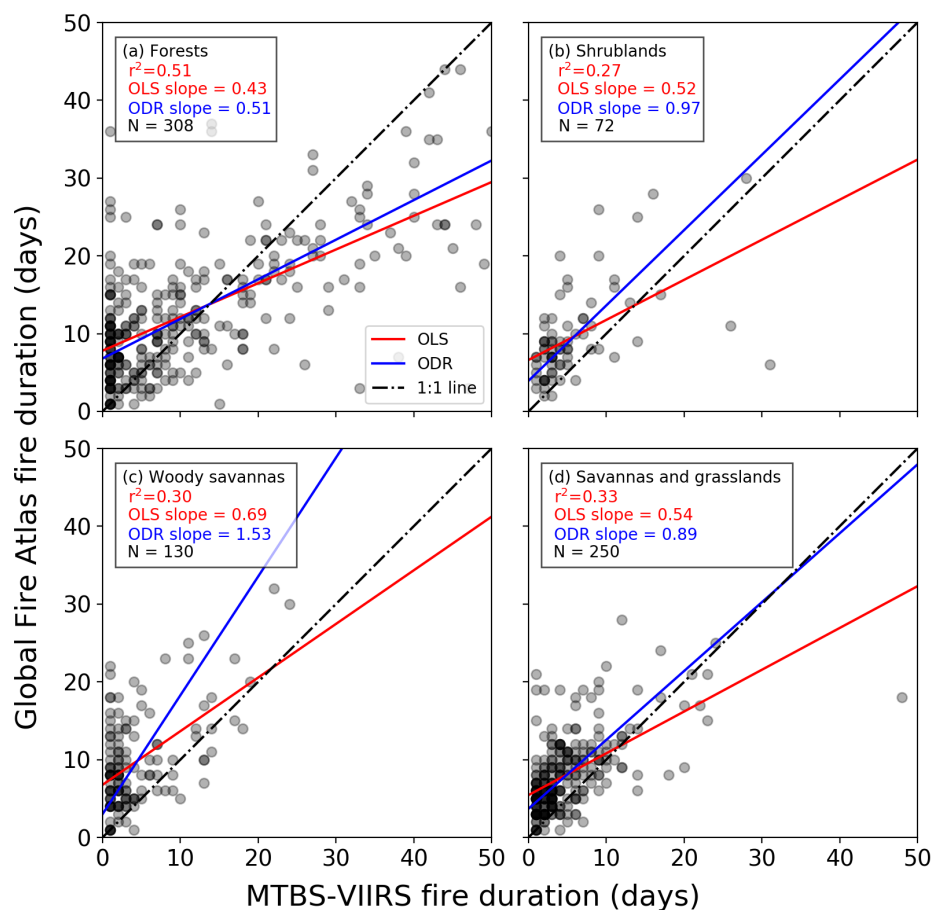
Figure 6: Comparison of fire duration estimates from the Global Fire Atlas and the combination of VIIRS active fire detections within MTBS fire perimeters for the continental US (2012 – 2015). (a) Forests, (b) shrublands, (c) woody savannas, and (d) savannas and grasslands. Red lines indicate the slope
