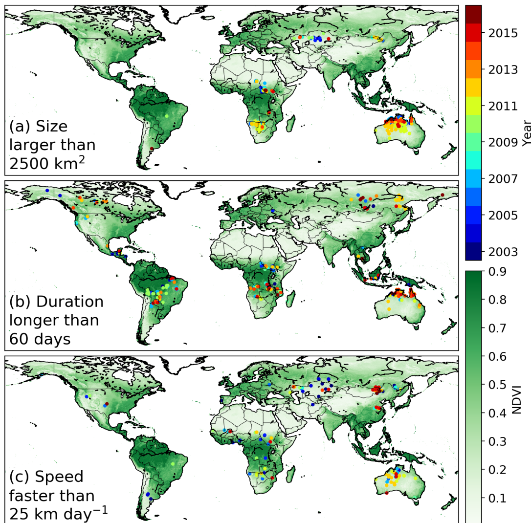
Figure 11: Location and year of the largest, longest, and fastest fires over the study period 2003 – 2016. (a) fires larger than 2500 km 2 , (b) fires longer than 60 days, and (c) fires with an average velocity higher than 25 km day -1 . The background image depicts mean MODIS normalized difference vegetation index (NDVI, 2003 – 2016), an indicator for large scale vegetation patterns and available fuels.
