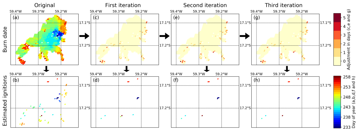
Figure A1: Burn date adjustment to remove local minima that are not associated with ignition points. (a) MCD64A1 burn date estimate for the 2015 example fires in the Brazilian Cerrado ecosystem, (b) local minima within (a). (c) Burn date adjustment after the first iteration, and (d) resulting local minima. (e) Burn date adjustment after the second iteration, and (f) resulting local minima. (g) Burn date adjustment after the third iteration, and (h) resulting local minima. Note that for these particular fires there was no difference between (e and f) and (g and h), and the final iteration has no added value here. We found that multiple iterations were particularly beneficial for slow moving fires in forested ecosystems.
