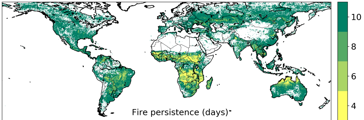
Figure A3: Average fire persistence threshold at 0.25° resolution. The fire persistence threshold determines how long a fire may take to spread from one 500 m grid cell into the next. We used a 4-day fire persistence threshold for 500 m grid cells that burned more than 3 times during the study period (2003 - 2016), and a 6, 8 and 10-day fire persistence period for grid cells that burned 3 times, 2 times, or 1 time, respectively.
