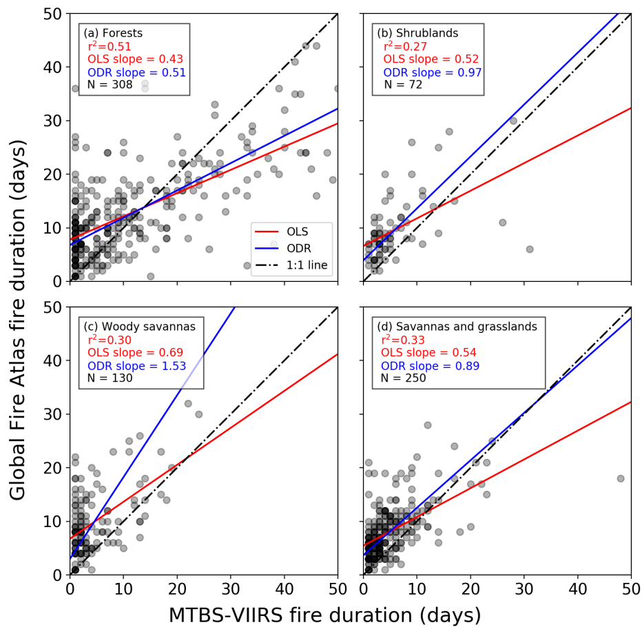
395 Figure 6: Comparison of fire duration estimates from the Global Fire Atlas and the combination of VIIRS active fire detections within MTBS fire perimeters for the continental US (2012 – 2015). (a) Forests, (b) shrublands, (c) woody savannas, and (d) savannas and grasslands. Red lines indicate the slope
