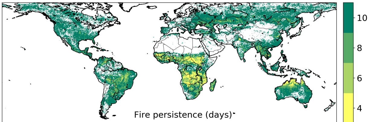
725 Figure A3: Average fire persistence threshold at 0.25° resolution. The fire persistence threshold determines how long a fire may take to spread from one 500 m grid cell into the next. We used a 4-day fire persistence threshold for 500 m grid cells that burned more than 3 times during the study period (2003 - 2016), and a 6, 8 and 10-day fire persistence period for grid cells that burned 3 times, 2 times, or 1 time, respectively.
