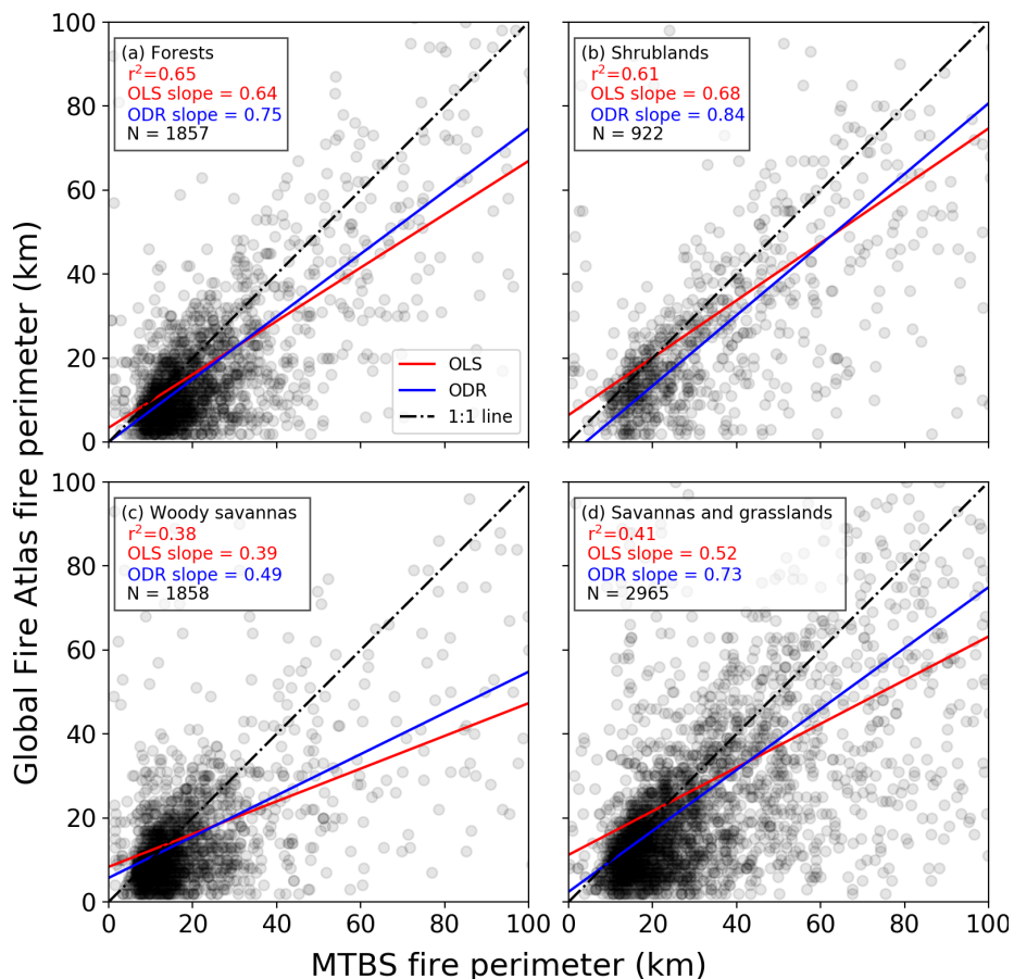
370 Figure 5: Comparison of fire perimeter estimates based on the Global Fire Atlas and MTBS for the continental US (2003 – 2015). (a) Forests, (b) shrublands, (c) woody savannas, and (d) savannas and grasslands. Red lines indicate the slope between both datasets based on ordinary least squares (OLS) with corresponding r^2 values, while blue lines are based on orthogonal distance regression (ODR). For the scatter plots, darker gray or black indicates a greater density of points.
