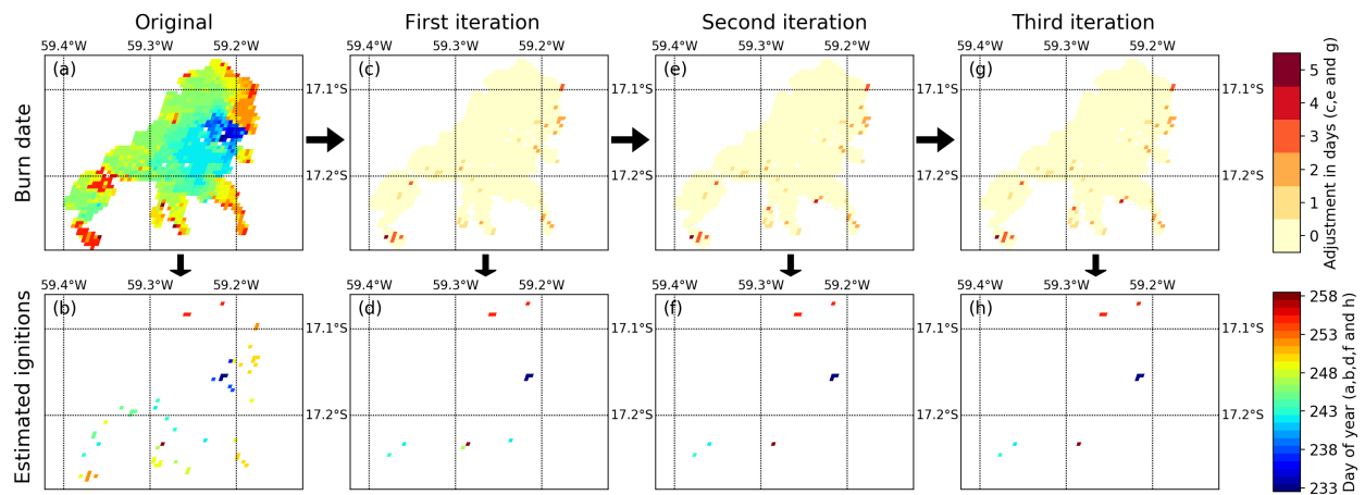
710 Figure A1: Burn date adjustment to remove local minima that are not associated with ignition points. (a) MCD64A1 burn date estimate for the 2015 example fires in the Brazilian Cerrado ecosystem, (b) local minima within (a). (c) Burn date adjustment after the first iteration, and (d) resulting local minima. (e) Burn date adjustment after the second iteration, and (f) resulting local minima. (g) Burn date adjustment after the third iteration, and (h) resulting local minima. Note that for these particular fires there was no difference between (e and f) and (g and h), and the final iteration has no added value here. We found that multiple iterations were particularly beneficial for slow moving fires in forested ecosystems.
