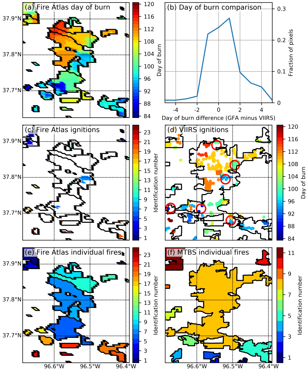
745 Figure B2: Comparison of Global Fire Atlas perimeters and ignition locations to estimates based on 750 MTBS and VIIRS for frequently-burning grasslands in Kansas, USA. (a) Global Fire Atlas adjusted 755 burn dates from MCD64A1, (b) per-pixel comparison of adjusted burn dates used within the Global Fire Atlas (GFA) to the day of the active fire detection from VIIRS, (c) ignition points as estimated by the Global Fire Atlas, (d) manually interpreted ignition locations (red circles) based on VIIRS active fire detections on top of MTBS fire perimeters, (e) individual fires as estimated by the Global Fire Atlas, and (f) the MTBS burned area and individual fires. Here, MCD64A1 data underestimated the total burned area compared to the visual interpretation of Landsat data within the MTBS project, resulting in fragmentation of individual large fires. However, the daily temporal resolution of MODIS imagery allowed the Global Fire Atlas to distinguish individual fires and ignition points within larger burn scars that cannot be resolved from infrequent Landsat observations used to delineate fire perimeters within the MTBS project. Broad patterns of ignition locations identified by the Global Fire Atlas were confirmed by manual interpretation of patterns inferred from VIIRS active fire detections (d).
