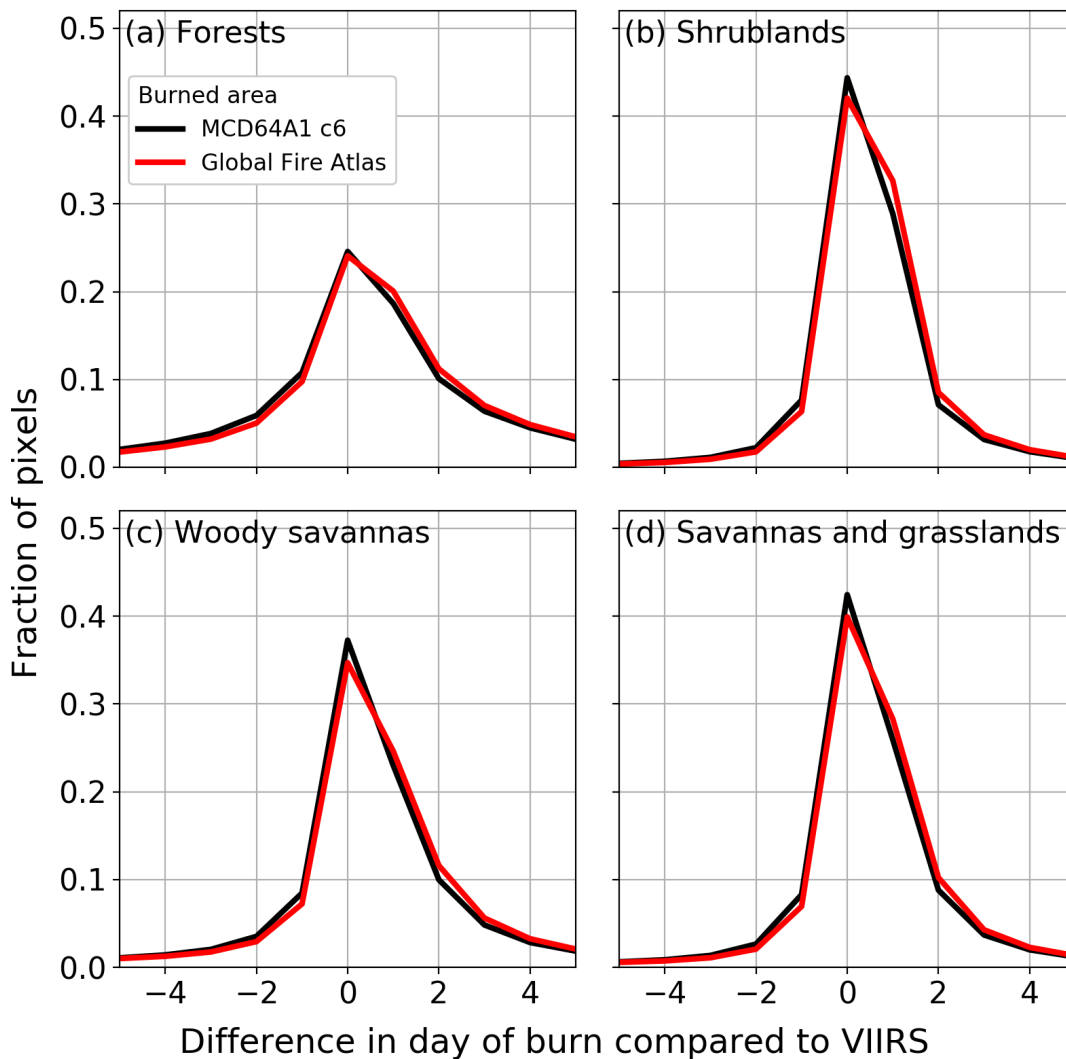
340 Figure 4: Global comparison of burn dates derived from the MCD64A1 burned area product, 345 adjusted burn dates of the Global Fire Atlas, and VIIRS active fire detections (2012 – 2016). (a) Forests, (b) shrublands, (c) woody savannas, and (d) savannas and grasslands. Negative values indicate pixels with a burned area day of burn earlier than the corresponding VIIRS active fire detection, zero indicates no difference in day of burn between both datasets, and positive numbers indicate a delayed detection of burned area compared to active fire detections.
