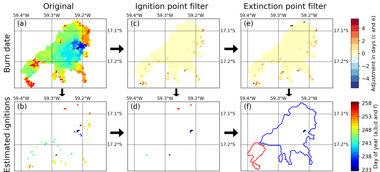
220 Figure 2: Algorithm example accounting for uncertainty in the “day of burn” and identifying individual fires within large clusters of adjacent burned pixels. (a) The original MCD64A1 collection 6 day of burn for one burned patch in the Brazilian Cerrado (in the year 2015), and (b) local minima or “ignition points” identified within the original day of burn data layer. (c) Burn date adjustment based on 225 the filter that removes local minima that do not progress continuously through time and space (positive adjustment), and (d) the corresponding estimate of ignition points based on the adjusted day of burn field. (e) Further burn date adjustment based on the removal of outliers along the edge of the fire (negative adjustment of extinction points), and (f) the final estimate of ignition locations and date by the Global Fire Atlas based on the combined adjustments shown in (e). In (f), the red and blue lines indicate the final fire 230 perimeters.
