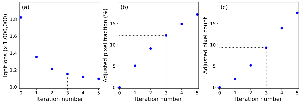
715 Figure A2: Tradeoffs between reducing local minima not associated with ignition locations and adjustments made to the global burned area product. (a) Local minima (ignitions) detected within the daily 500 m global burned area data for 2015 after different number of iterations of the ignition point filter, (b) corresponding fraction of burned area pixels with adjusted burn date, and (c) corresponding number of burned area pixels adjusted divided by the reduction in ignition count. In this study, we used three iterations 720 of the ignition point filter (indicated with the intermittent lines in figures a, b and c), and “0 iterations” refers to the original MCD64A1 col. 6 burned area data.
