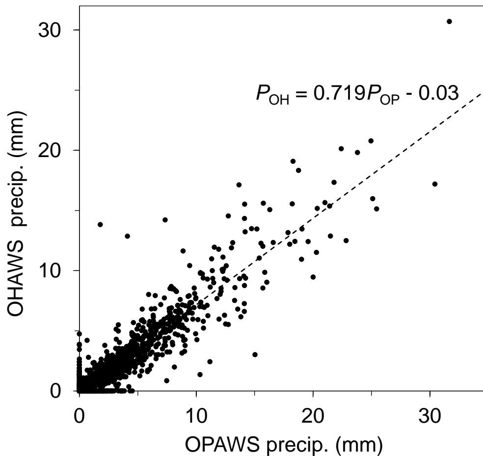
Figure 3. Relationship between daily winter precipitation at OHAWS ( P_{OH} ) and OPAWS ( P_{OP} ). Plotted data have been 260 corrected for instrument noise and wind-induced undercatch.
