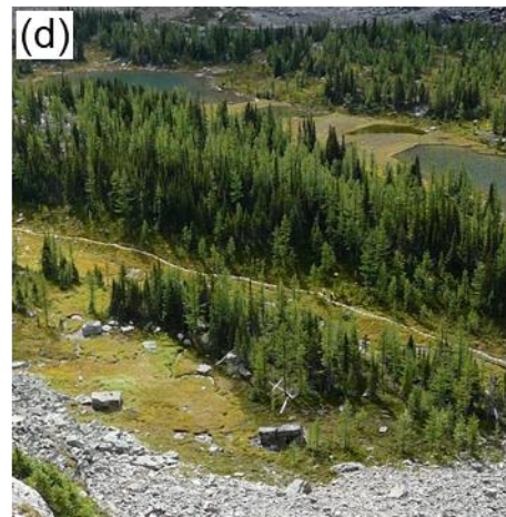
Figure 2. Major hydrogeological response units in the Lake O'Hara watershed. (a) Exposed bedrock. (b) Proglacial moraine. (c) Talus. (d) Alpine meadow.
