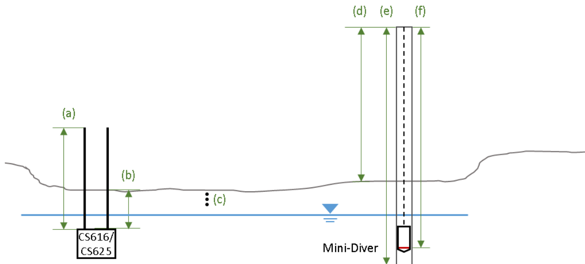
720 Figure D1. Scheme of setup of water level measurement in the polygon center: (a) length of the parallel measurement rods (30 cm) of the Campbell Scientific CS616/CS625 sensors, (b) distance from the sensor base to the ground surface (CS625: -15 cm; CS616 -11.5 cm), (c) Campbell Scientific T109 probes at depths of -1 cm, -3 cm, -6 cm below surface, (d) height of the well above the ground surface (45.5 cm), (e) length of the well (70 cm), (f) distance from 725 the top of the well to the water pressure measurement level of the Schlumberger Mini-Diver. The difference between the ground level at CS616 and Mini-Diver locations is 3 cm. Blue line illustrates water level, gray line the ground surface.
