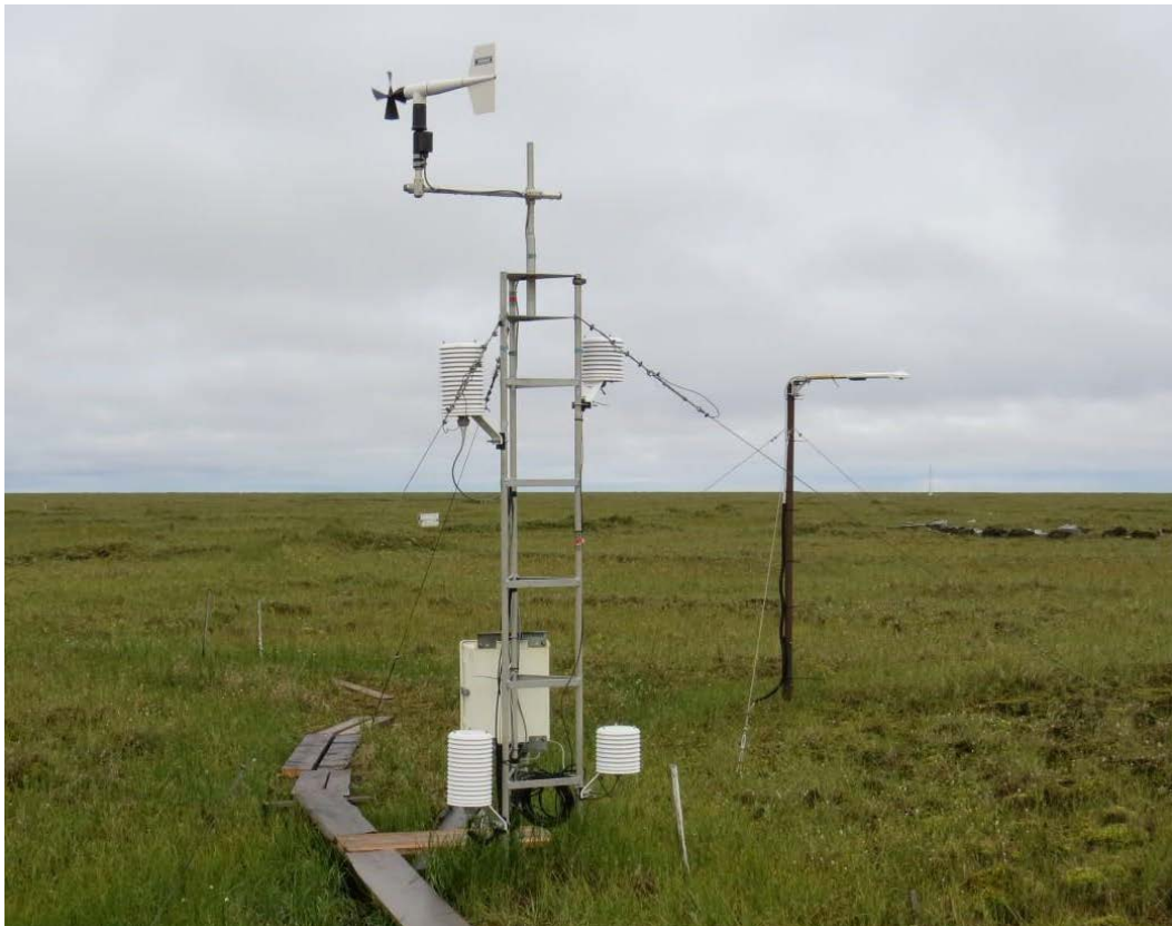
Figure B1. Samoylov meteorological station setup, August 2002–present (72.37001° N, 126.48106° E). Photo taken in August 2015. The two long radiation shields (left side of tower) at heights of 0.5 m and 2 m house the combined temperature and relative humidity probes (two Vaisala HMP155A sensors were installed on 17 September 2017) and the two shorter shields (right side of tower) at the same heights contain Campbell Scientific PT100 sensors (installed on 22 August 2013) to measure air temperature only. The data logger (Campbell Scientific CR1000, installed on 30 June 2009), multiplexer (Campbell Scientific AM16/32A, installed on 27 July 2010) and barometric pressure sensor (Vaisala PTP110, installed on 22 August 2014) are located in the white box at the back of the tower. The wind monitor and radiation sensor are shown in the figures below (Figures B2 and B3).
