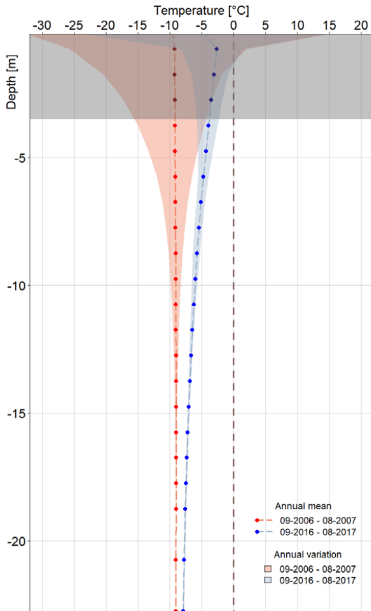
560 Figure 3. Mean annual, maximum and minimum permafrost temperatures at different depths between 2006 and 2017, as recorded in the Samoylov Island borehole. Mean annual temperatures are based on the period 1 September 2006 to 31 August 2007, and 1 September 2016 to 31 August 2017. Maximum and minimum annual variations are based on the same time period and computed from mean daily temperatures. The upper 3.5 m below surface are shaded 565 in grey since we recommend not to these data for active layer thermal processes.
